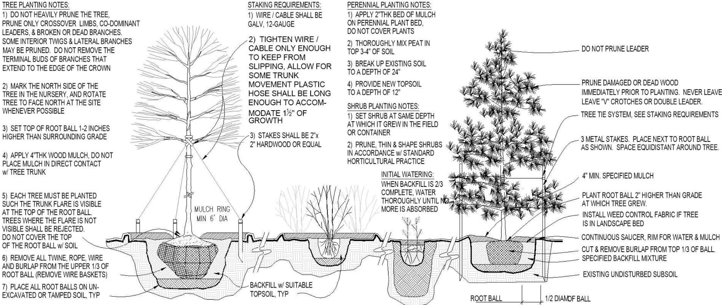
2 PLANTING INSTALLATION DETAILS SCALE: NTS
