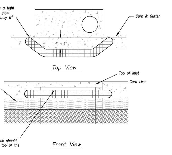
Sump Inlet Sediment Filter
