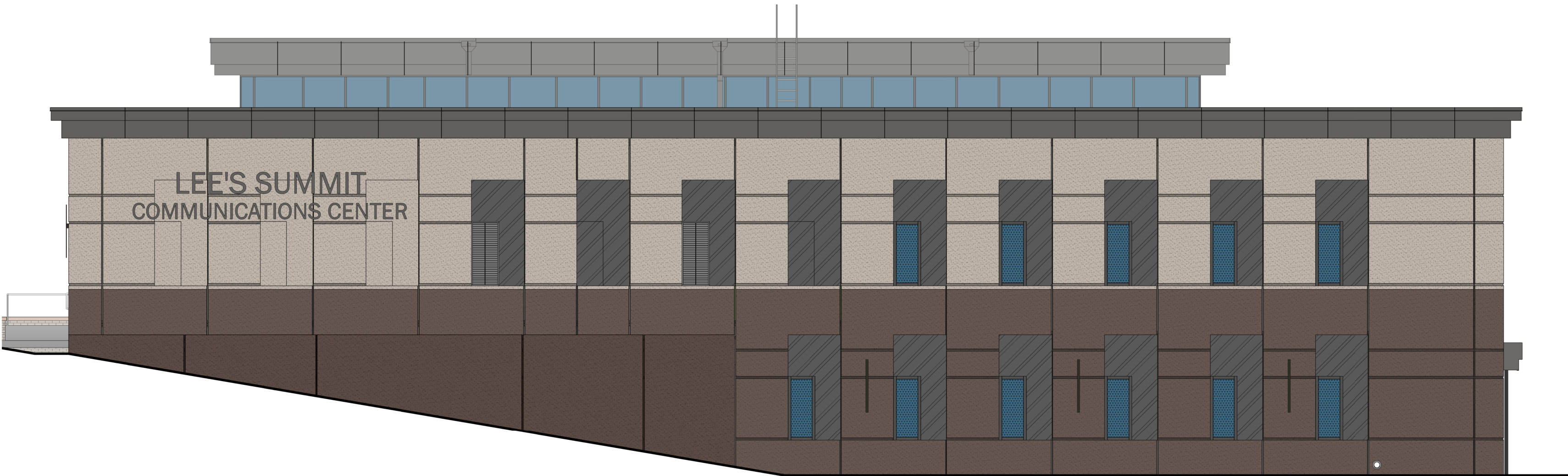
SOUTH ELEVATION 1/8" = 1'-0"
