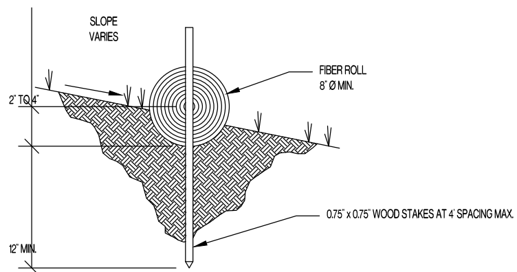
ENTRENCHMENT DETAIL
