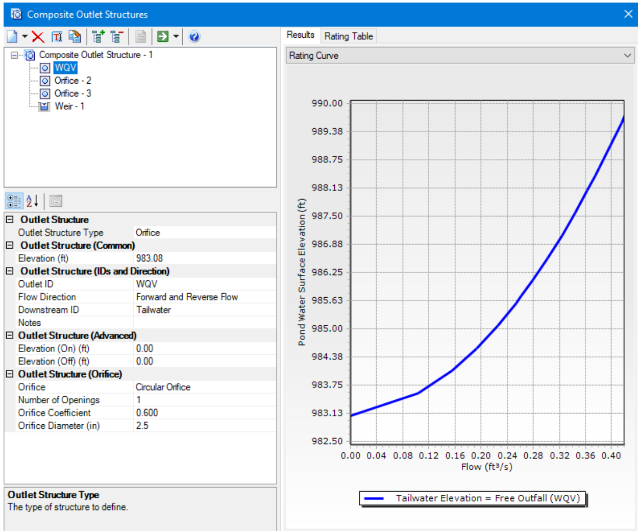
Water Quality Volume Orifice - Rating Curve and Design Parameters
