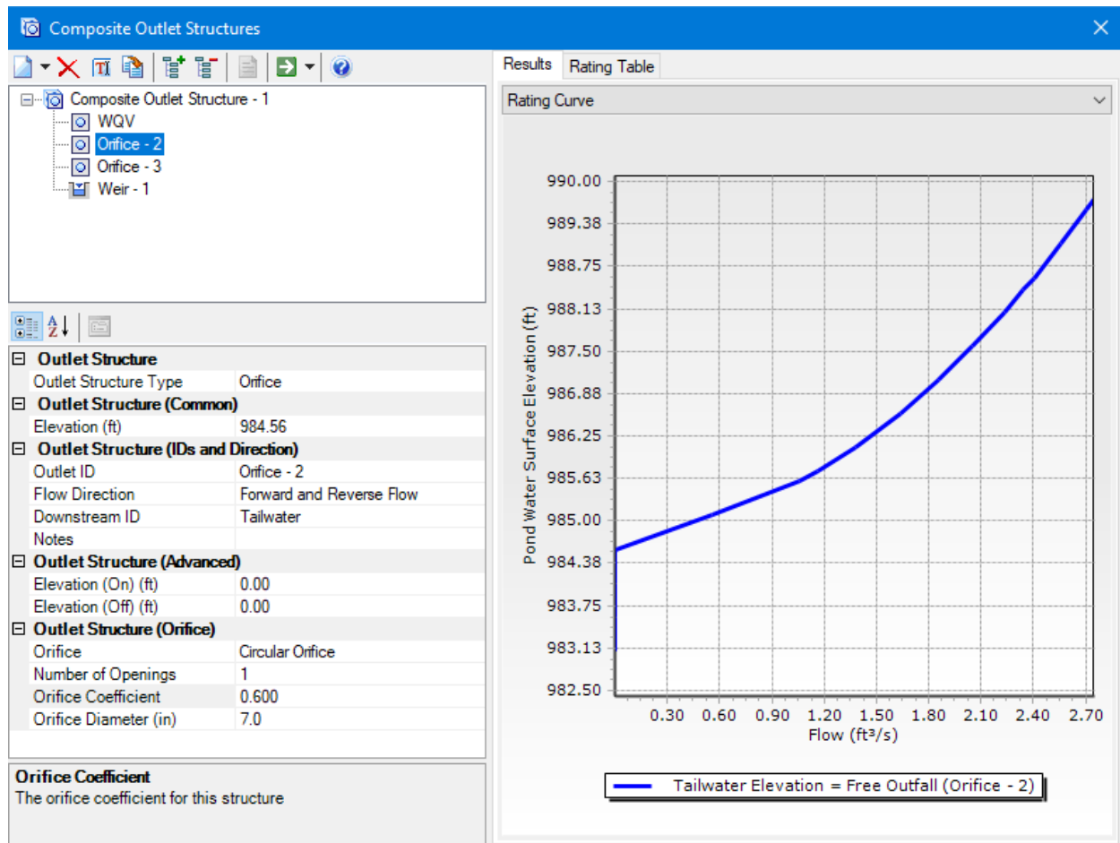
Orifice 2 - Rating Curve and Design Parameters
