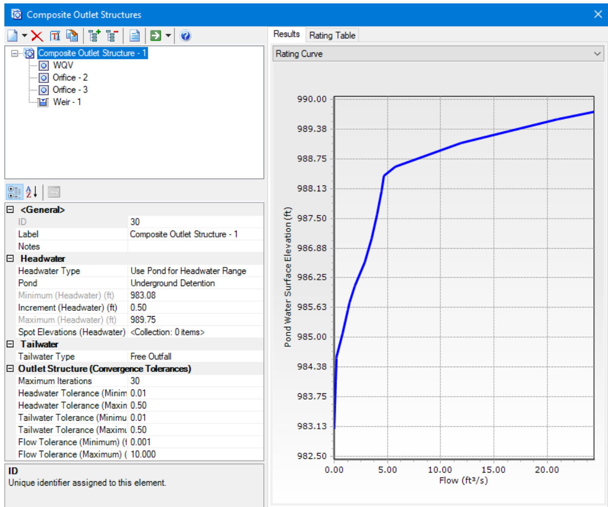
Composite Outlet Structure - Rating Curve and Design Parameters
