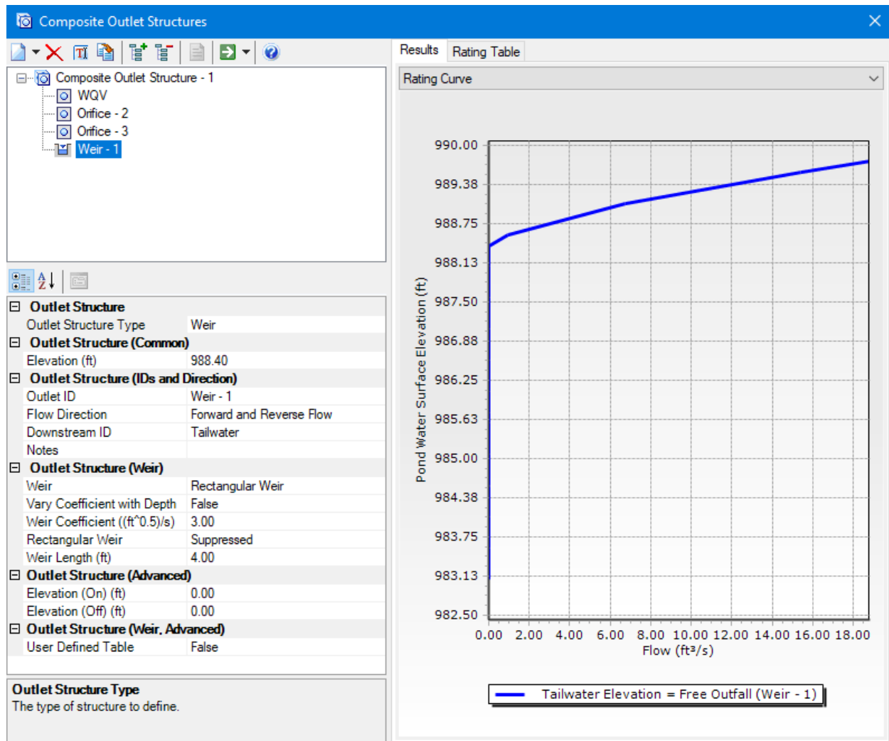
Weir - Rating Curve and Design Parameters
