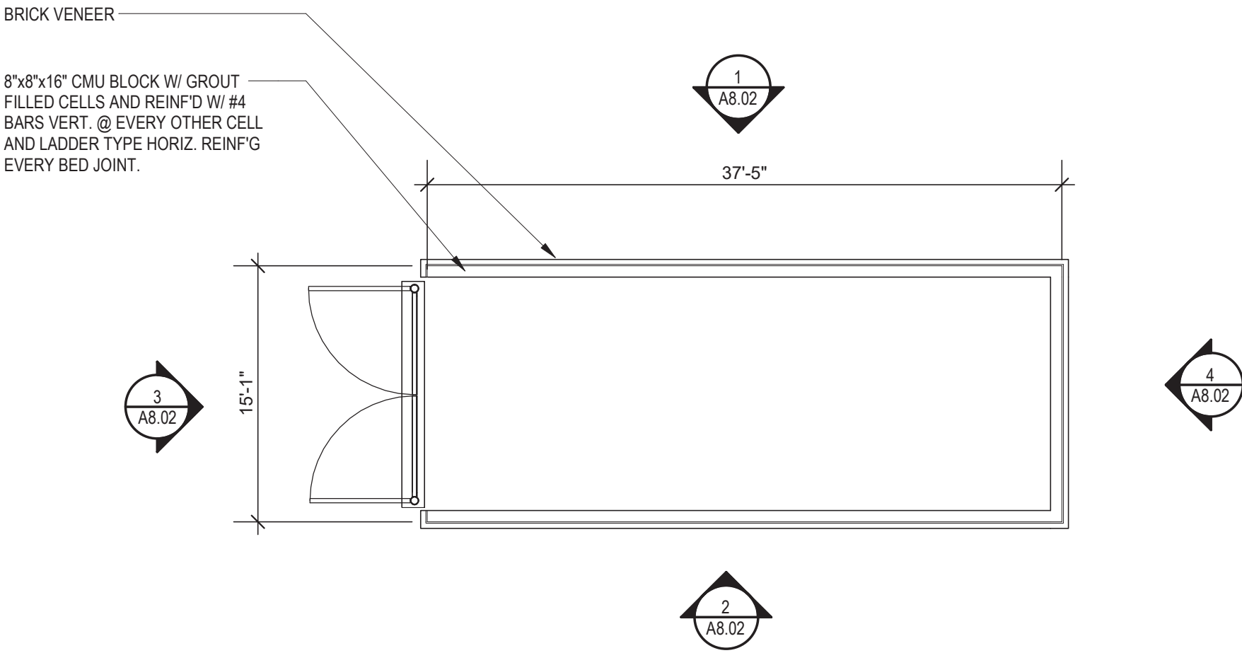
6 1ST FLOOR BUILDING PLAN 1/8" = 1'-0"
