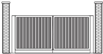
3 TRASH FRONT 1/8" = 1'-0"
