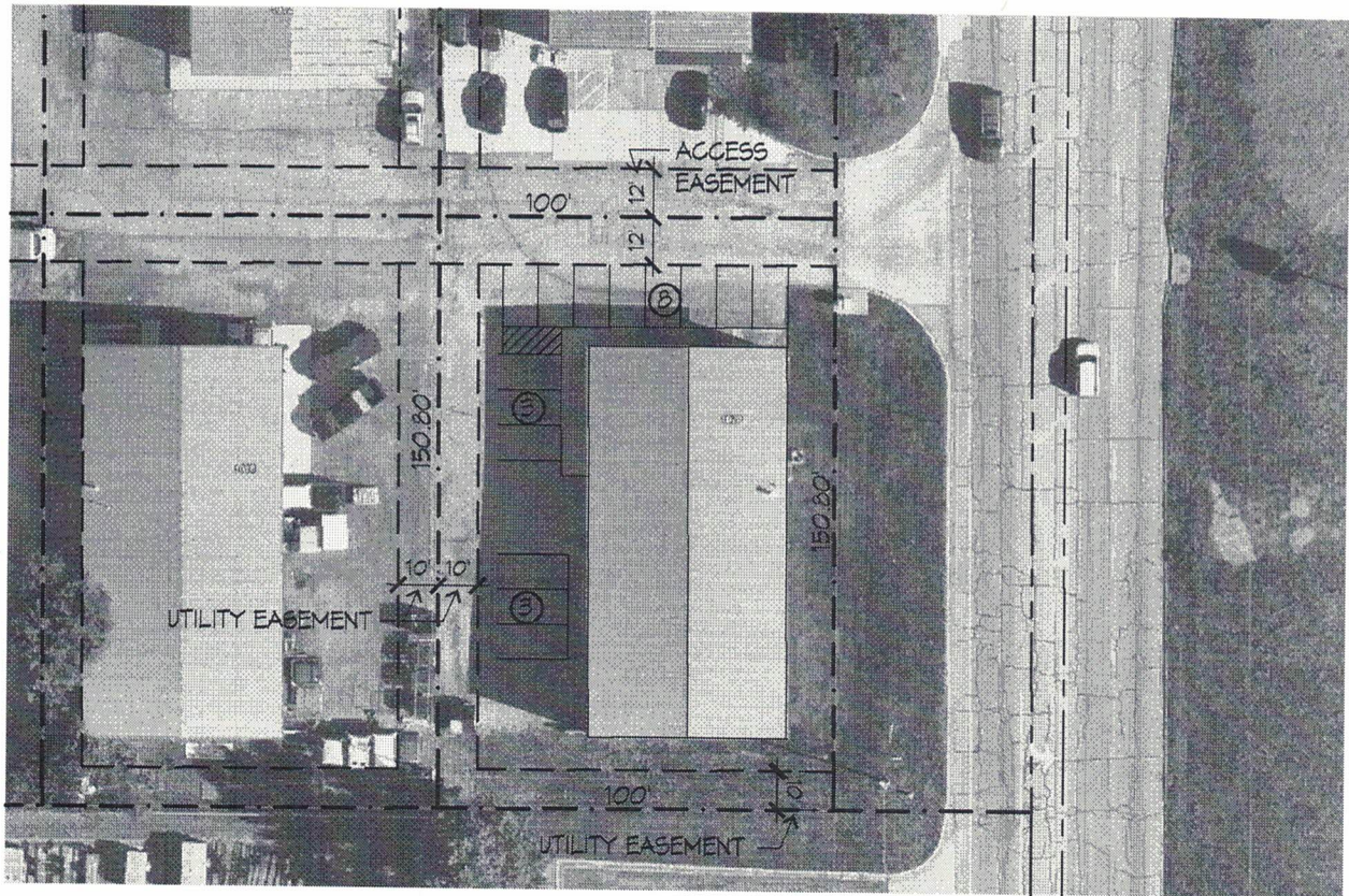
SITE PLAN
