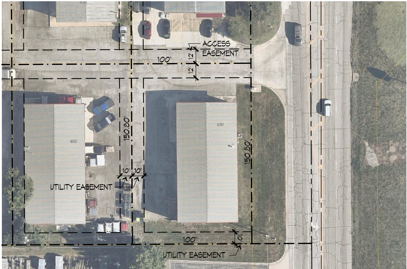
SITE PLAN
