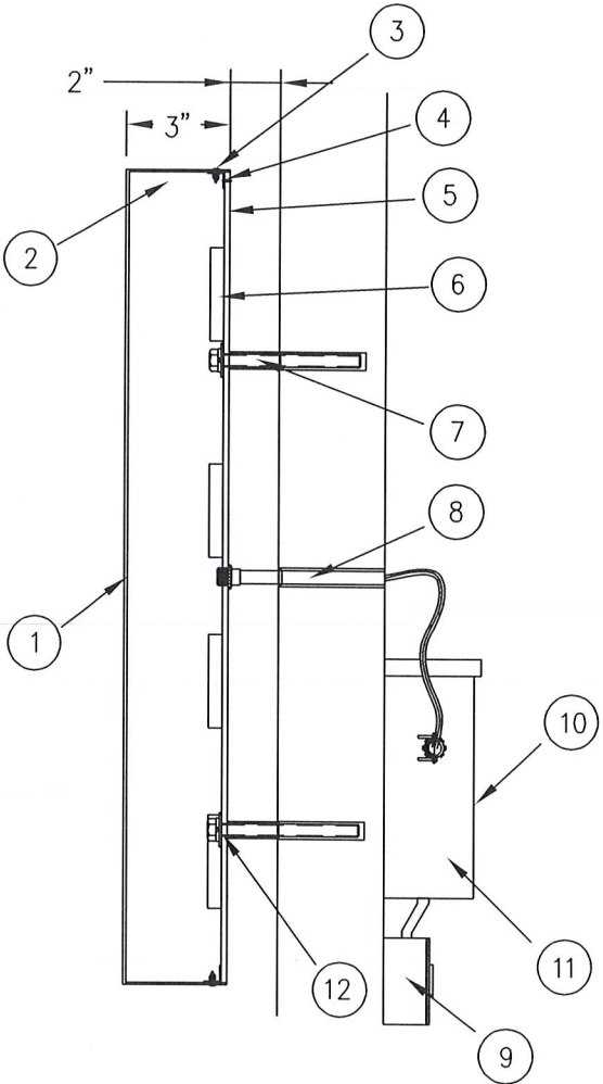
SECTION VIEW SCALE: 1/2"=1'-0"
