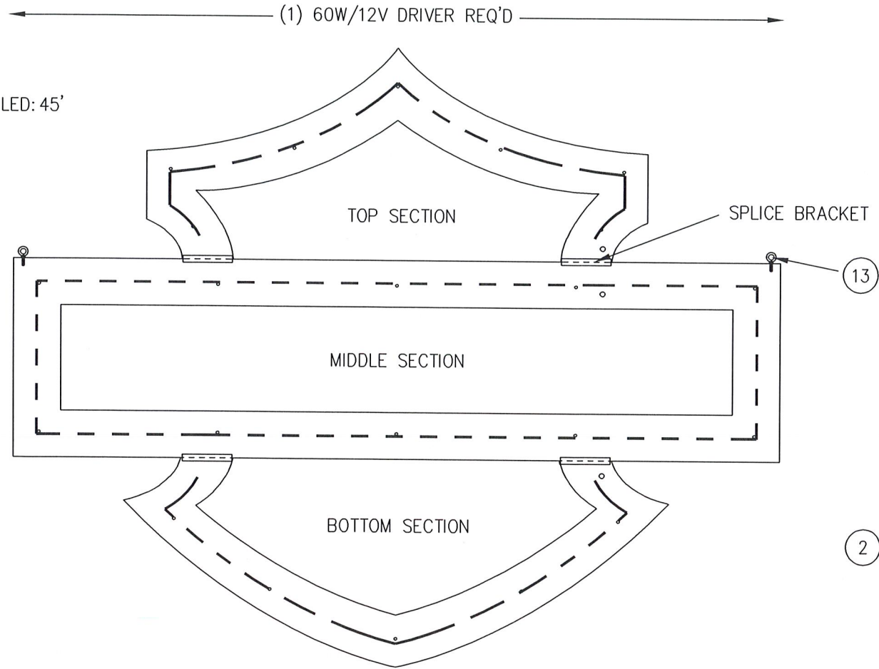
LED LAYOUT SCALE: 1/2"=1'-0"
