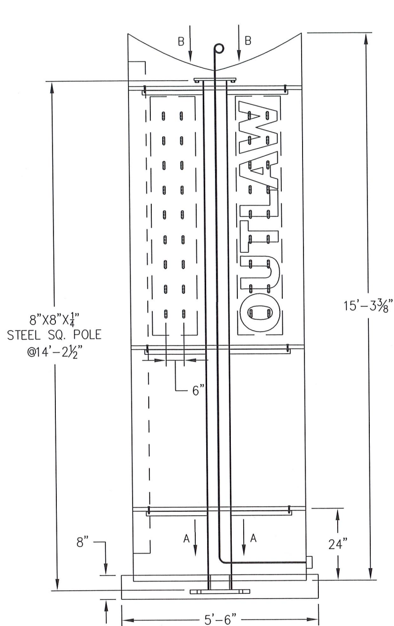
FRONT VIEW SCALE: 3/8"=1'-0"
