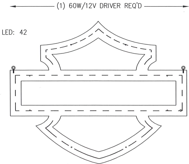
LED LAYOUT SCALE: 1/2"=1'-0"
