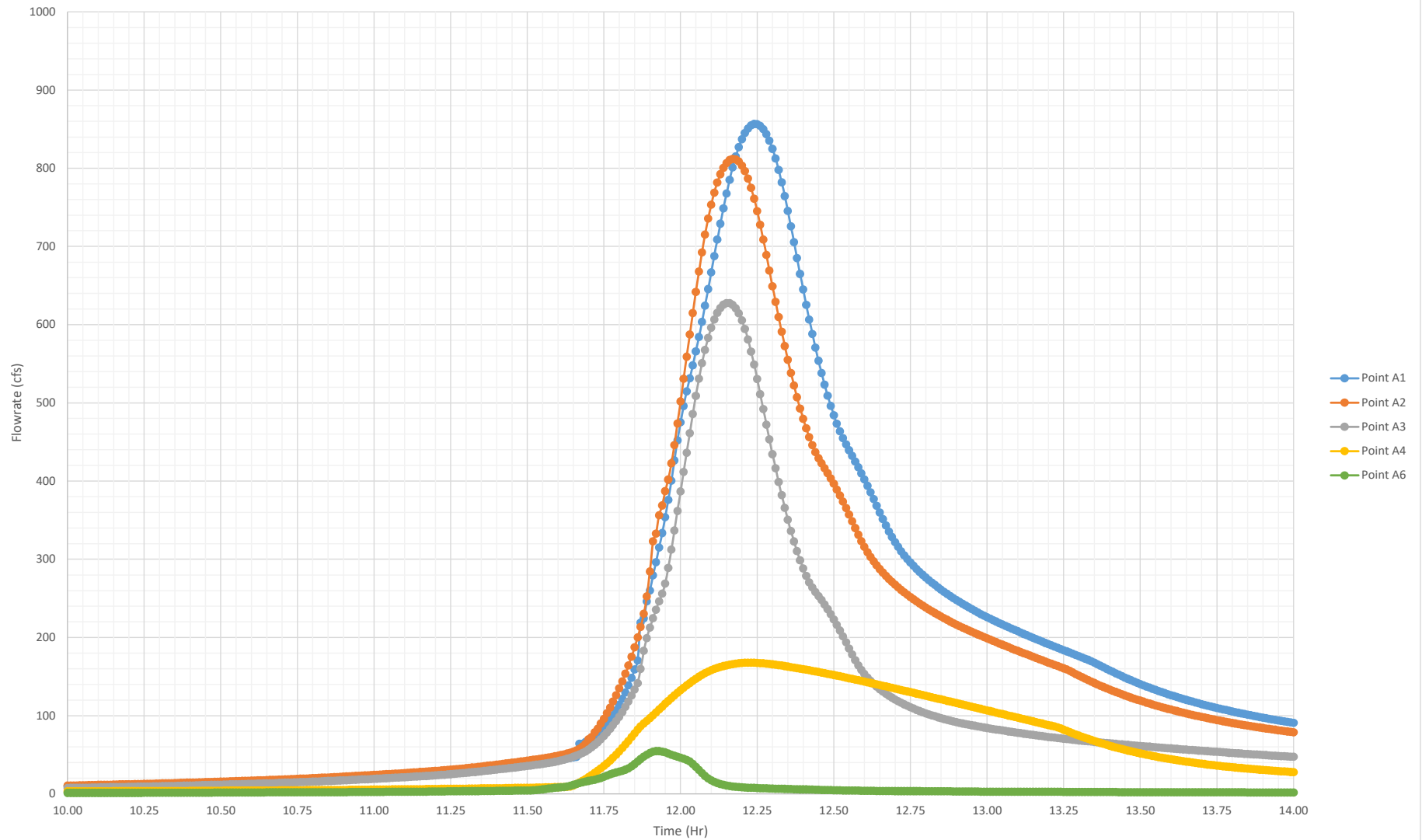
Proposed Peak 4-Hr 50% Flowrates (Fully Developed)
