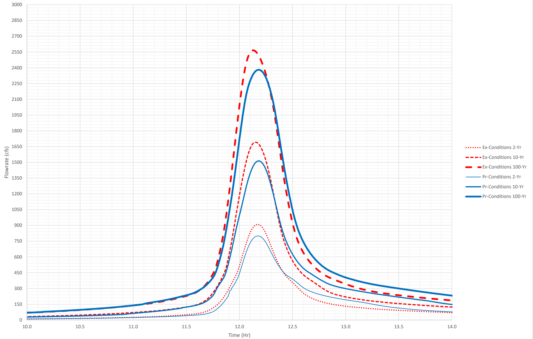
Existing & Proposed Conditions Point A2 Hydrograph
