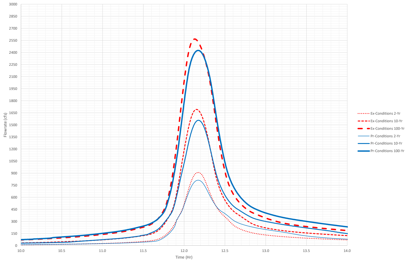
Existing & Fully-Developed Conditions Point A2 Hydrograph
