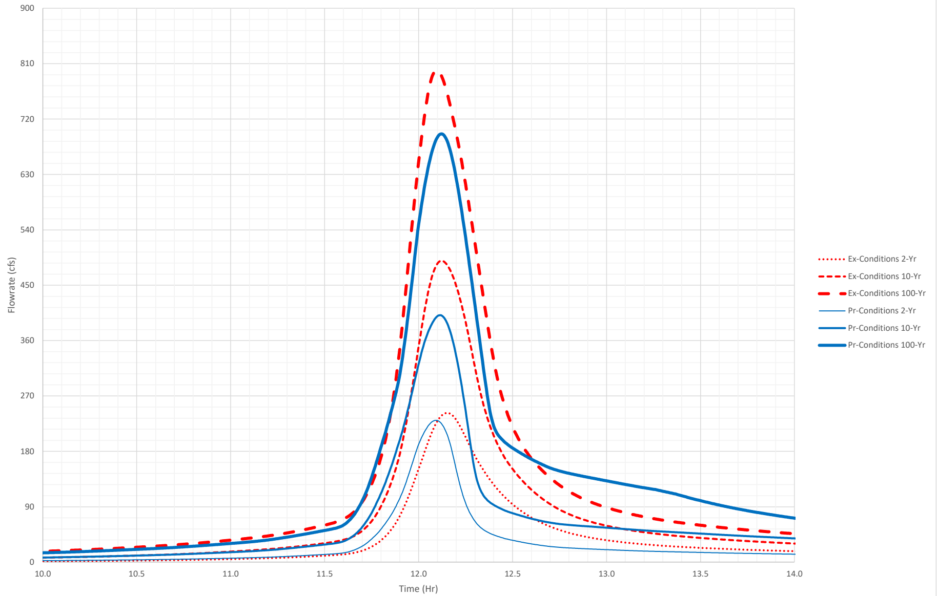
Existing & Proposed Conditions Point A5 Hydrograph
