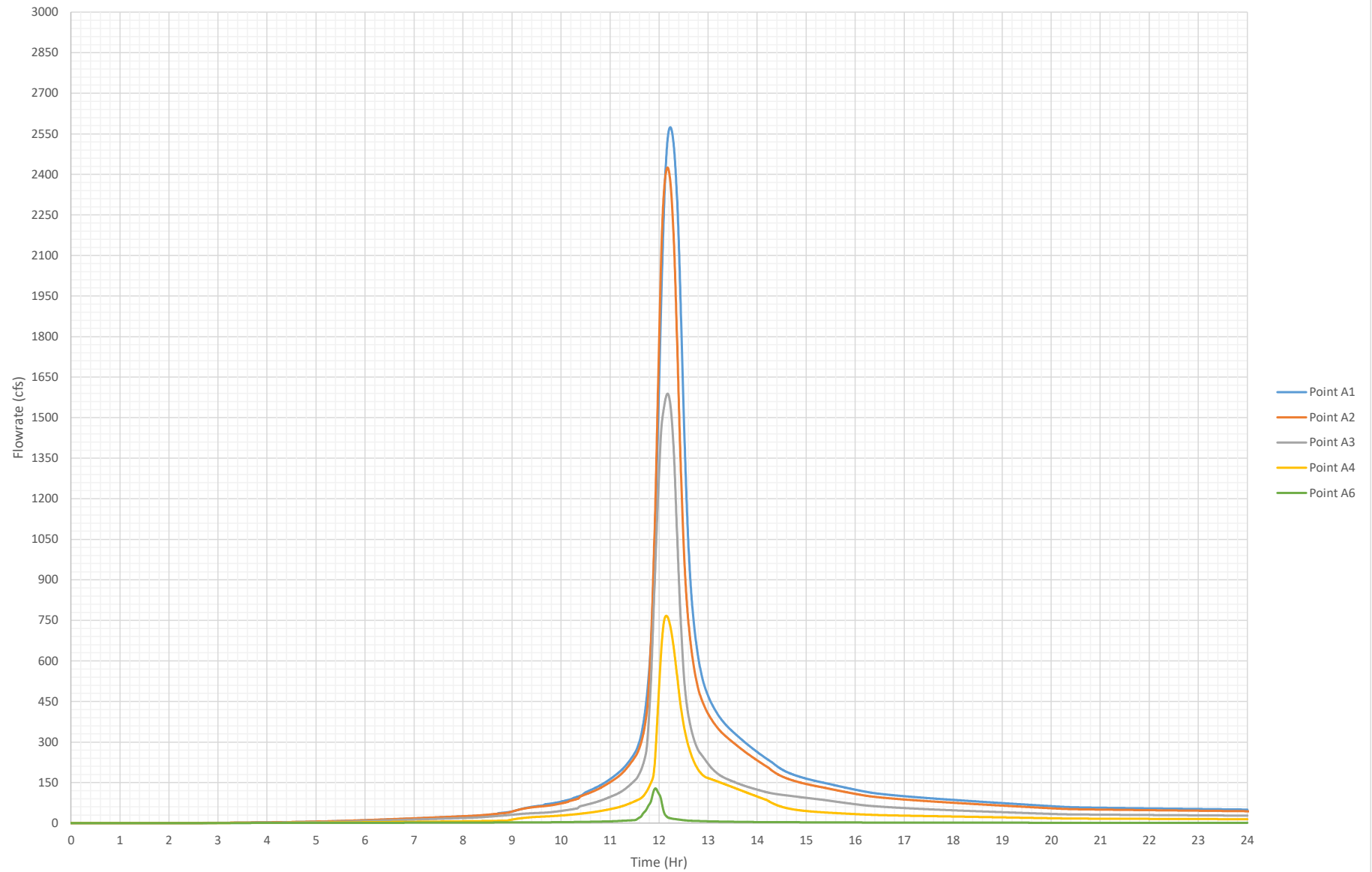
Proposed Peak 24-Hr 1% Flowrates (Fully Developed)
