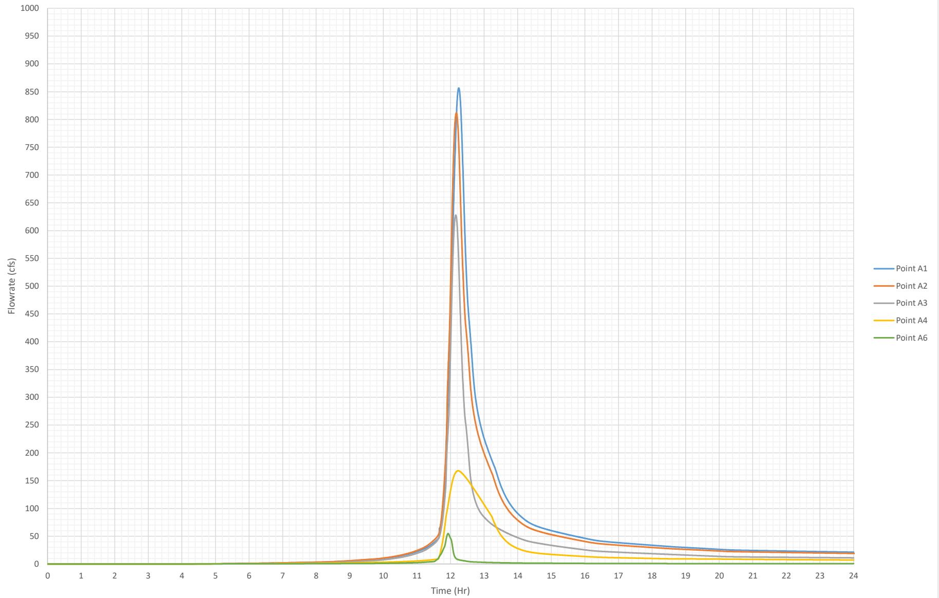
Proposed Peak 24-Hr 50% Flowrates (Fully Developed)
