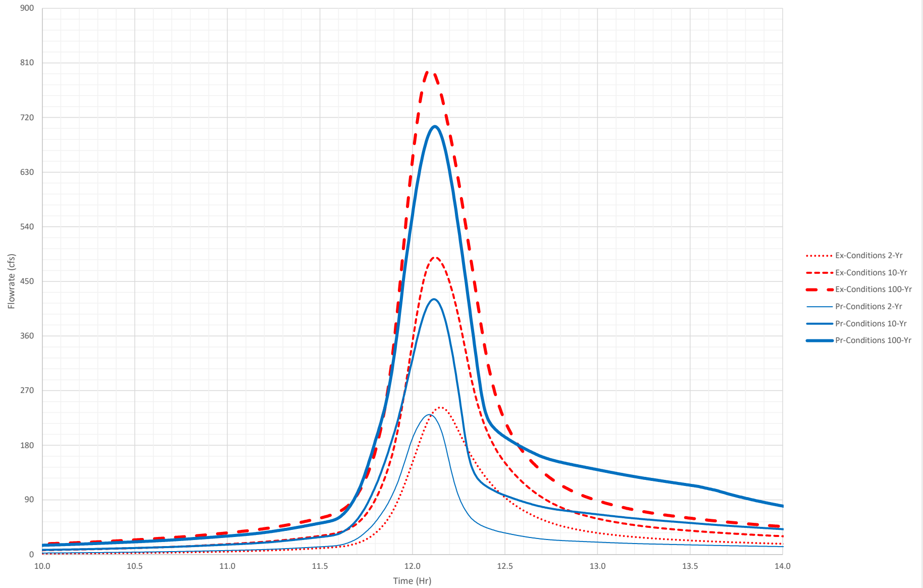
Existing & Fully-Developed Conditions Point A5 Hydrograph
