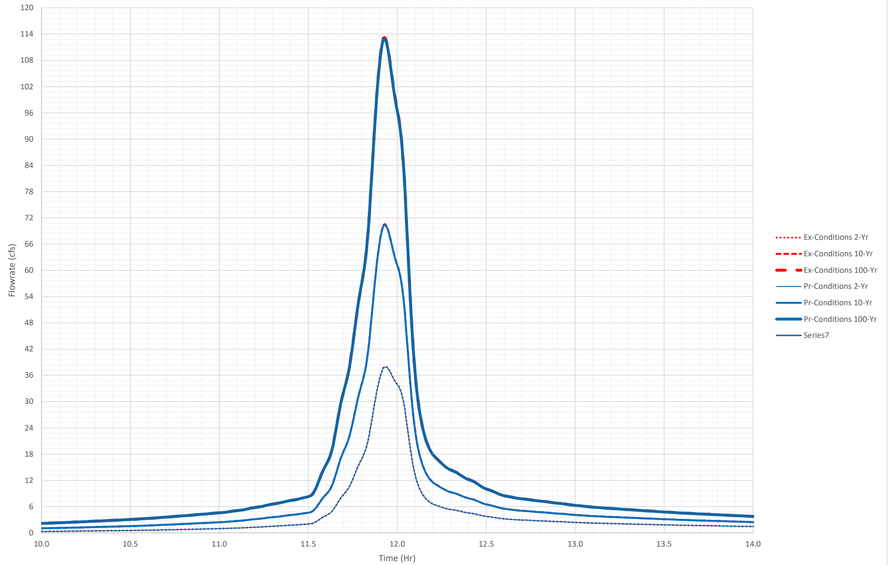
Existing & Proposed Conditions Point A6 Hydrograph
