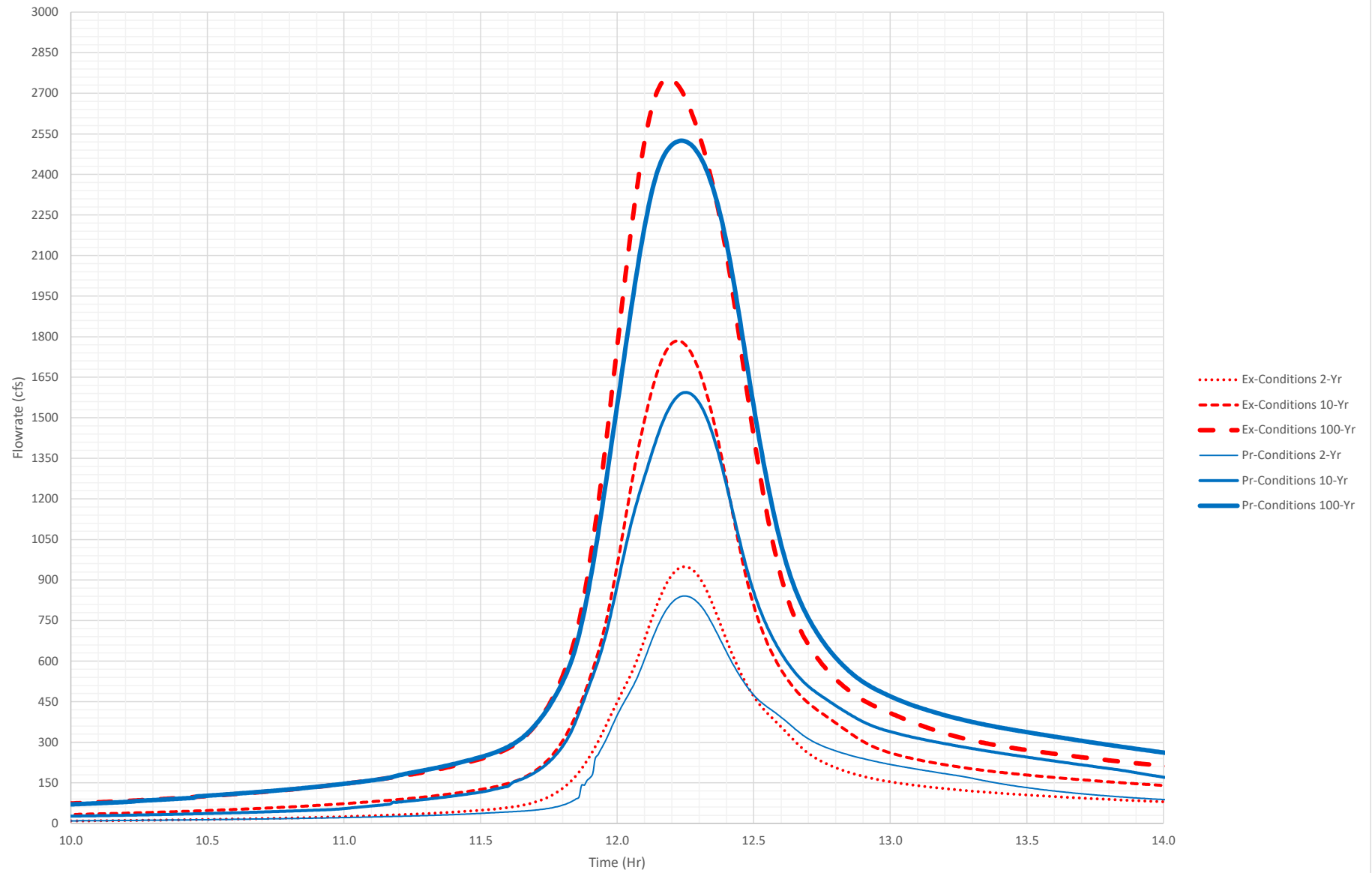
Existing & Proposed Conditions Point A1 Hydrograph
