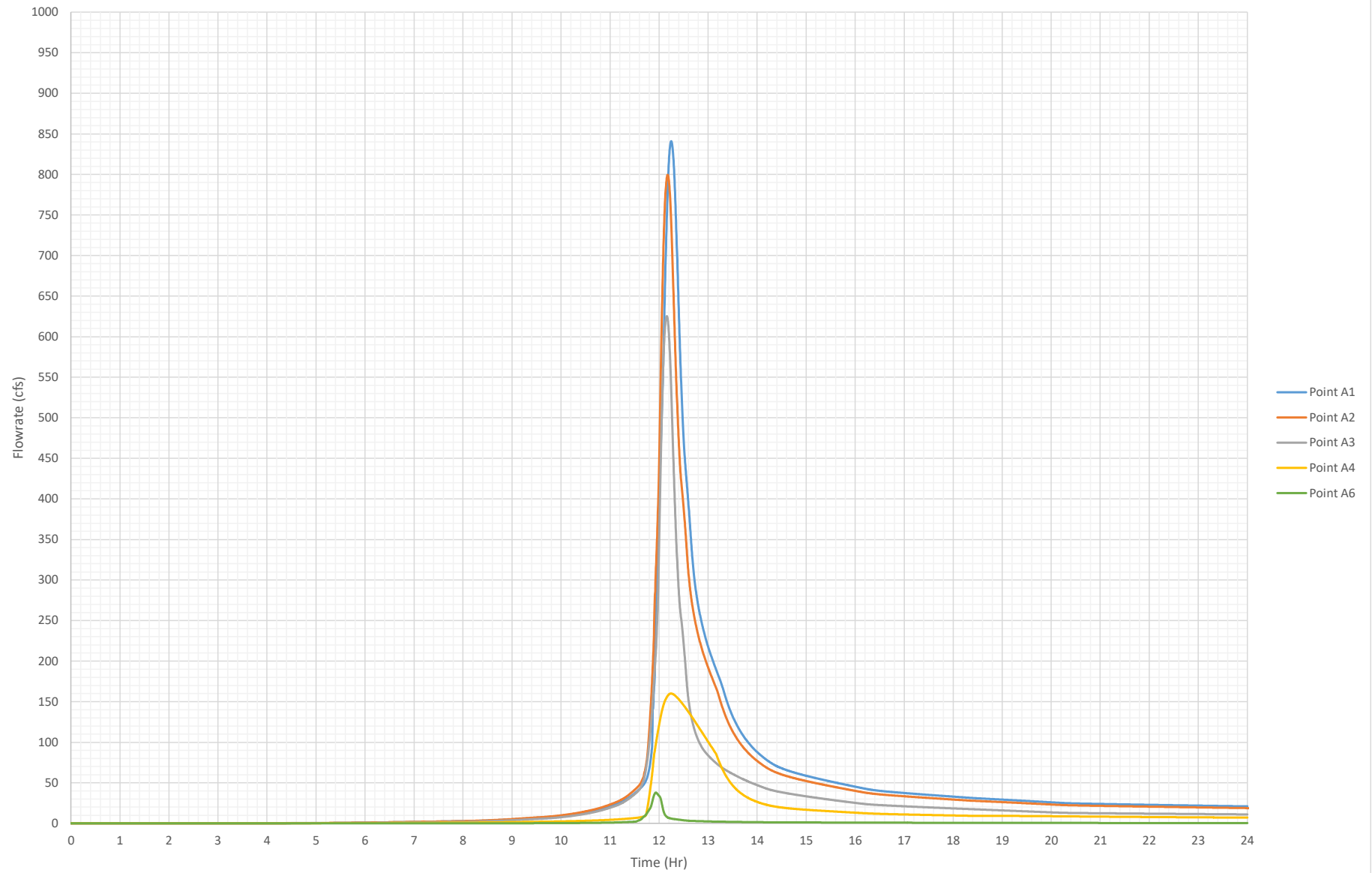
Proposed Peak 24-Hr 50% Flowrates
