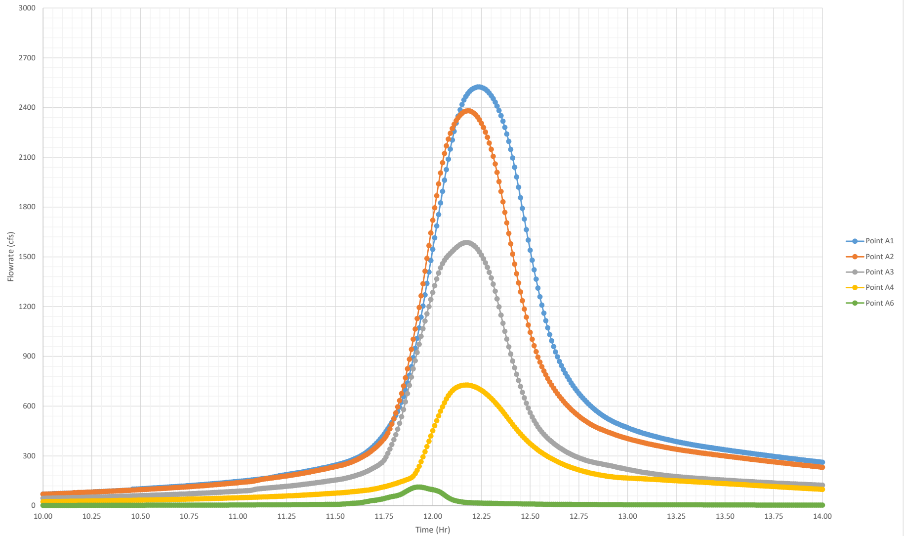
Proposed Peak 4-Hr 1% Flowrates
