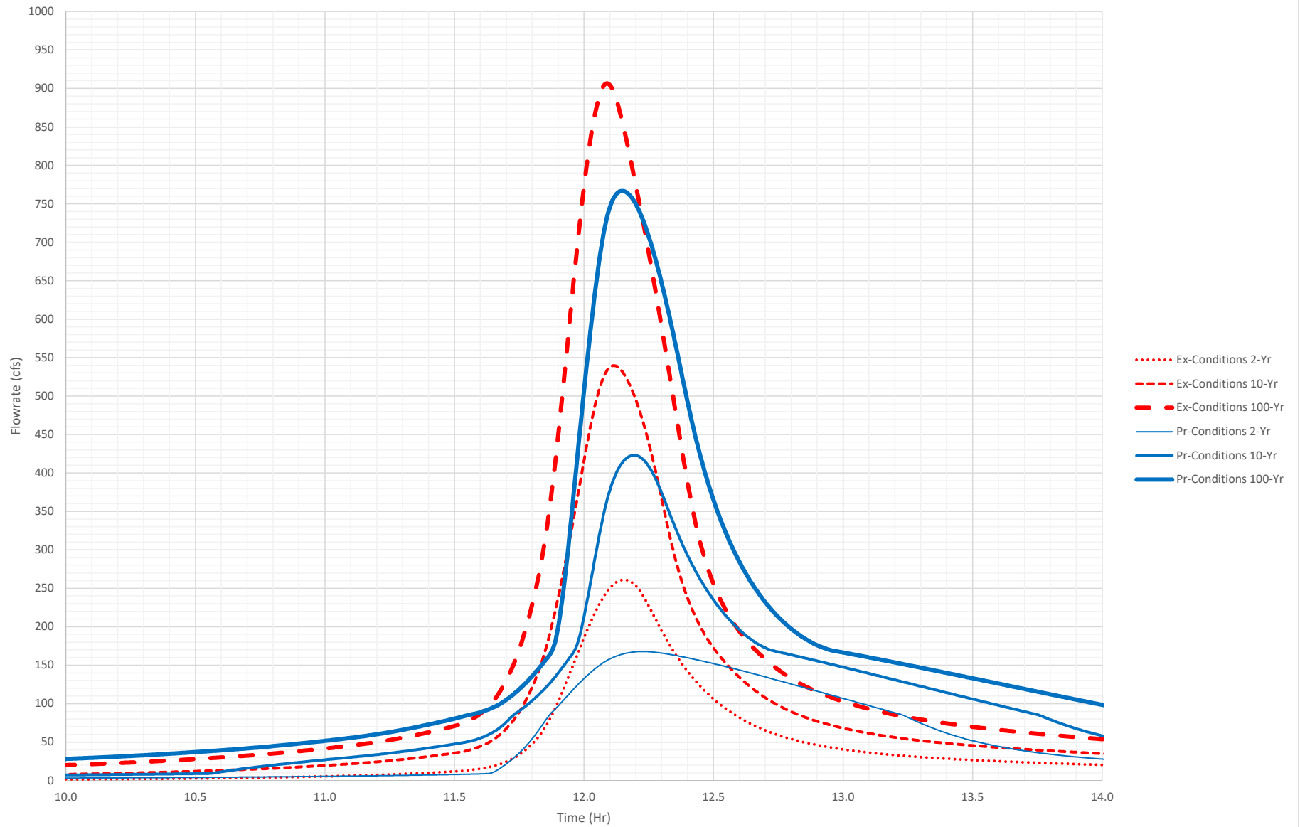
Existing & Fully-Developed Conditions Point A4 Hydrograph
