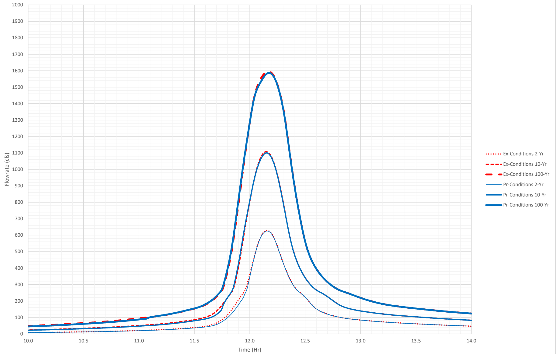
Existing & Proposed Conditions Point A3 Hydrograph
