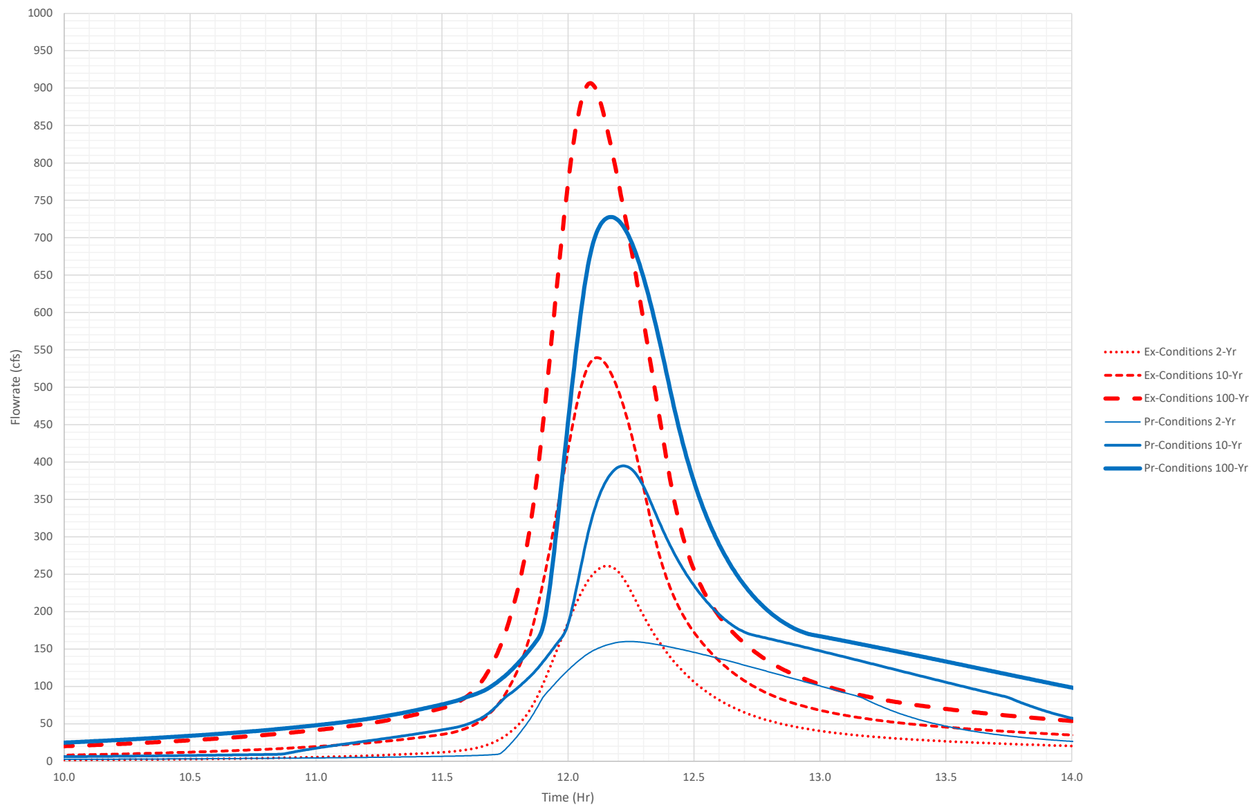
Existing & Proposed Conditions Point A4 Hydrograph
