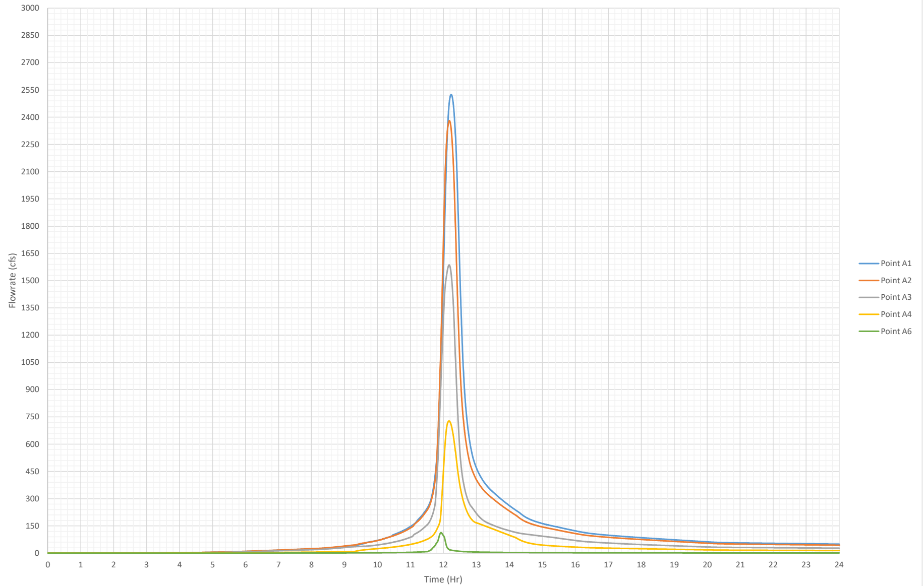
Proposed Peak 24-Hr 1% Flowrates
