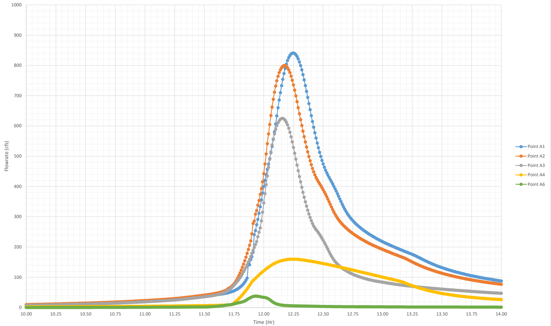
Proposed Peak 4-Hr 50% Flowrates
