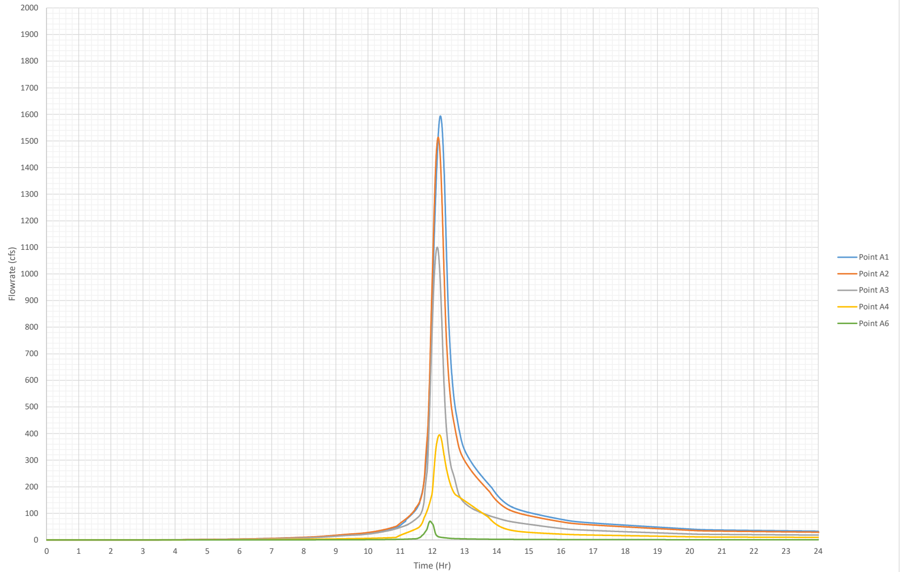
Proposed Peak 24-Hr 10% Flowrates
