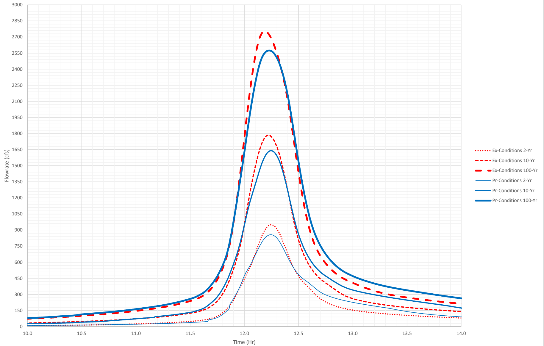
Existing & Fully-Developed Conditions Point A1 Hydrograph
