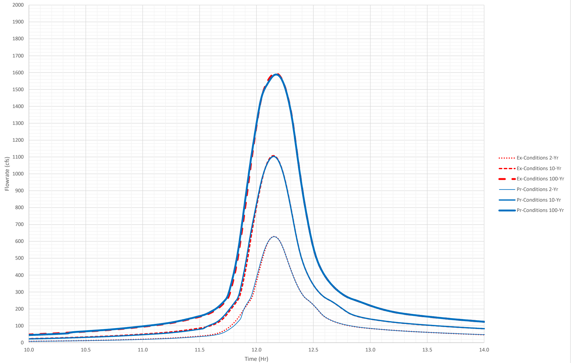
Existing & Fully-Developed Conditions Point A3 Hydrograph
