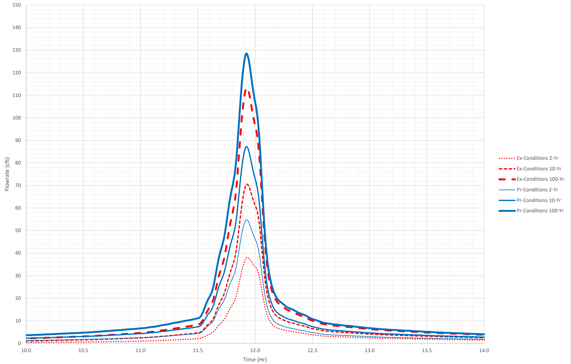
Existing & Fully-Developed Conditions Point A6 Hydrograph
