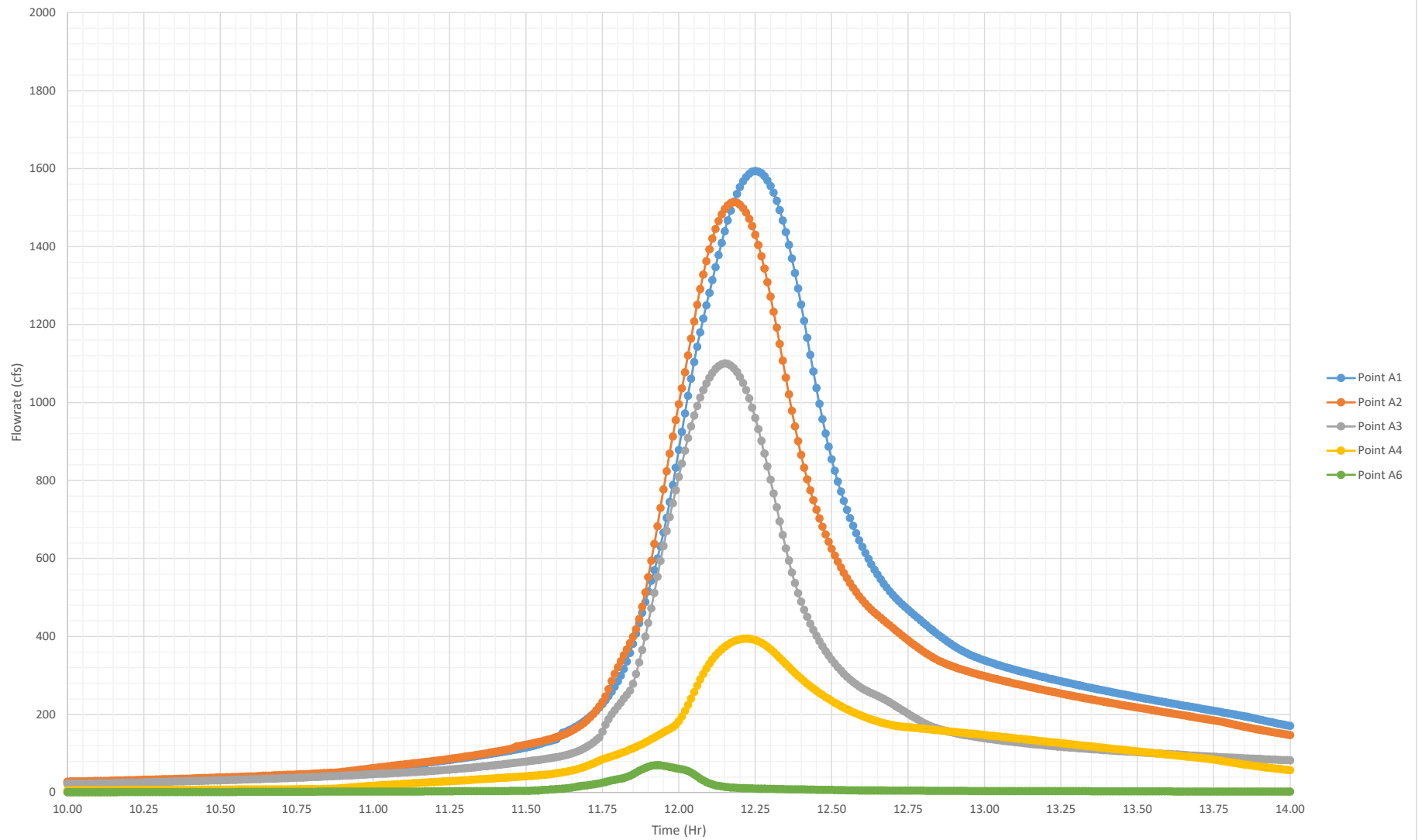
Proposed Peak 4-Hr 10% Flowrates
