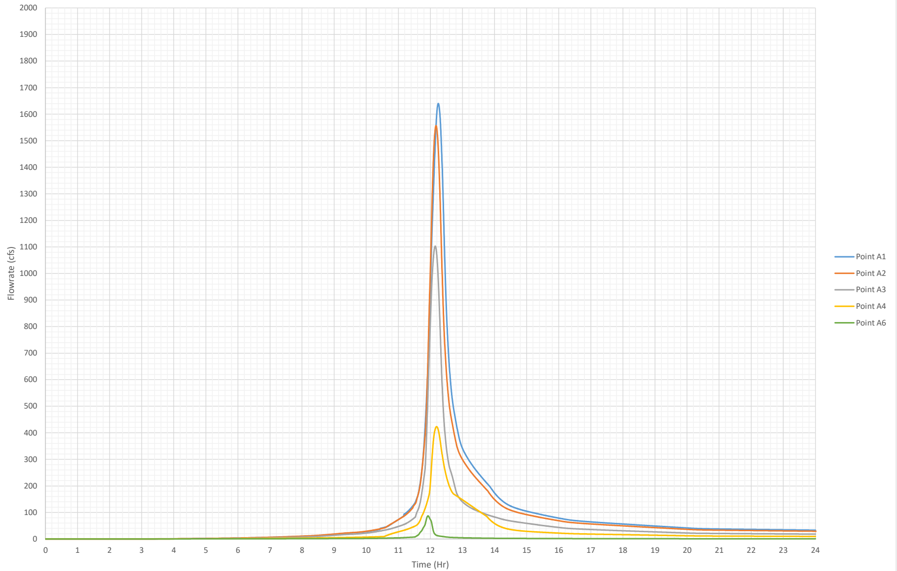
Proposed Peak 24-Hr 10% Flowrates (Fully Developed)
