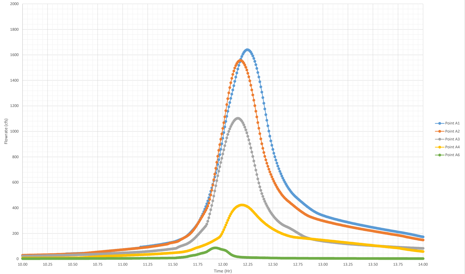
Proposed Peak 4-Hr 10% Flowrates (Fully Developed)
