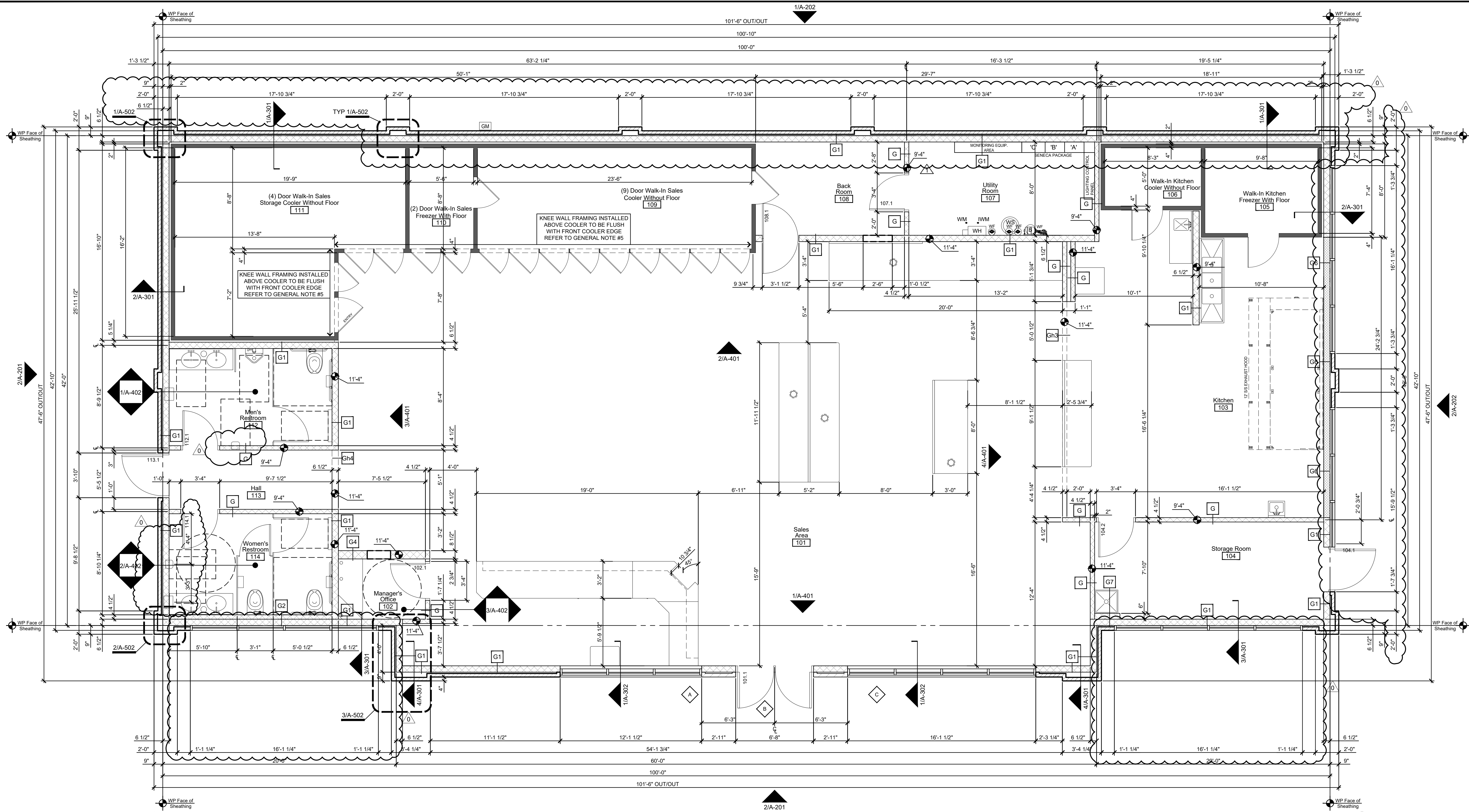
1 Floor Plan 1/4"=1'-0"
