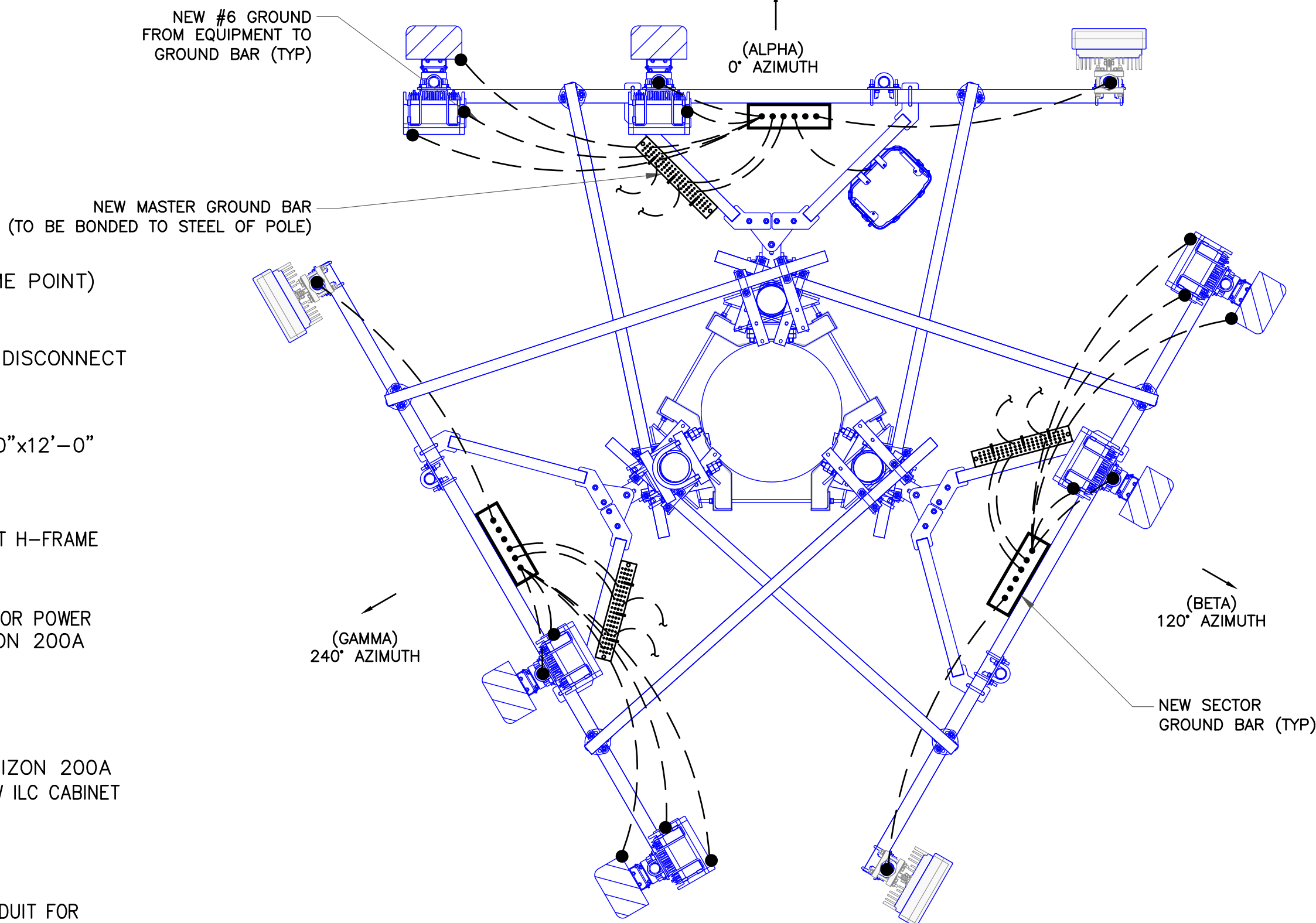
1 ANTENNA GROUNDING PLAN SCALE: NOT TO SCALE
