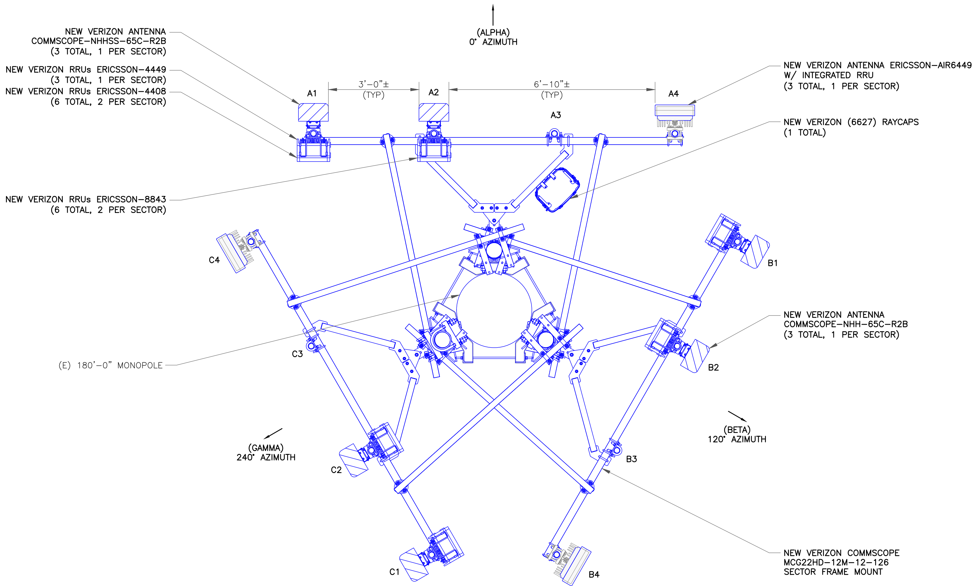
2 FINAL ANTENNA PLAN SCALE: NOT TO SCALE
