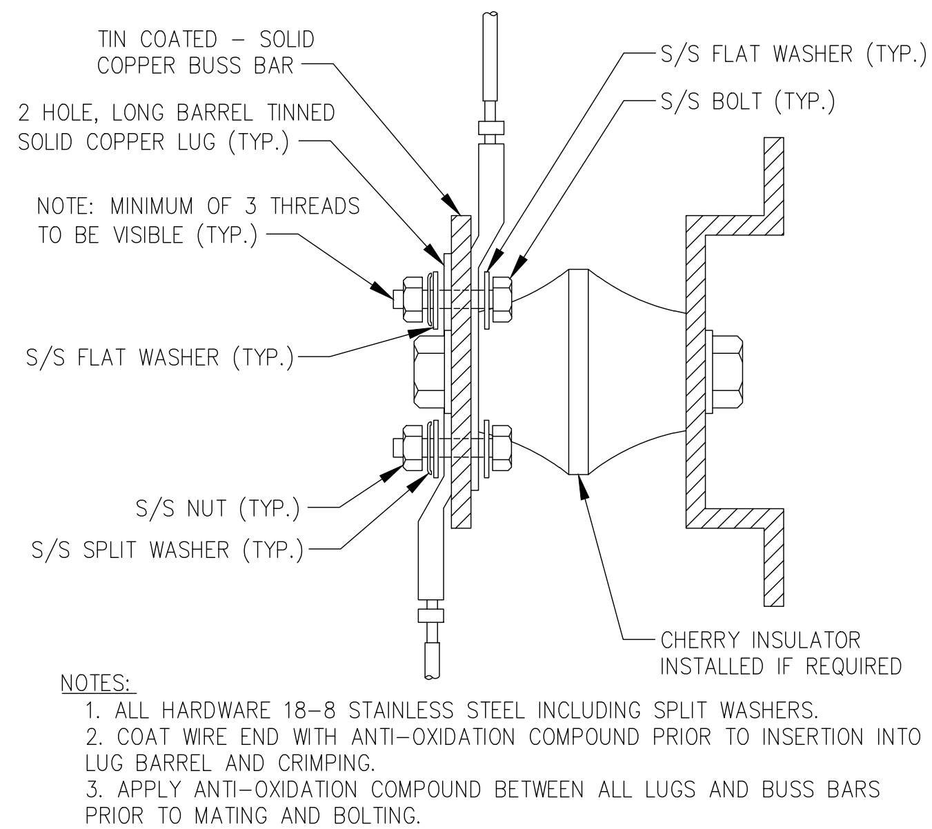
3 TYPICAL GROUND LUG SCALE: NOT TO SCALE
