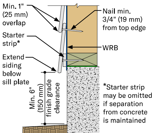
Siding - Direct to Stud Attachment
