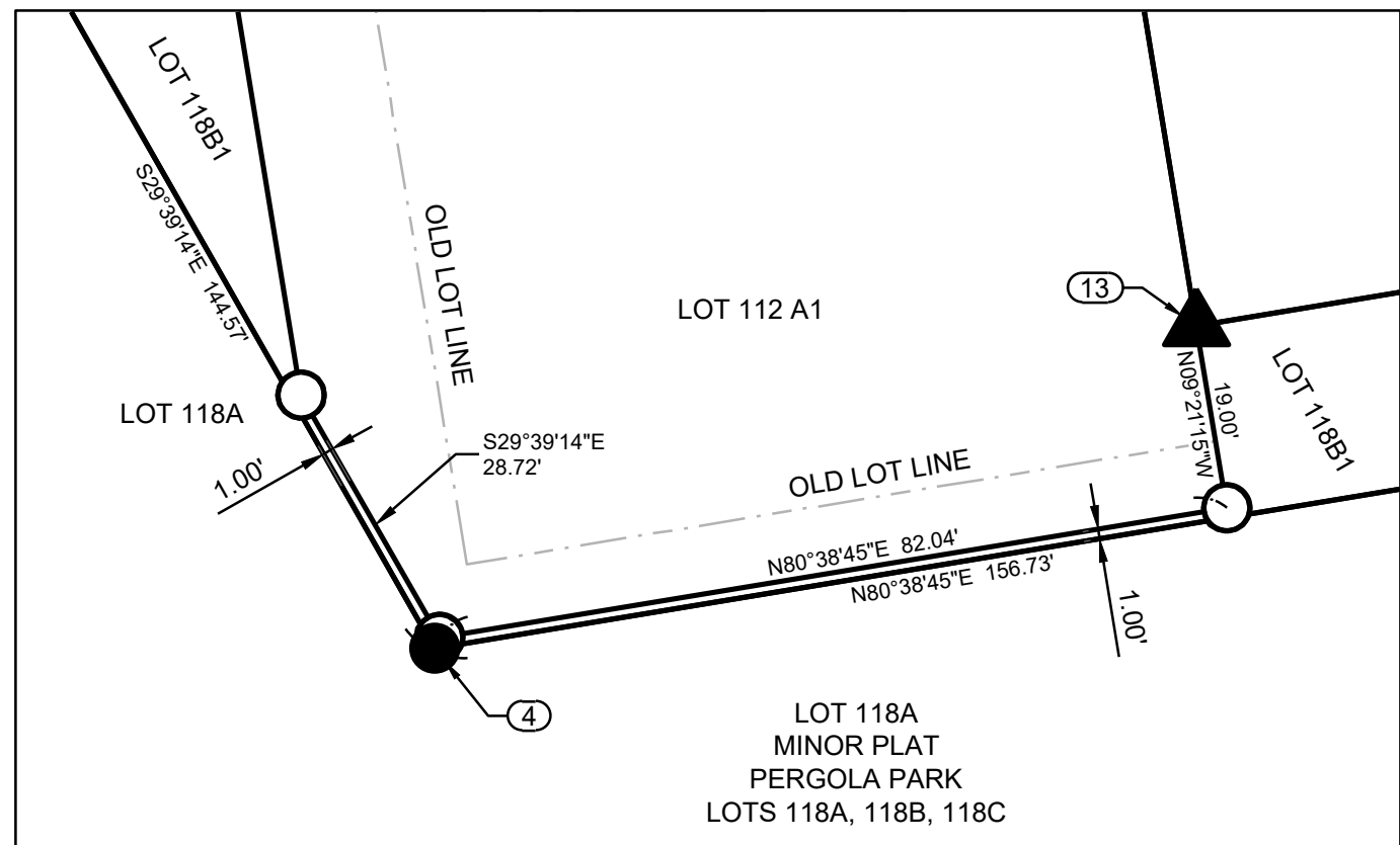
DETAIL LOT 112A1 1"=20'
