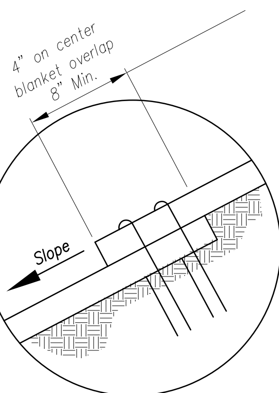
Splice Seam
