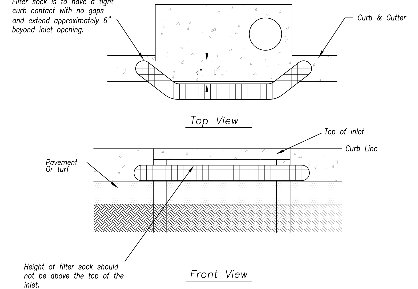
Sump Inlet Sediment Filter
