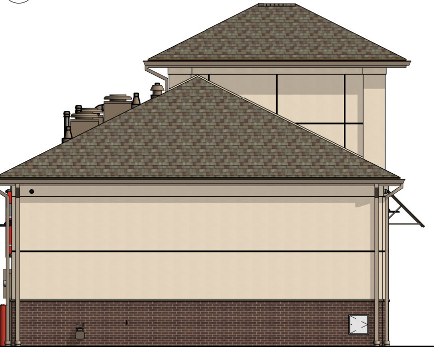
4 OVERALL LEFT SIDE EXTERIOR ELEVATION (LEFT) Scale: 1/8" = 1'-0"
