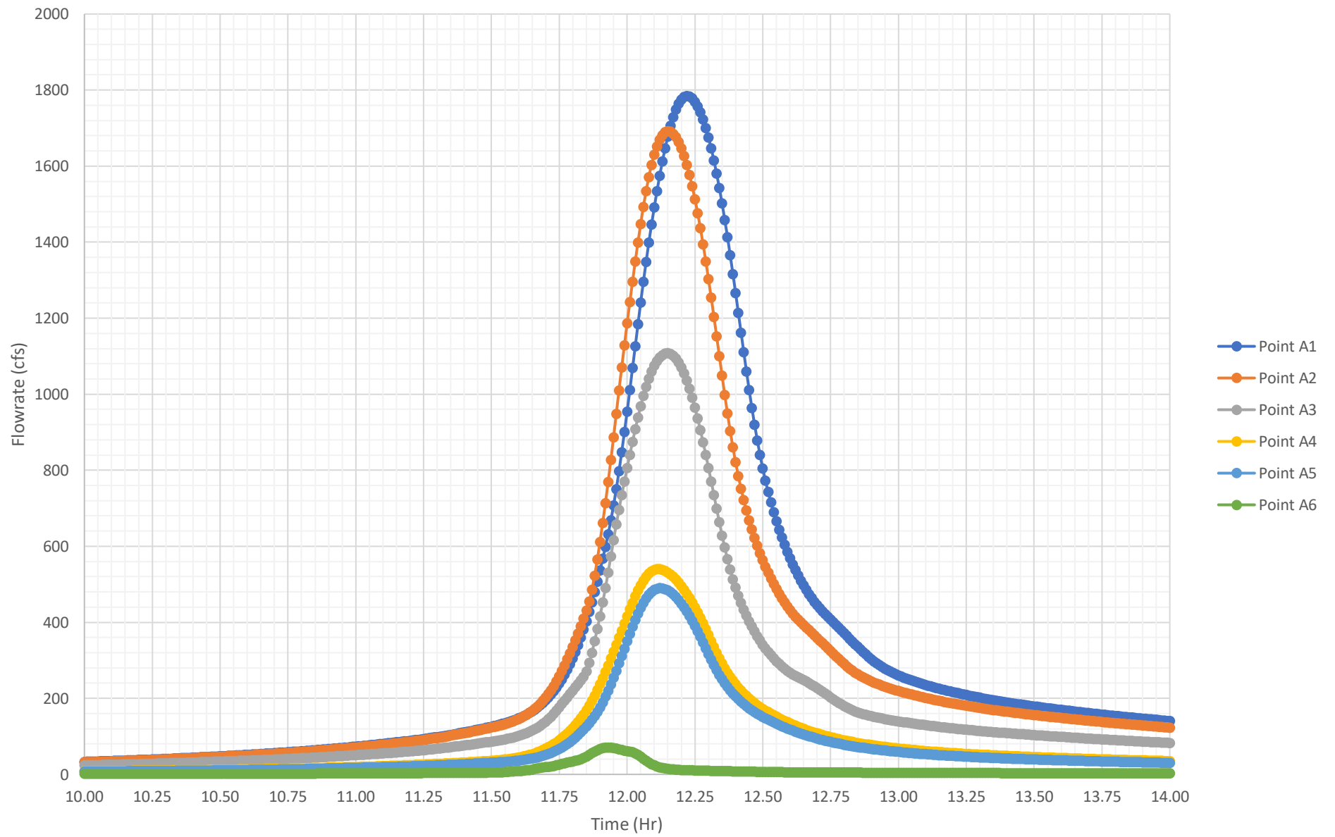
Existing Peak 4-Hr 10% Flowrates (Macro)
