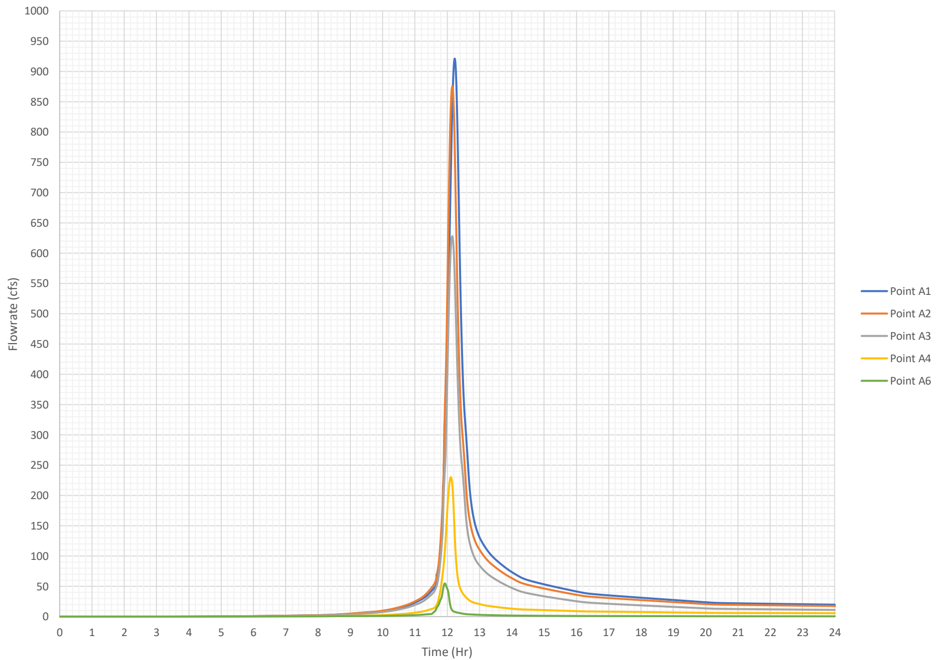
Proposed Peak 24-Hr 50% Flowrates (Macro)
