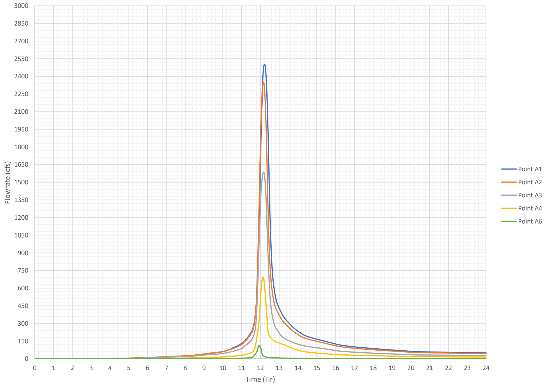
Proposed Peak 24-Hr 1% Flowrates (Micro)
