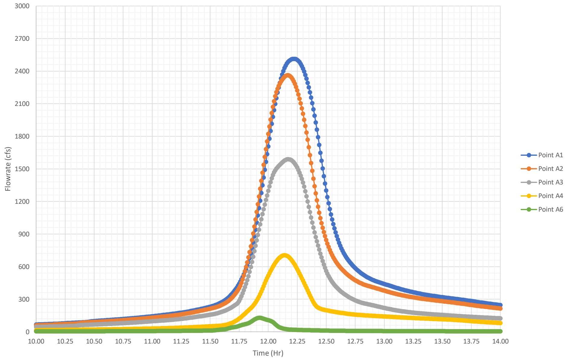
Proposed Peak 4-Hr 1% Flowrates (Macro)
