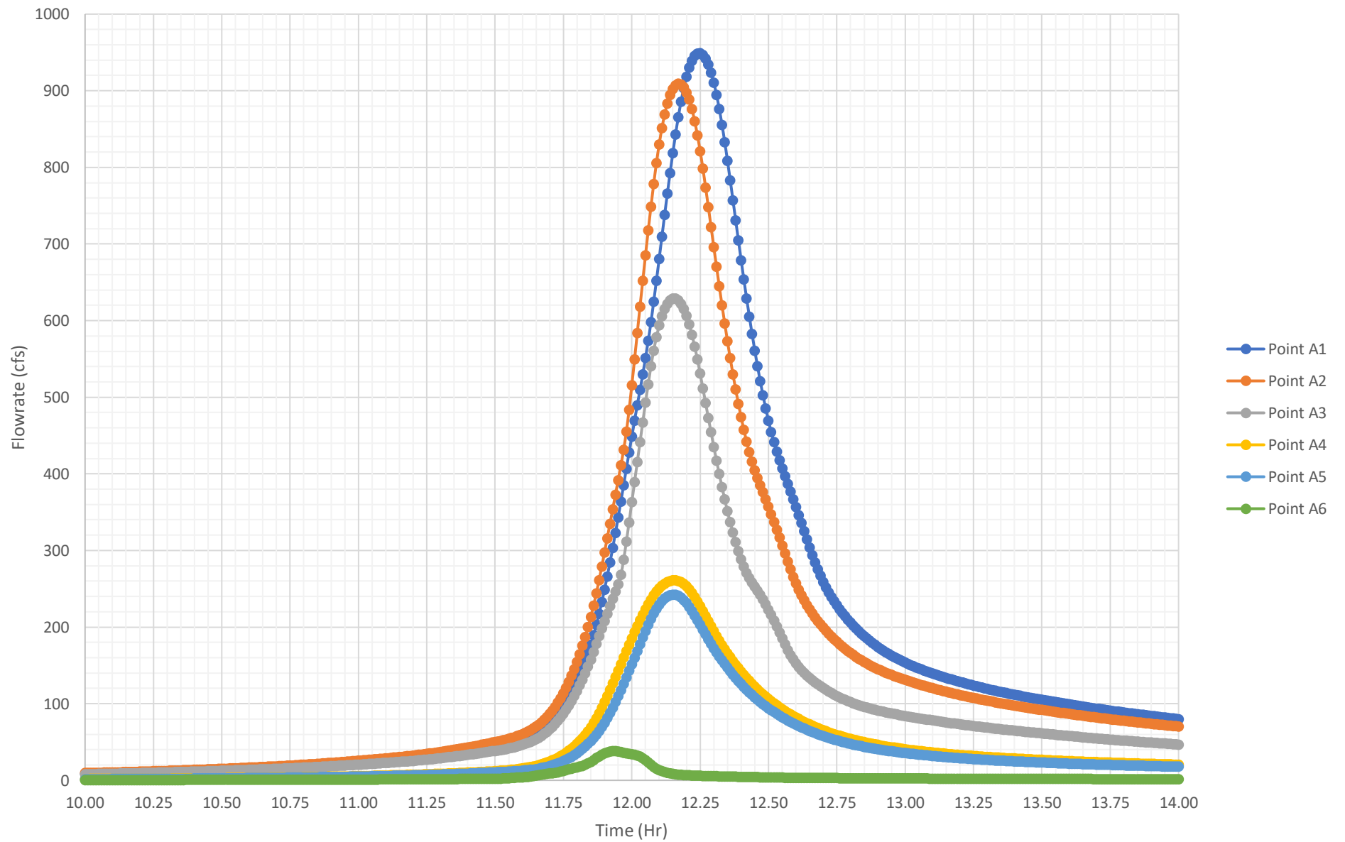
Existing Peak 4-Hr 50% Flowrates (Macro)
