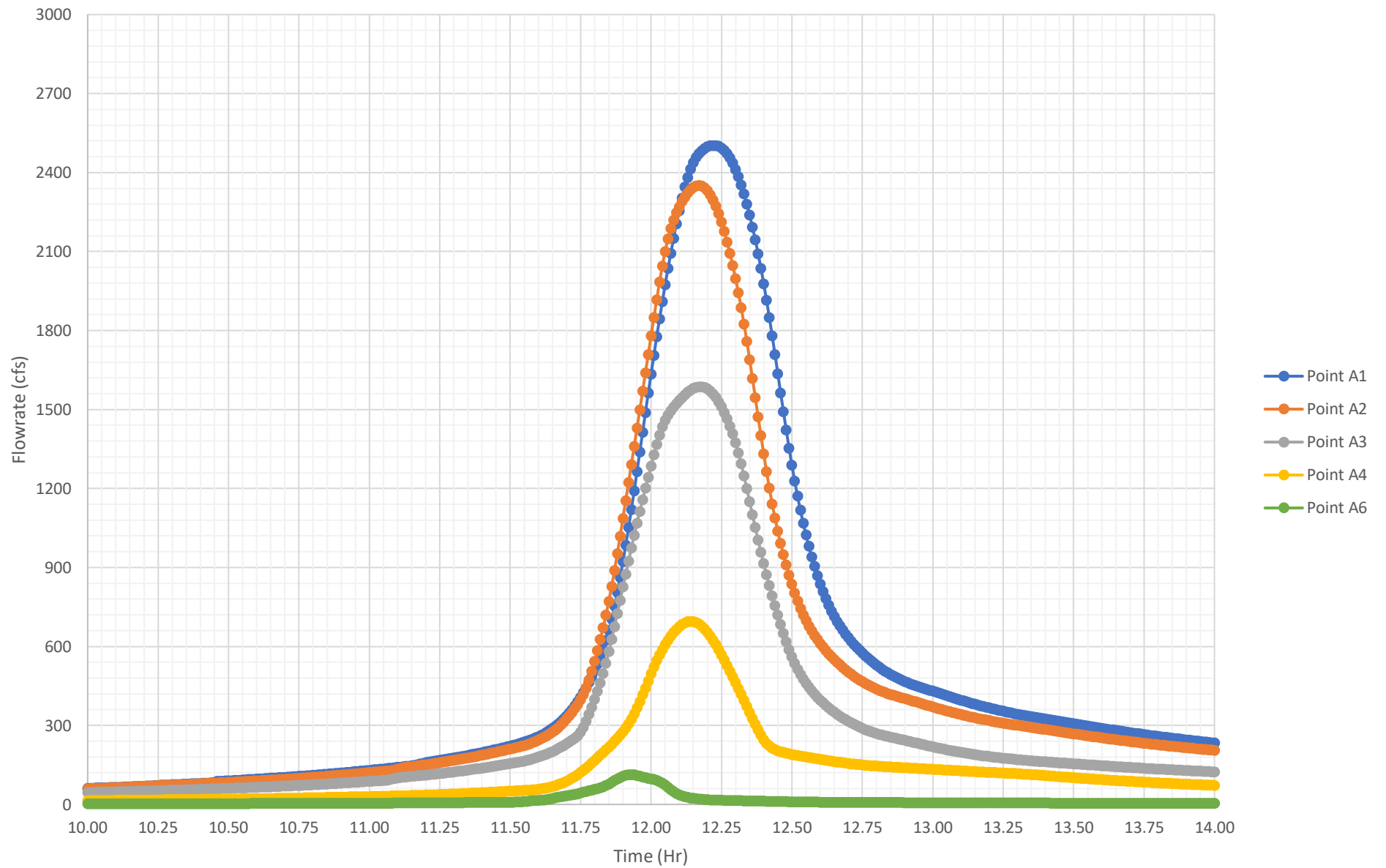
Proposed Peak 4-Hr 1% Flowrates (Micro)
