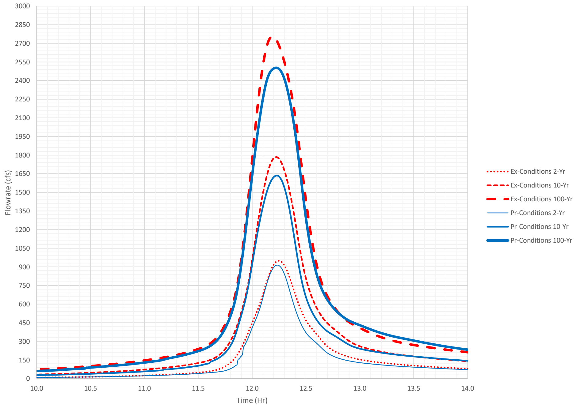
Existing & Proposed Conditions Point A1 Hydrograph(Micro)
