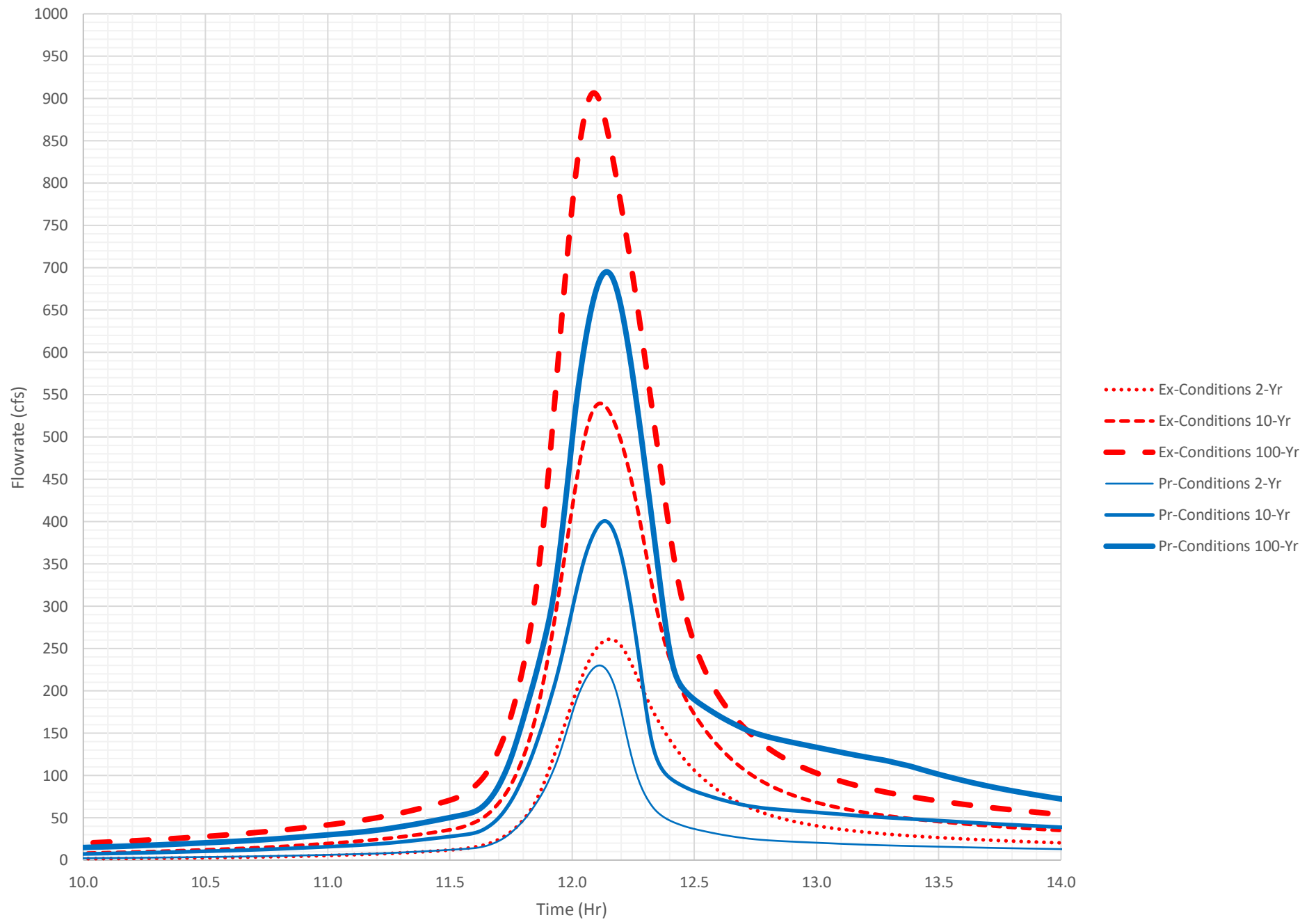
Existing & Proposed Conditions Point A4 Hydrograph(Micro)
