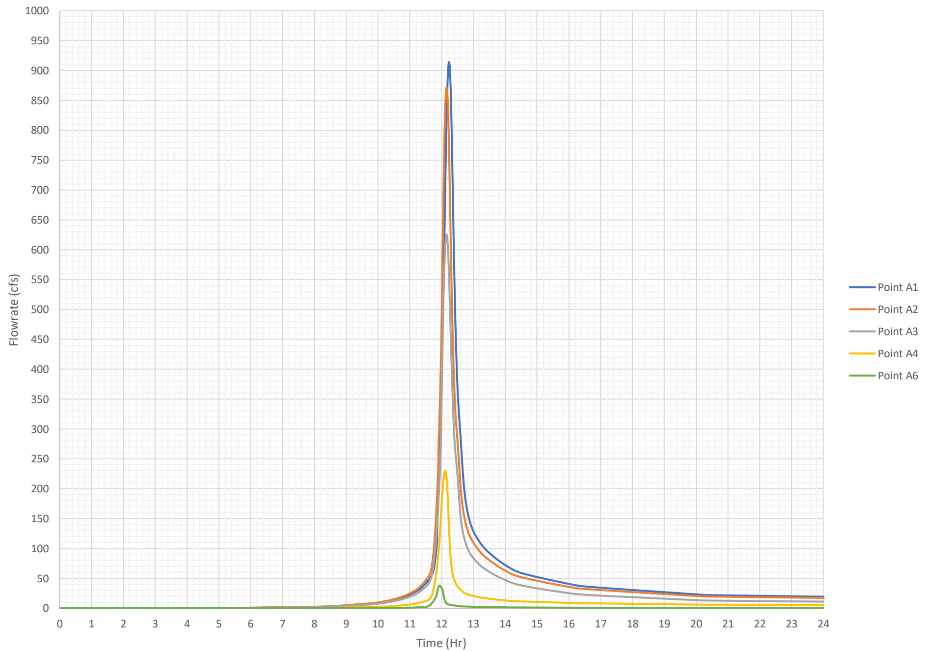
Proposed Peak 24-Hr 50% Flowrates (Micro)
