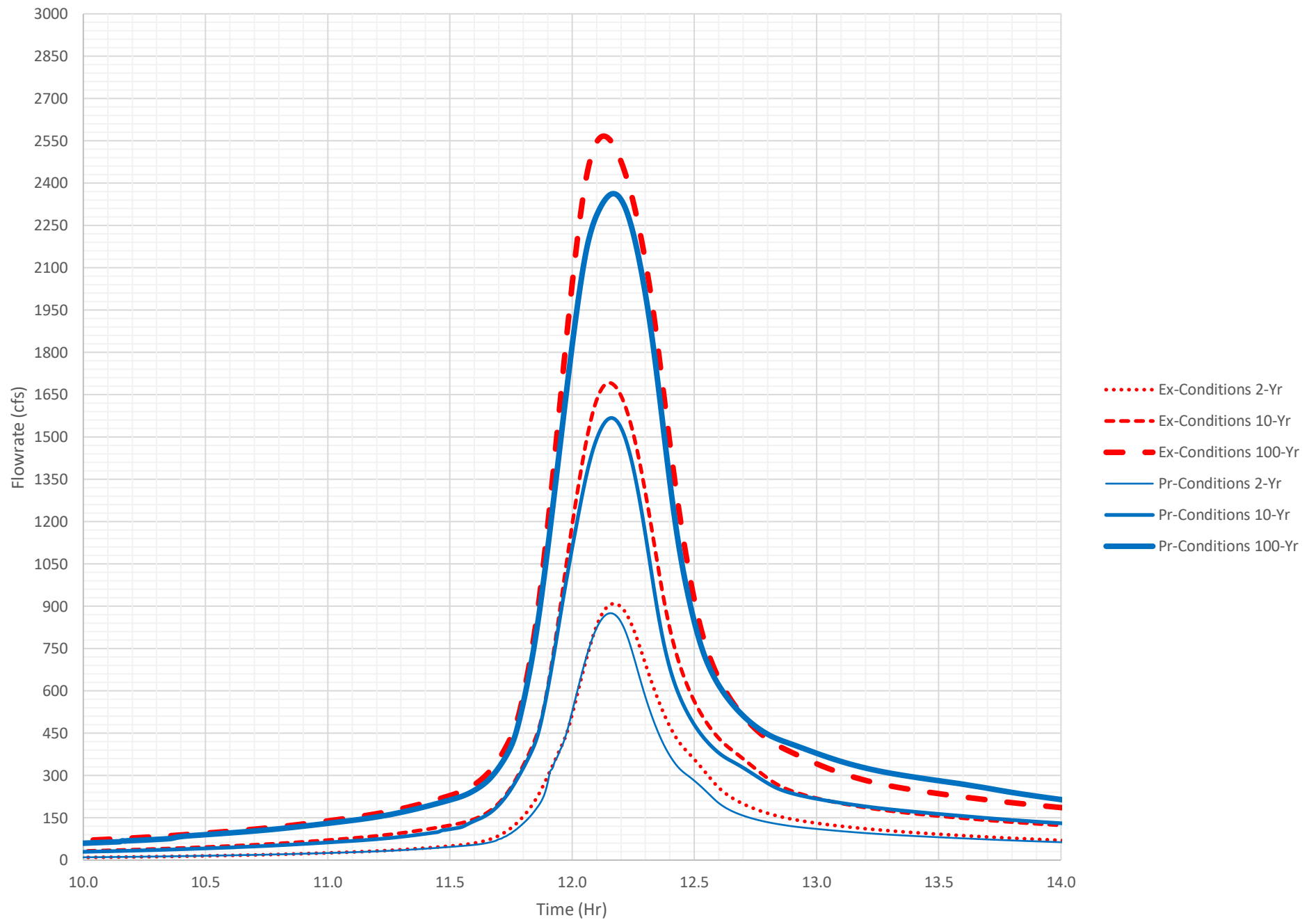
Existing & Proposed Conditions Point A2 Hydrograph(Fully-Developed)
