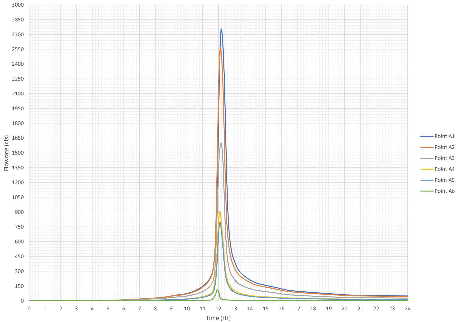
Existing Peak 24-Hr 1% Flowrates (Macro)
