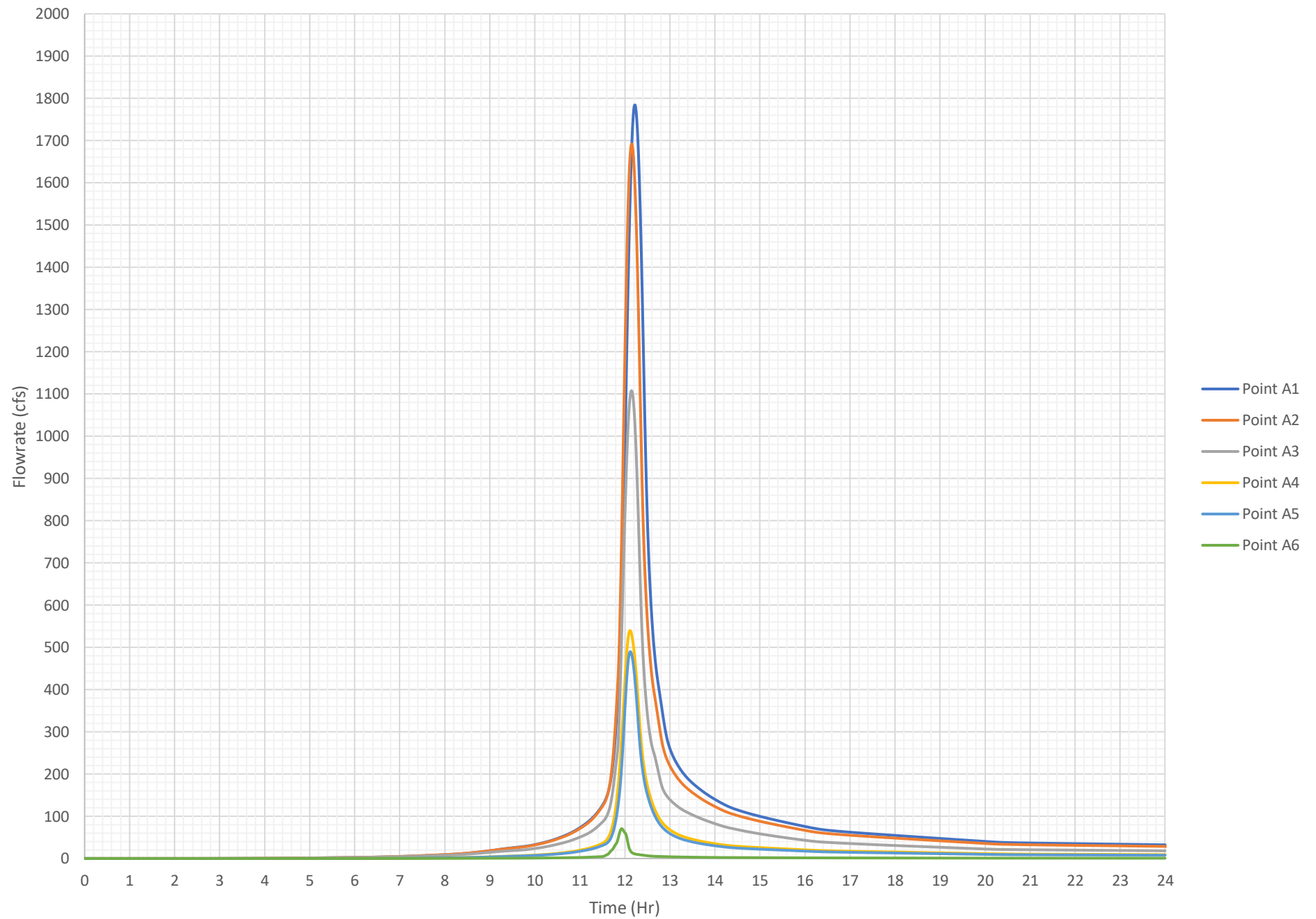
Existing Peak 24-Hr 10% Flowrates (Macro)
