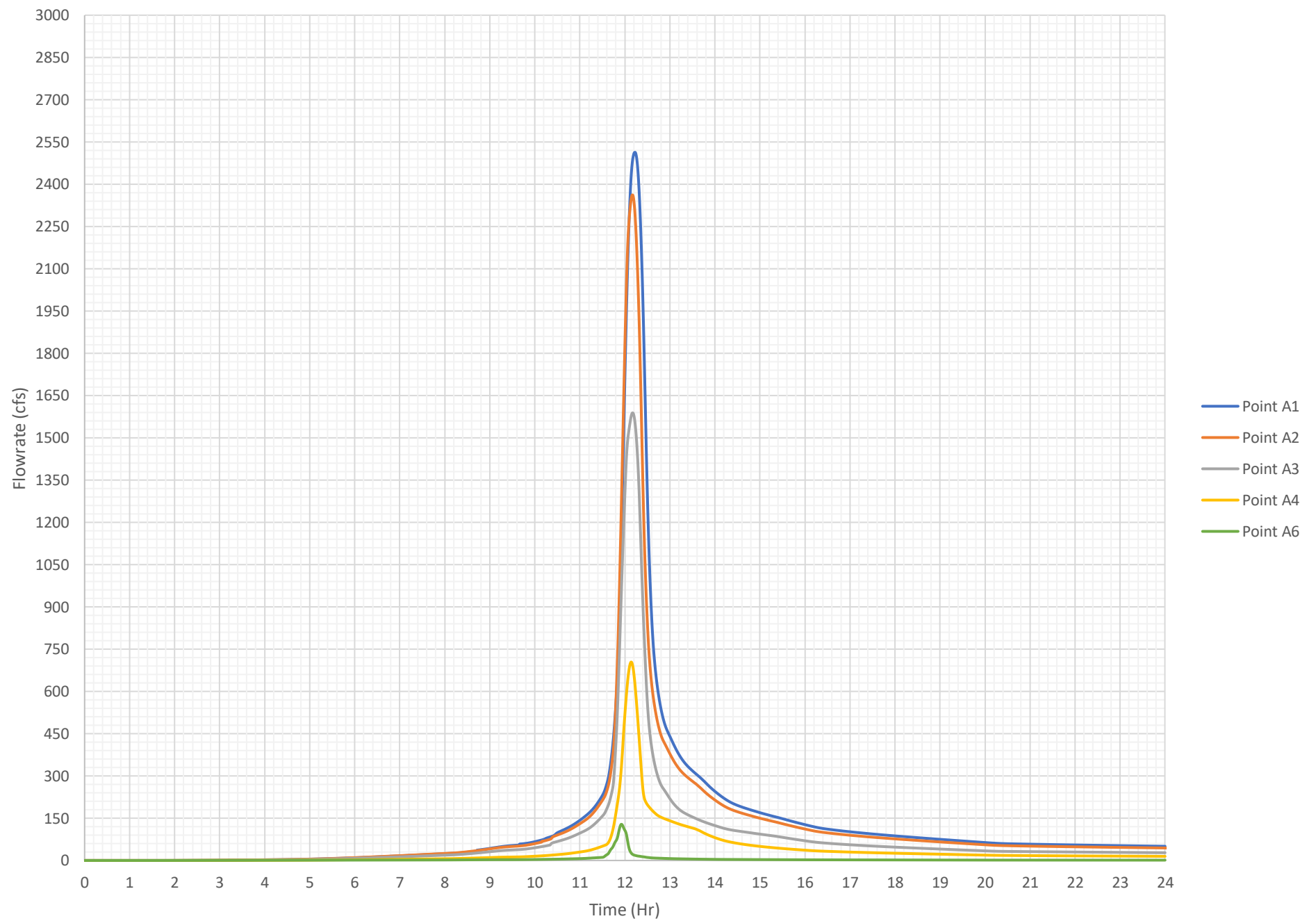
Proposed Peak 24-Hr 1% Flowrates (Macro)
