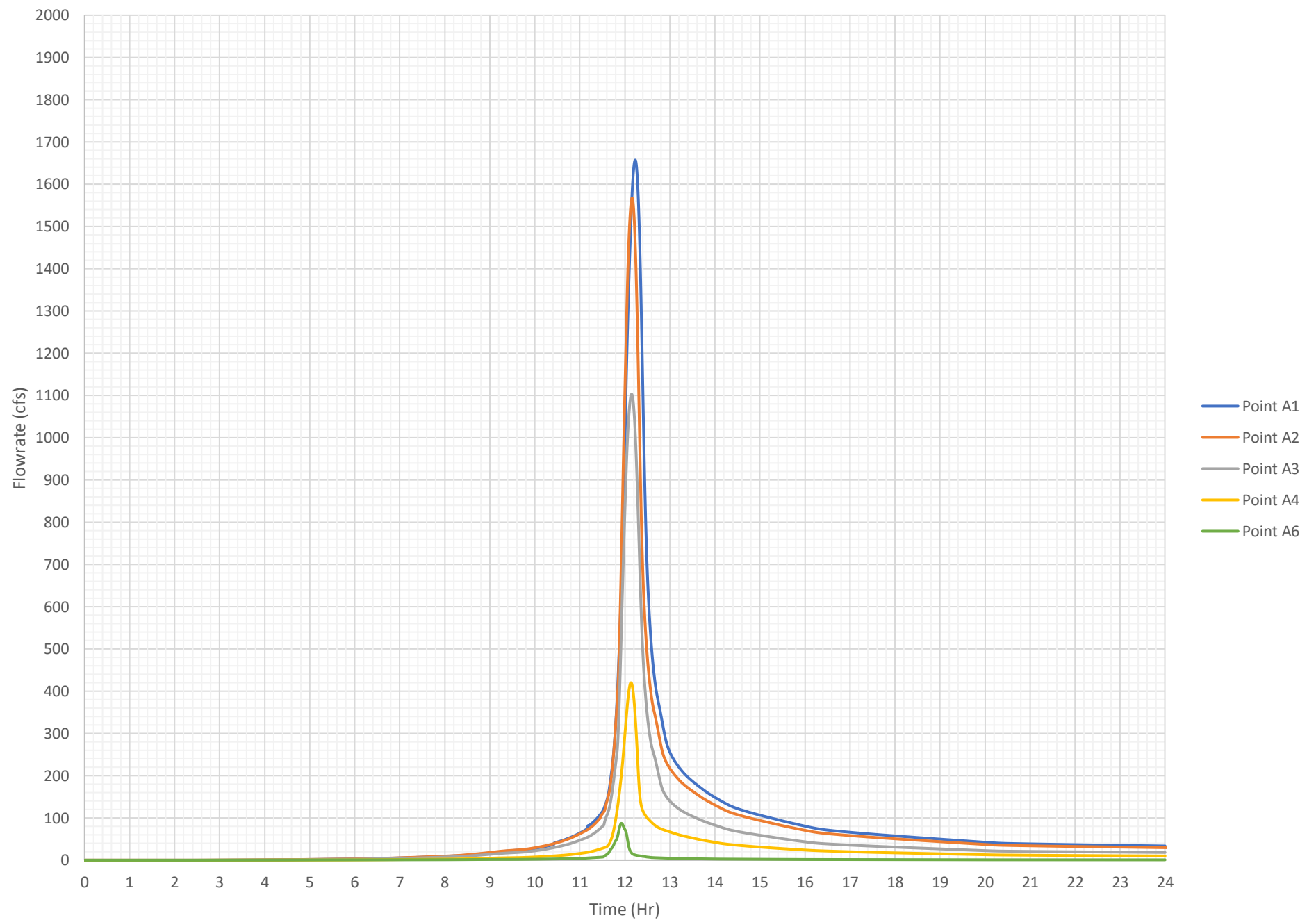
Proposed Peak 24-Hr 10% Flowrates (Macro)
