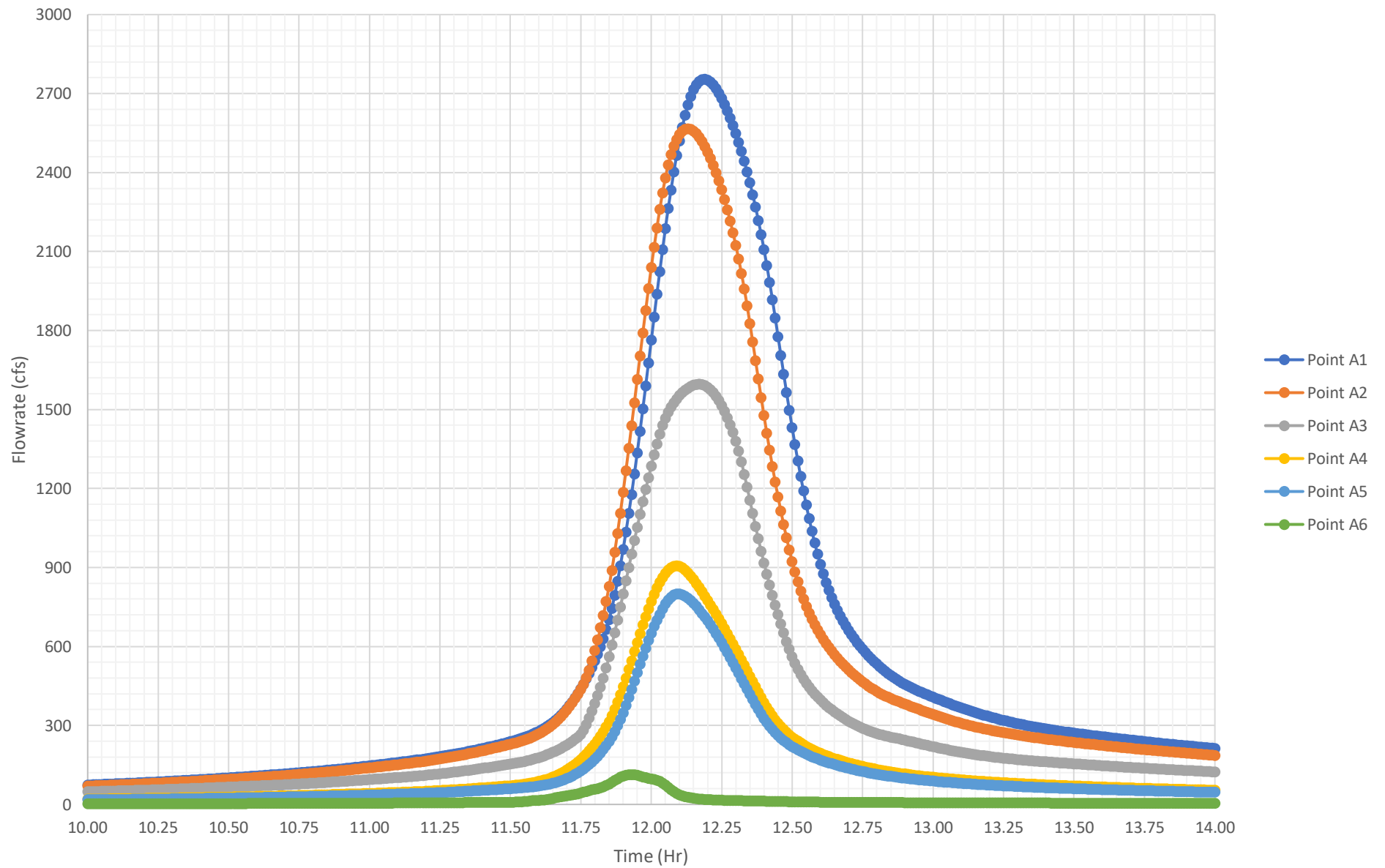
Existing Peak 4-Hr 1% Flowrates (Macro)
