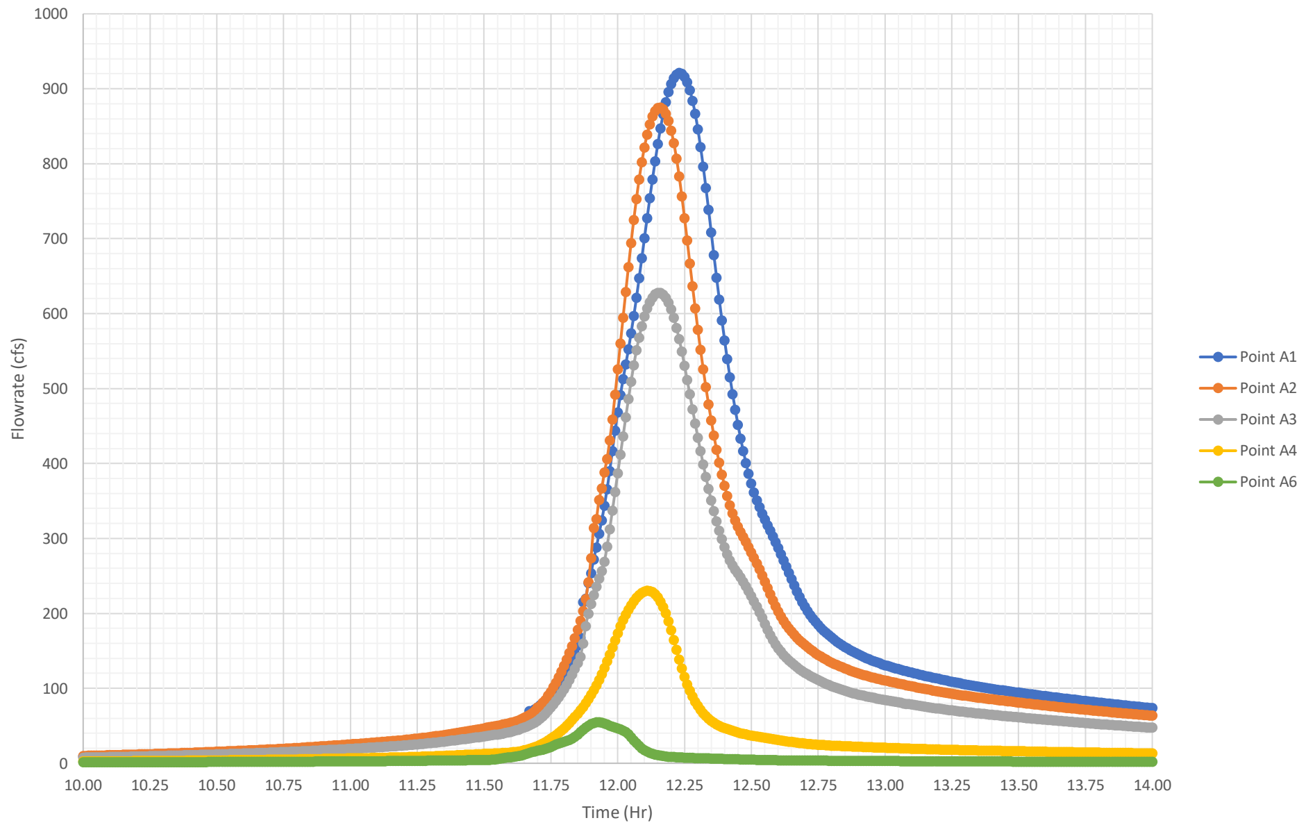
Proposed Peak 4-Hr 50% Flowrates (Macro)
