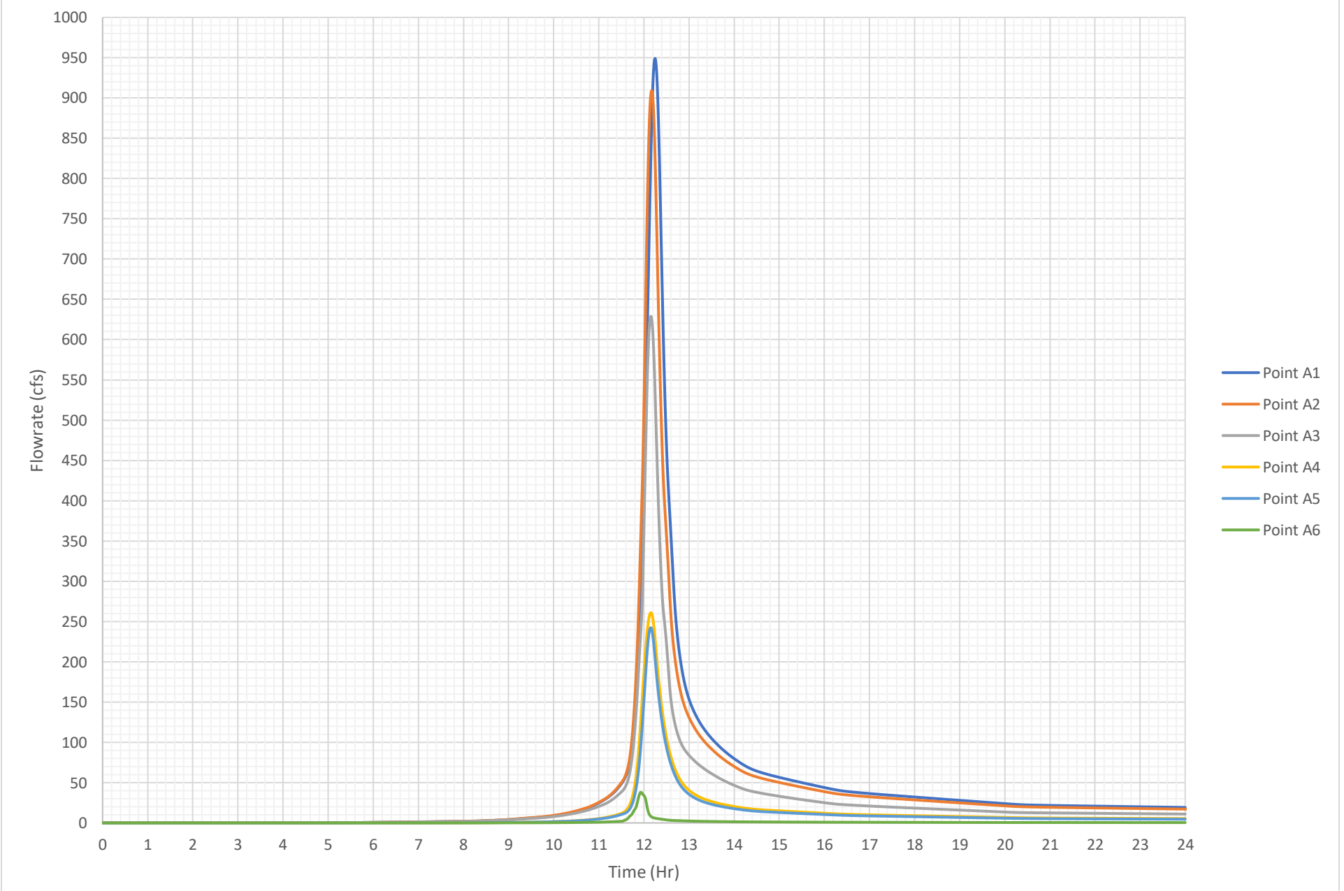
Existing Peak 24-Hr 50% Flowrates (Macro)
