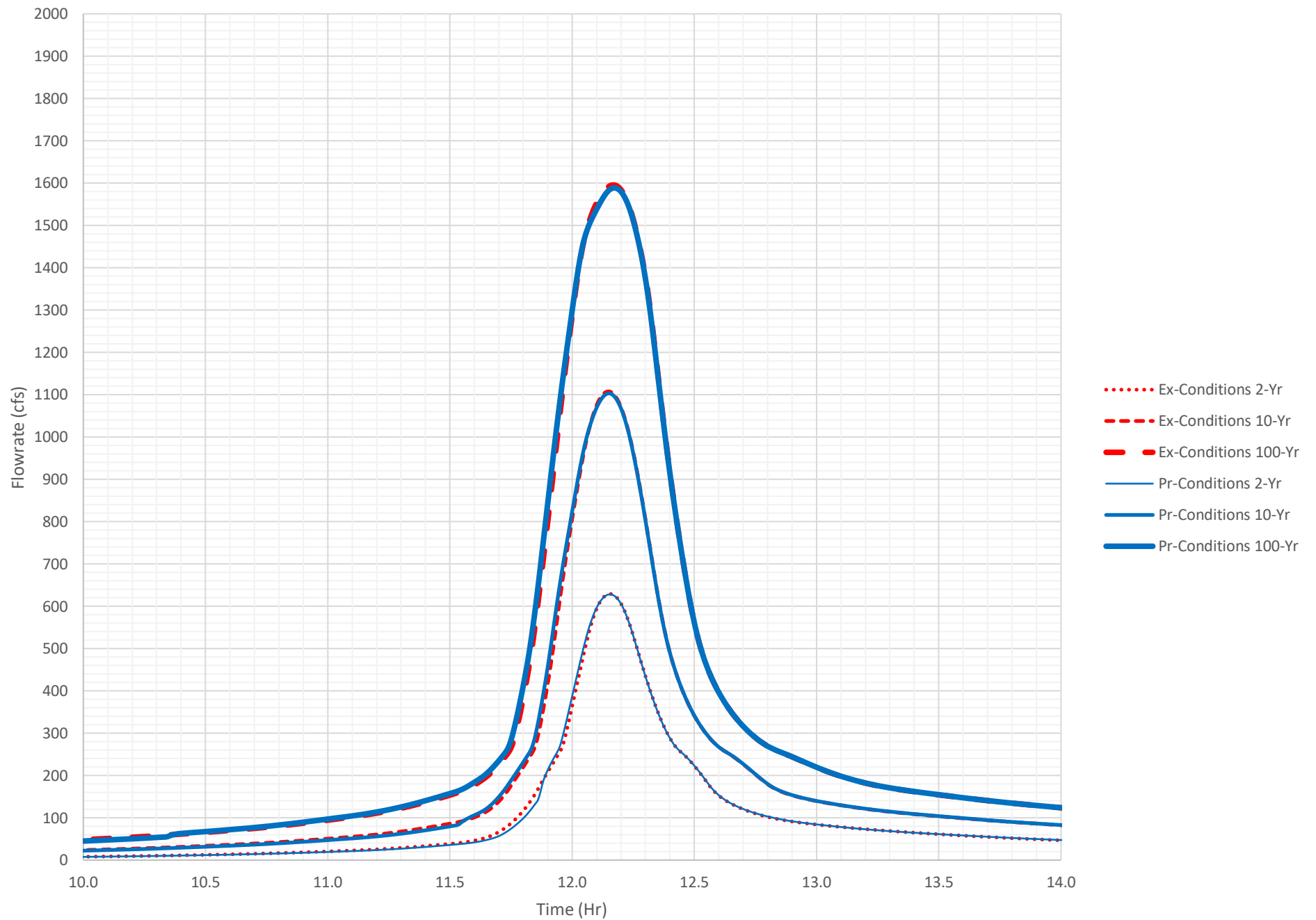
Existing & Proposed Conditions Point A3 Hydrograph(Fully-Developed)
