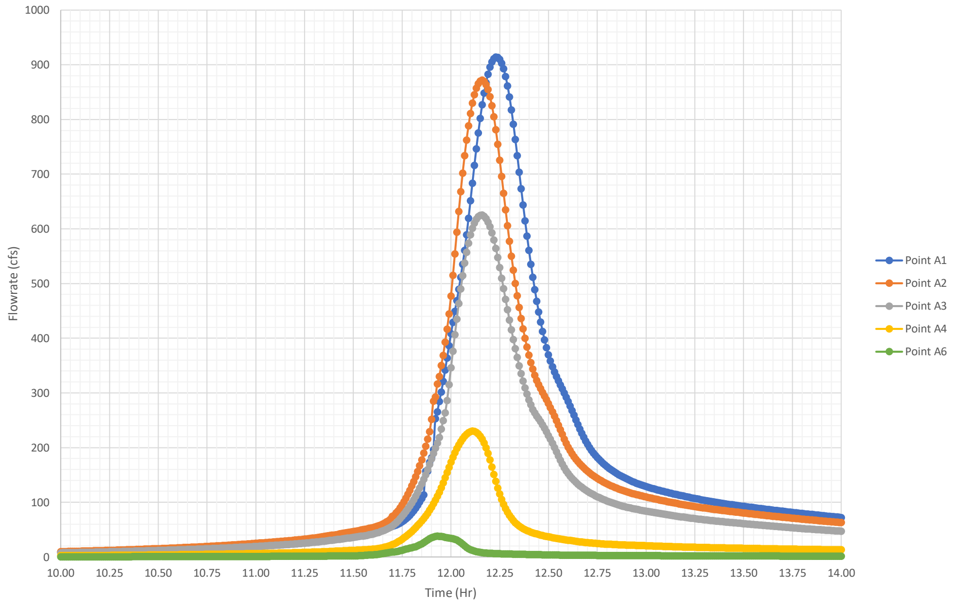
Proposed Peak 4-Hr 50% Flowrates (Micro)
