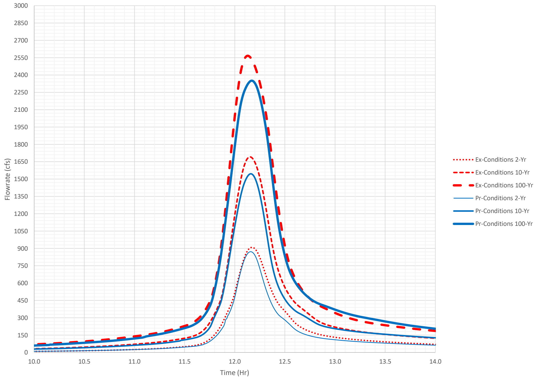
Existing & Proposed Conditions Point A2 Hydrograph(Micro)
