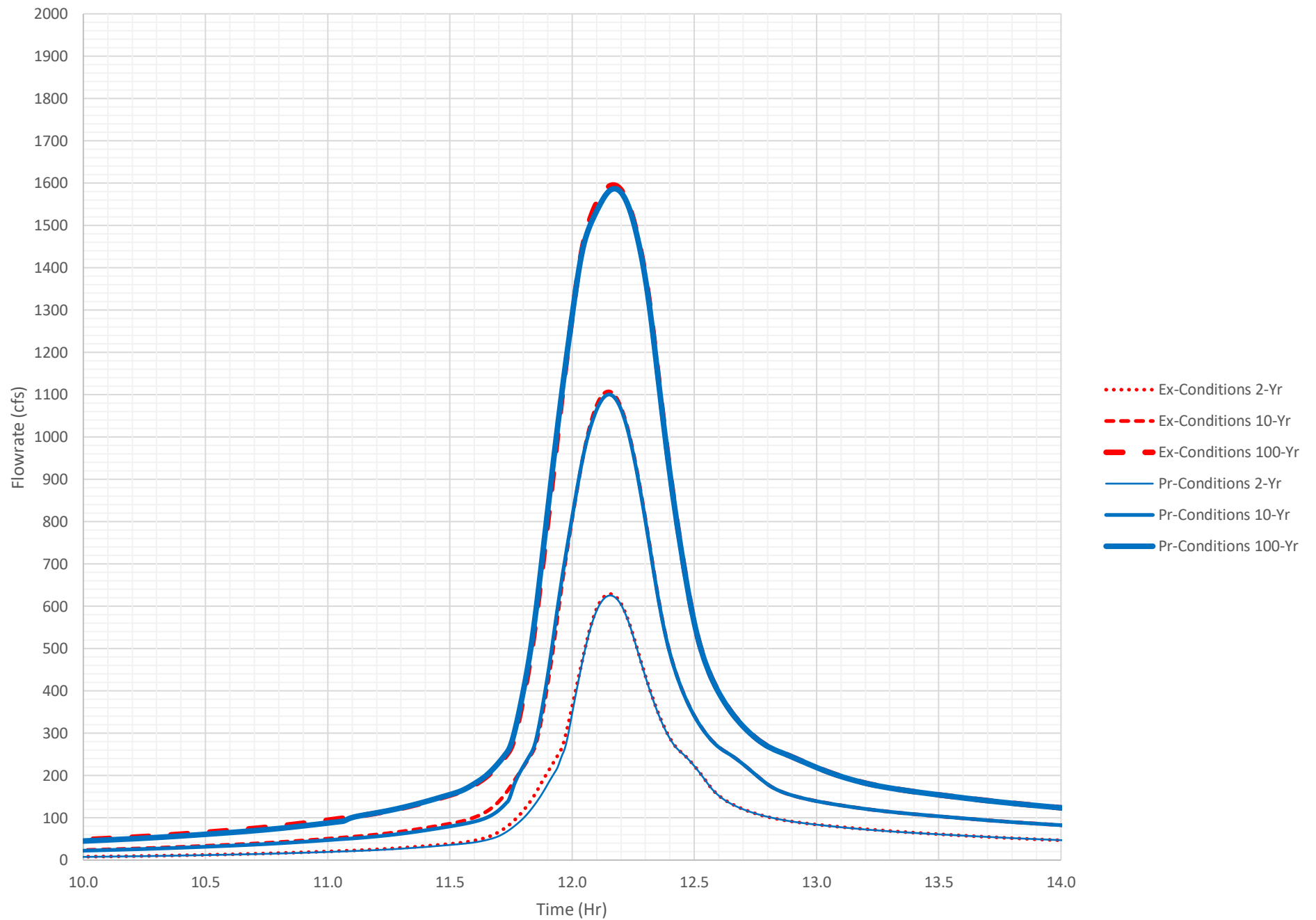
Existing & Proposed Conditions Point A3 Hydrograph(Micro)
