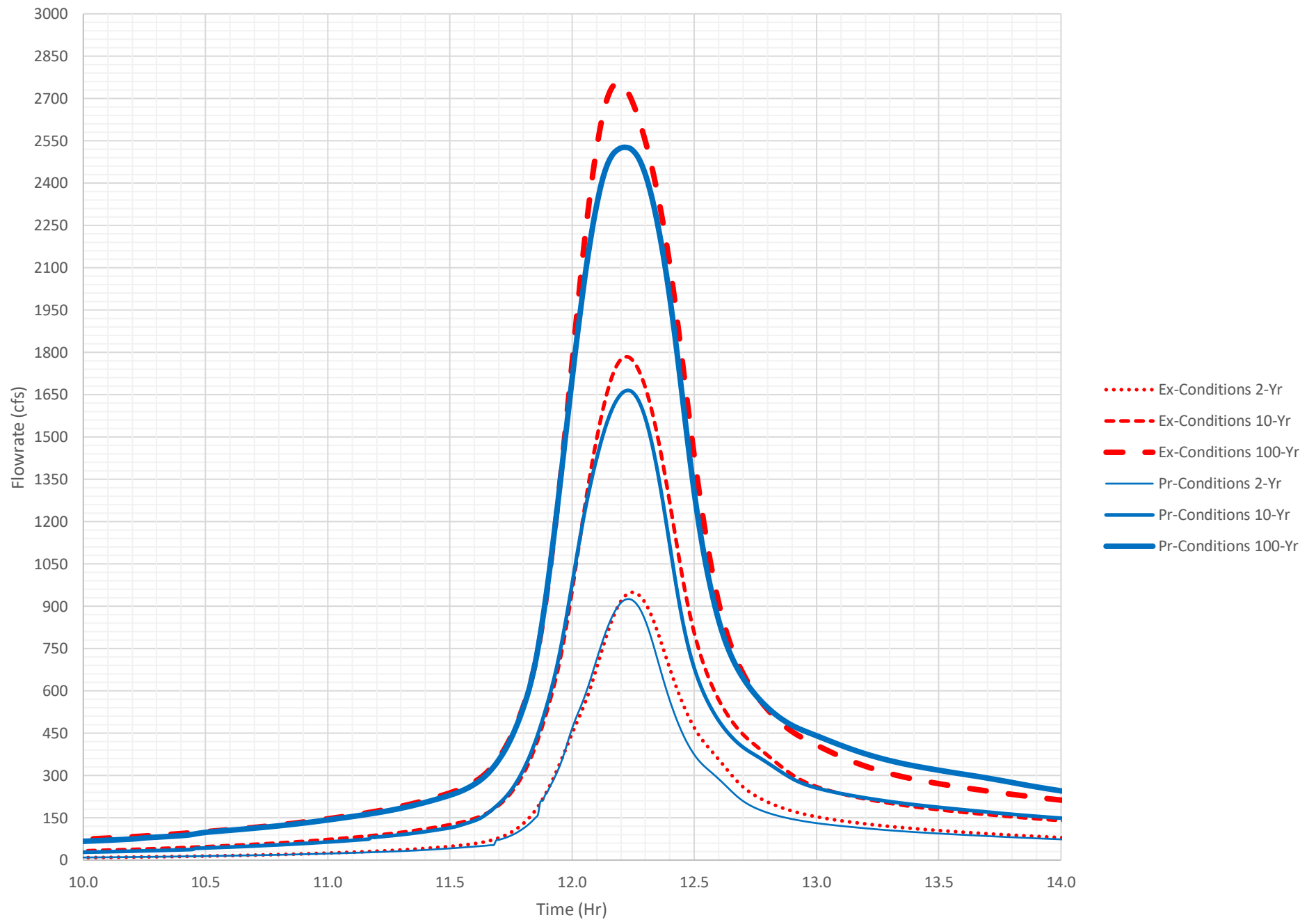
Existing & Proposed Conditions Point A1 Hydrograph(Fully-Developed)
