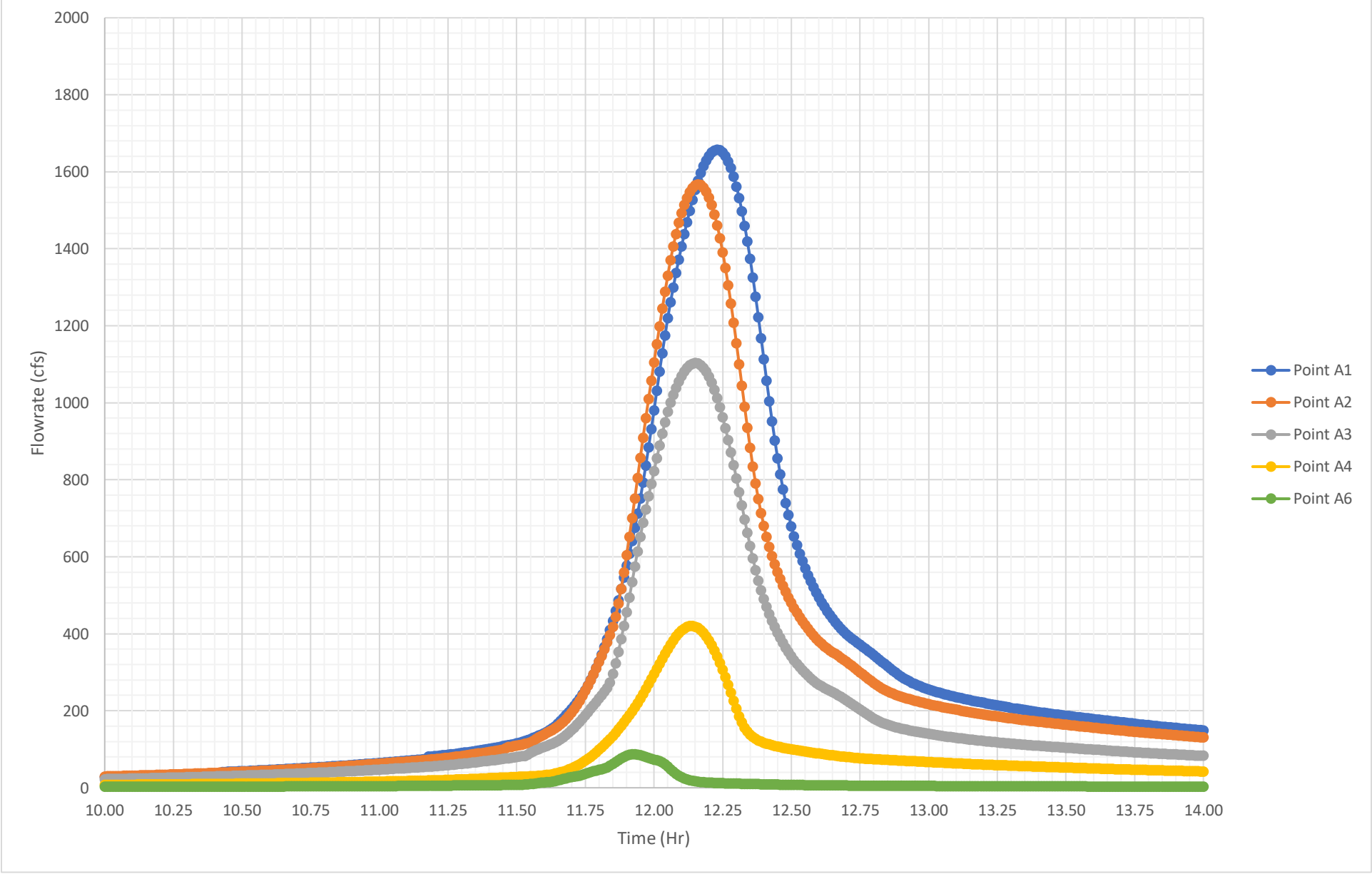
Proposed Peak 4-Hr 10% Flowrates (Macro)
