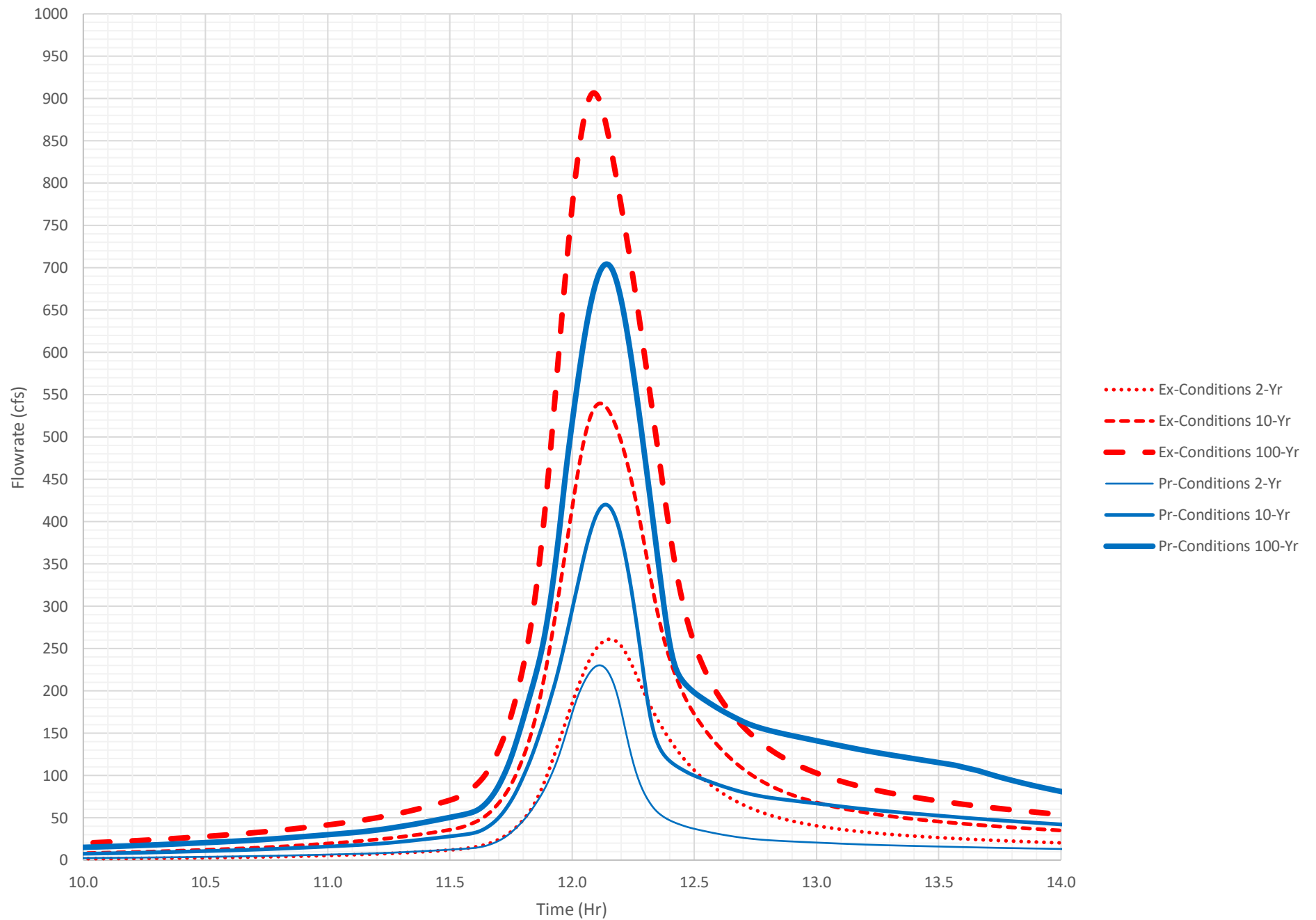
Existing & Proposed Conditions Point A4 Hydrograph(Fully-Developed)
