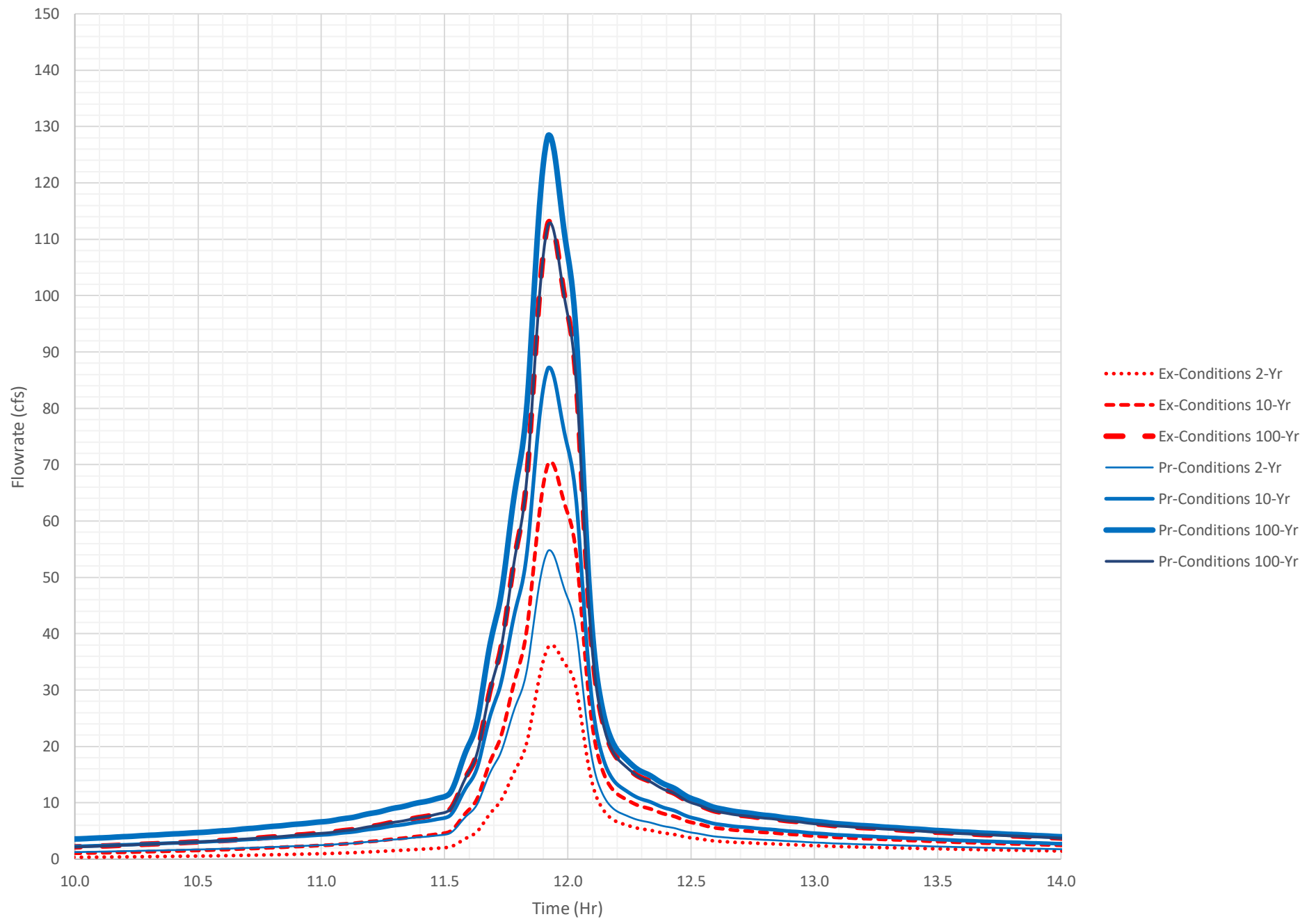
Existing & Proposed Conditions Point A6 Hydrograph(Fully Developed)
