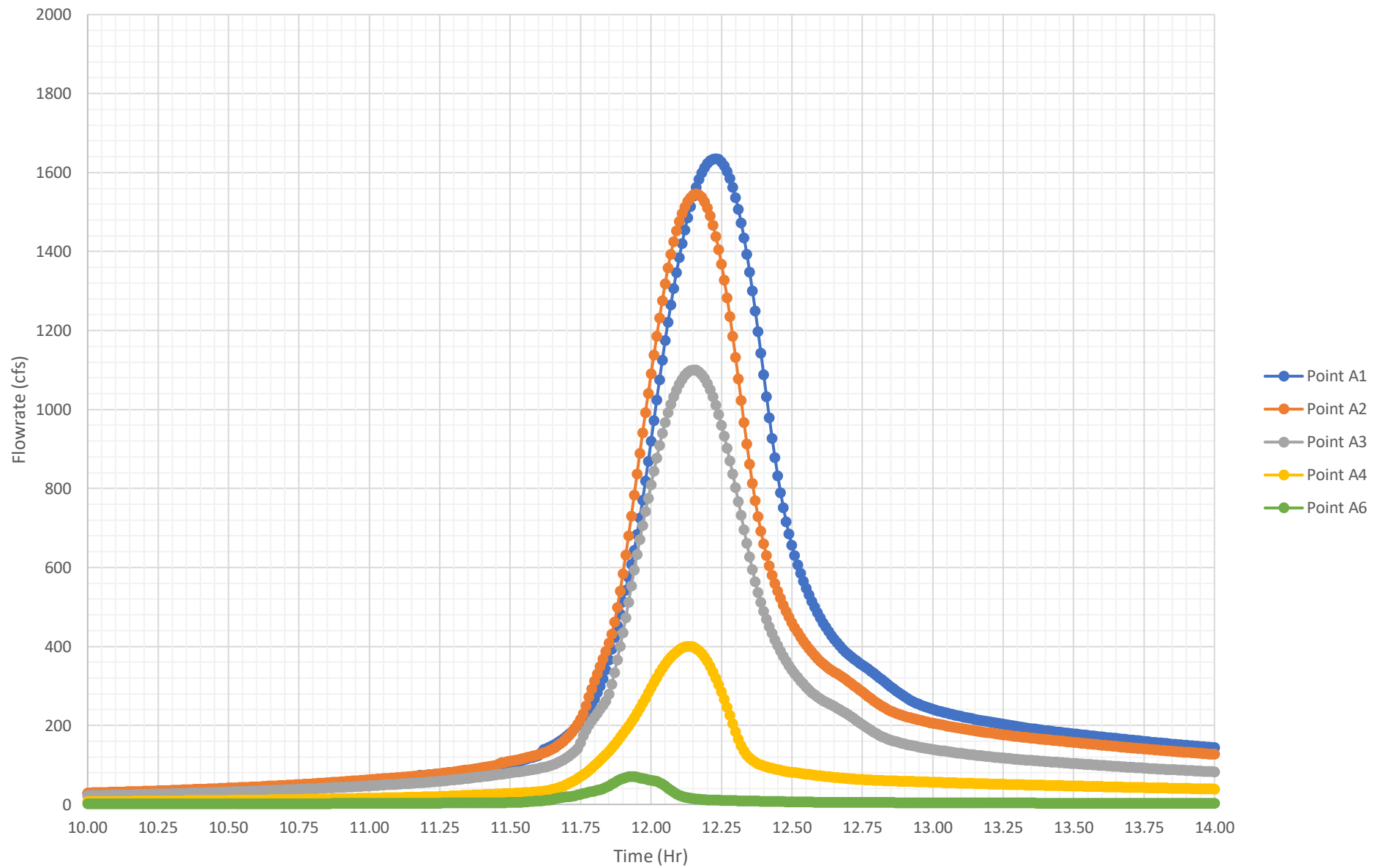
Proposed Peak 4-Hr 10% Flowrates (Micro)
