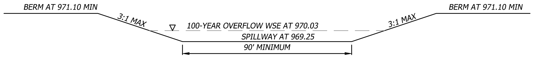
SPILLWAY CROSS-SECTION A-A
