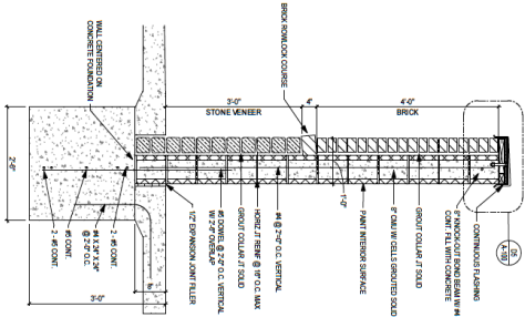
A4 TRASH ENCLOSURE WALL SECTION SCALE: 3/4\"/>
