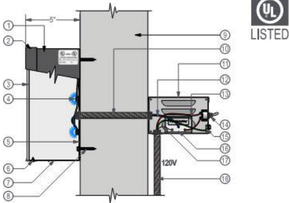
FIGURE 3 - FACE LIT CHANNEL LETTERS WITH LED ILLUMINATION DETAIL
