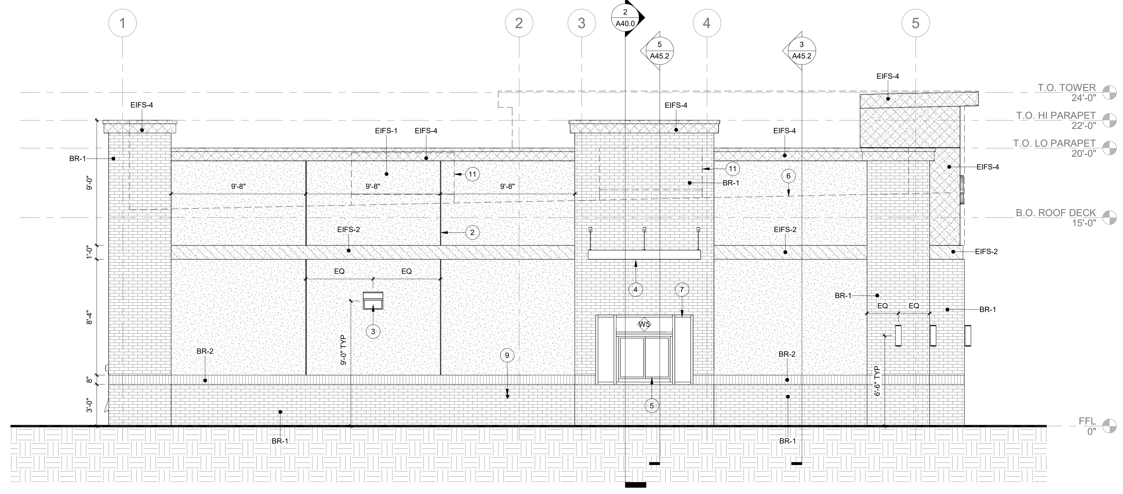
② WEST ELEVATION 1/4" = 1'-0"
