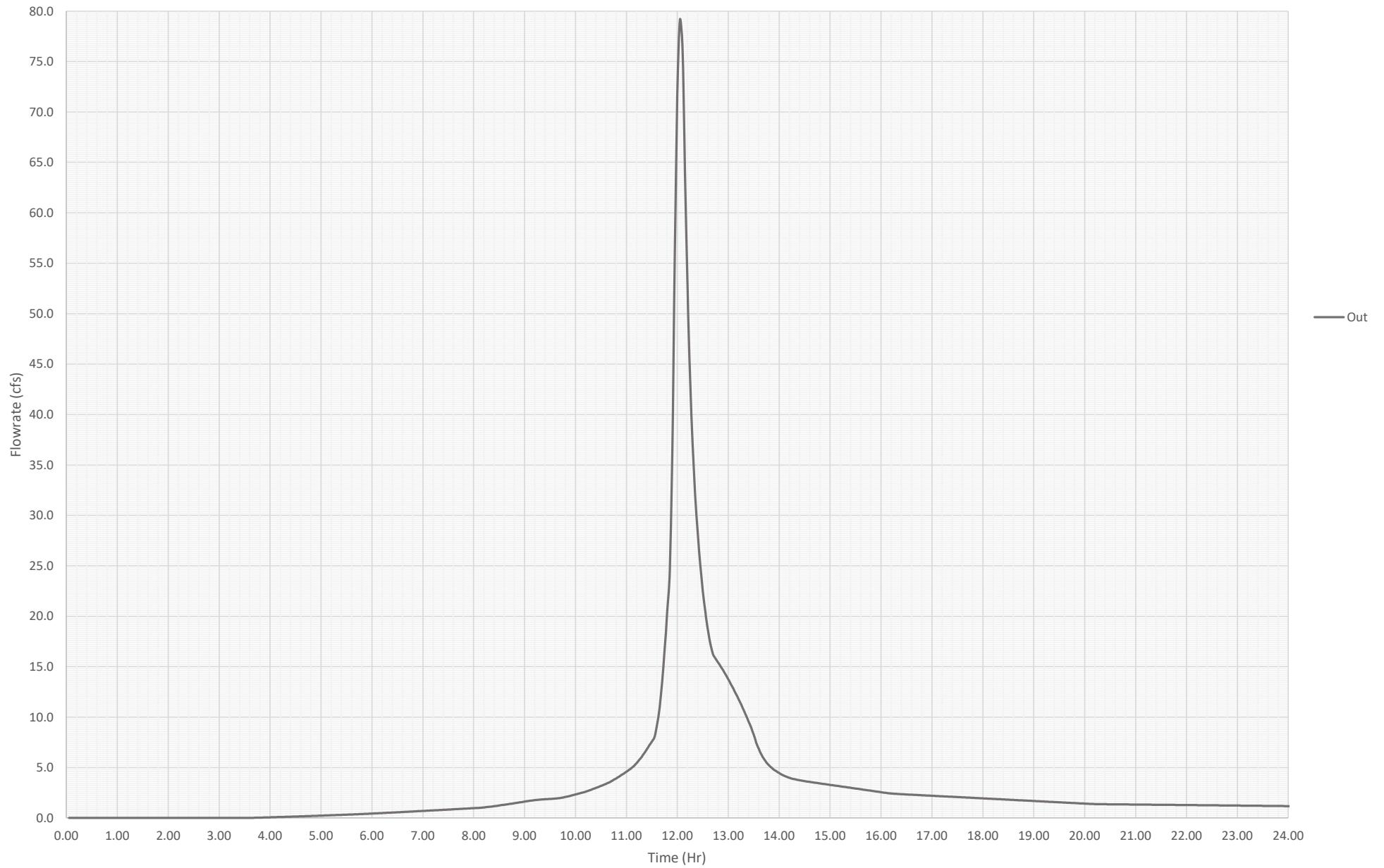
100 Year Event - Proposed Peak 24-Hr Flowrate
