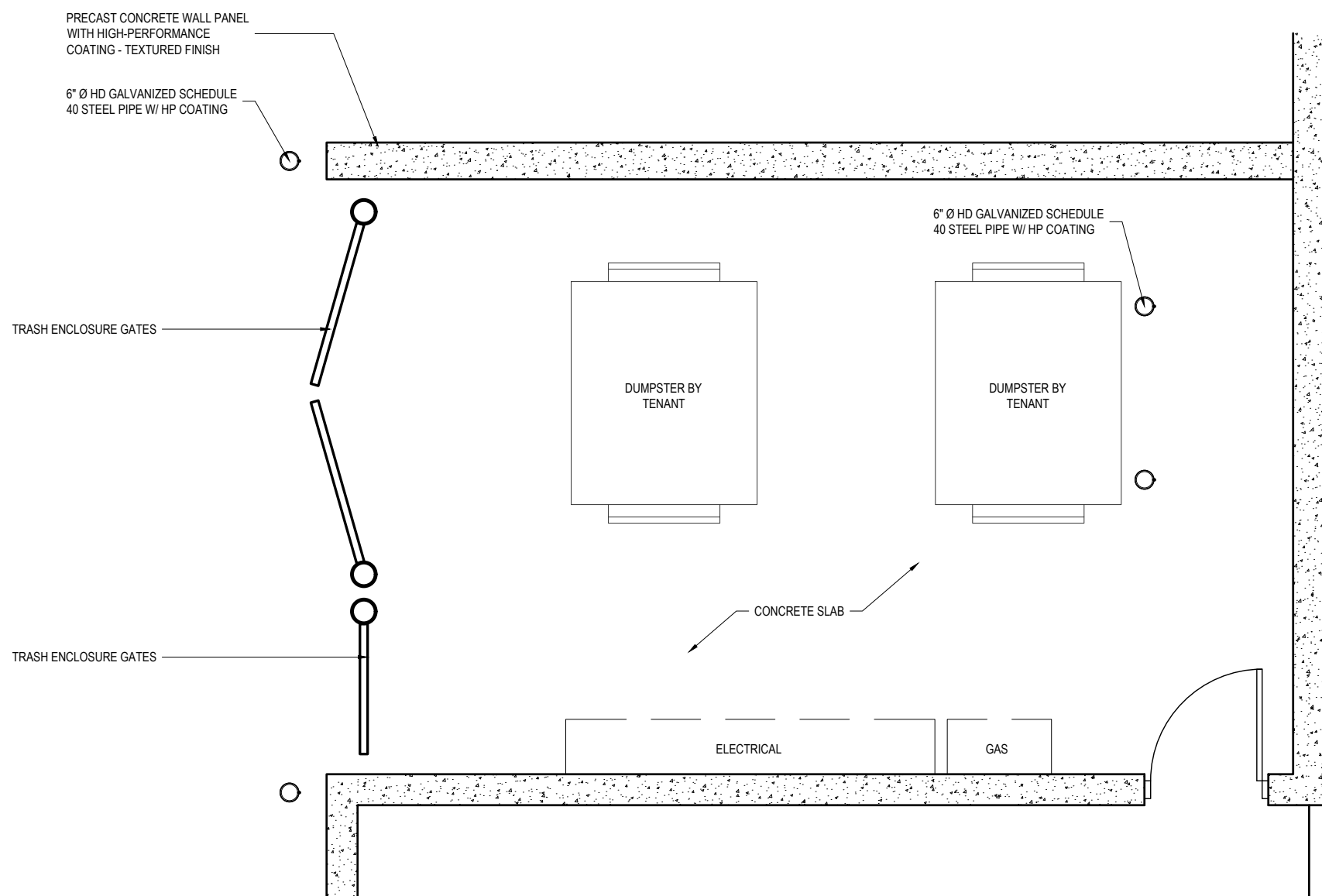
Enlarged Trash Enclosure Details 1/2" = 1'-0"
