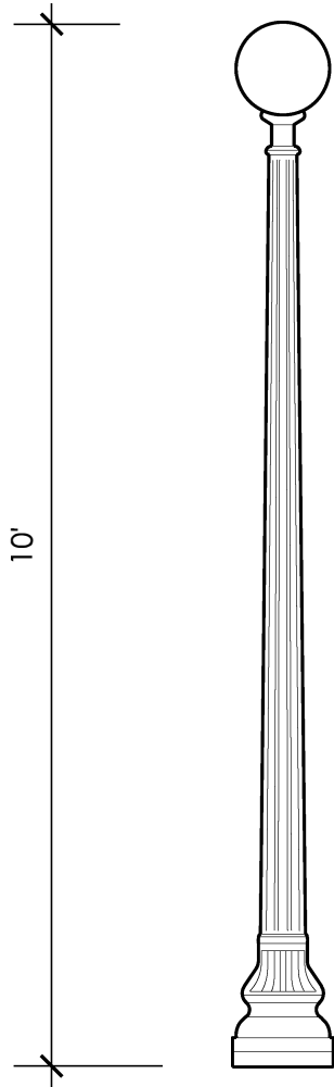
TUSCUMBIA METAL WORKS ST. CHARLES LIGHT A-1840 [TALL] 10' DARK BRONZE
