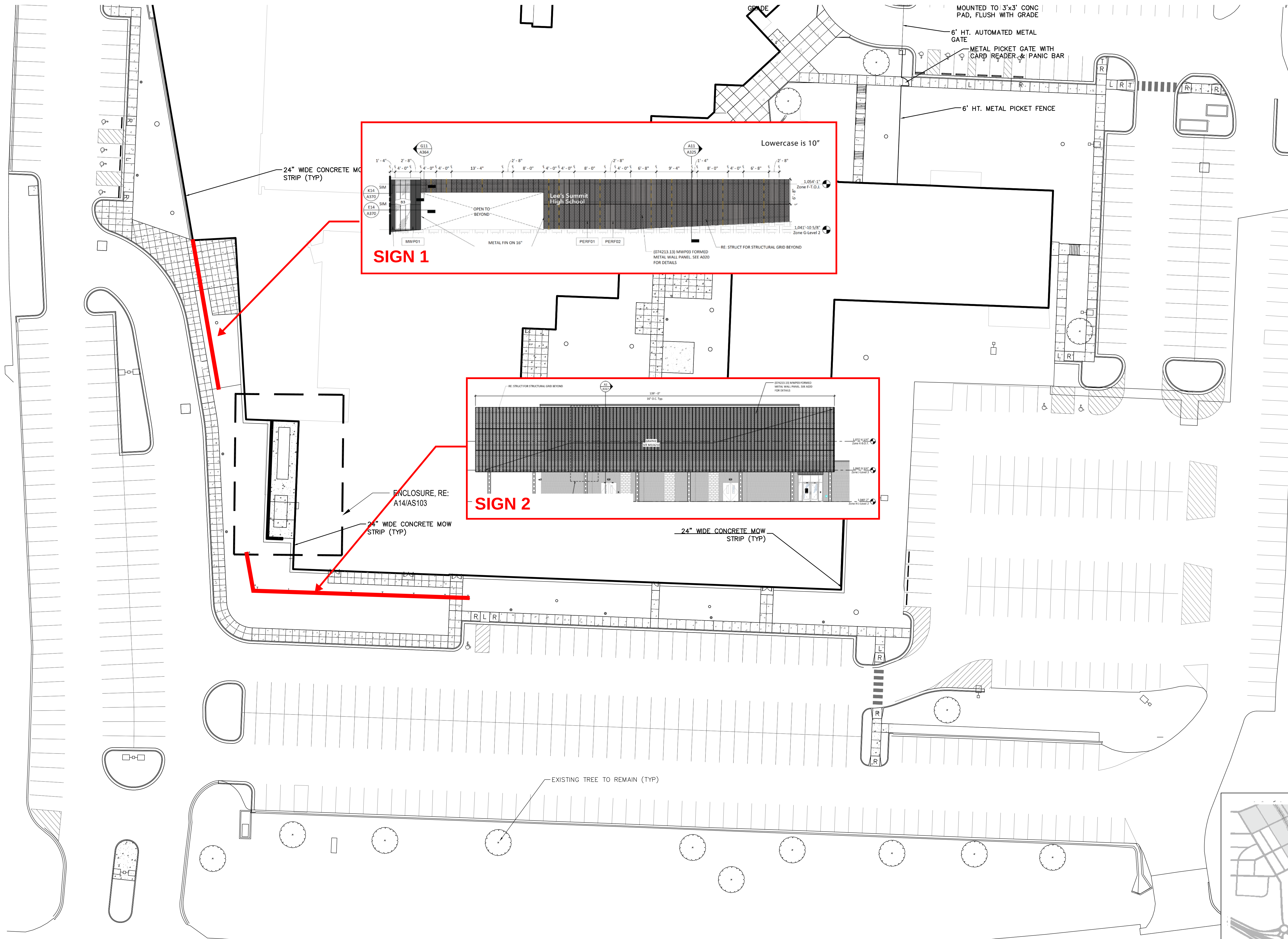
Architectural Site Plan (south site)
