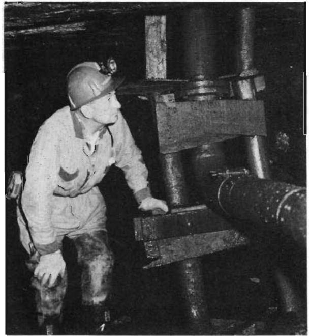
Fig. 5. Elbow at the foot of a controlled flushing borehole.
