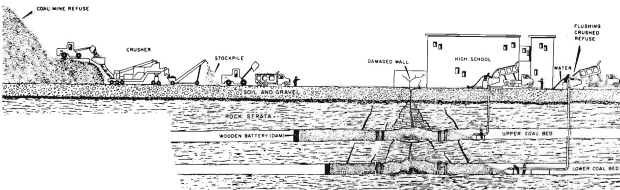
Fig. 3. A typical controlled backfilling project.
