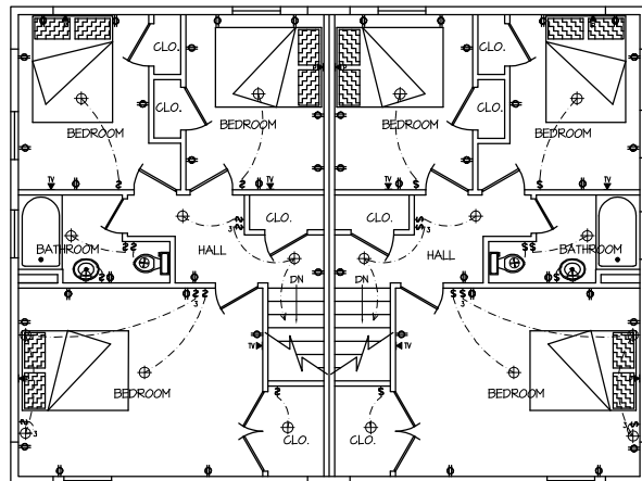
Upper Floor Electrical Plan
