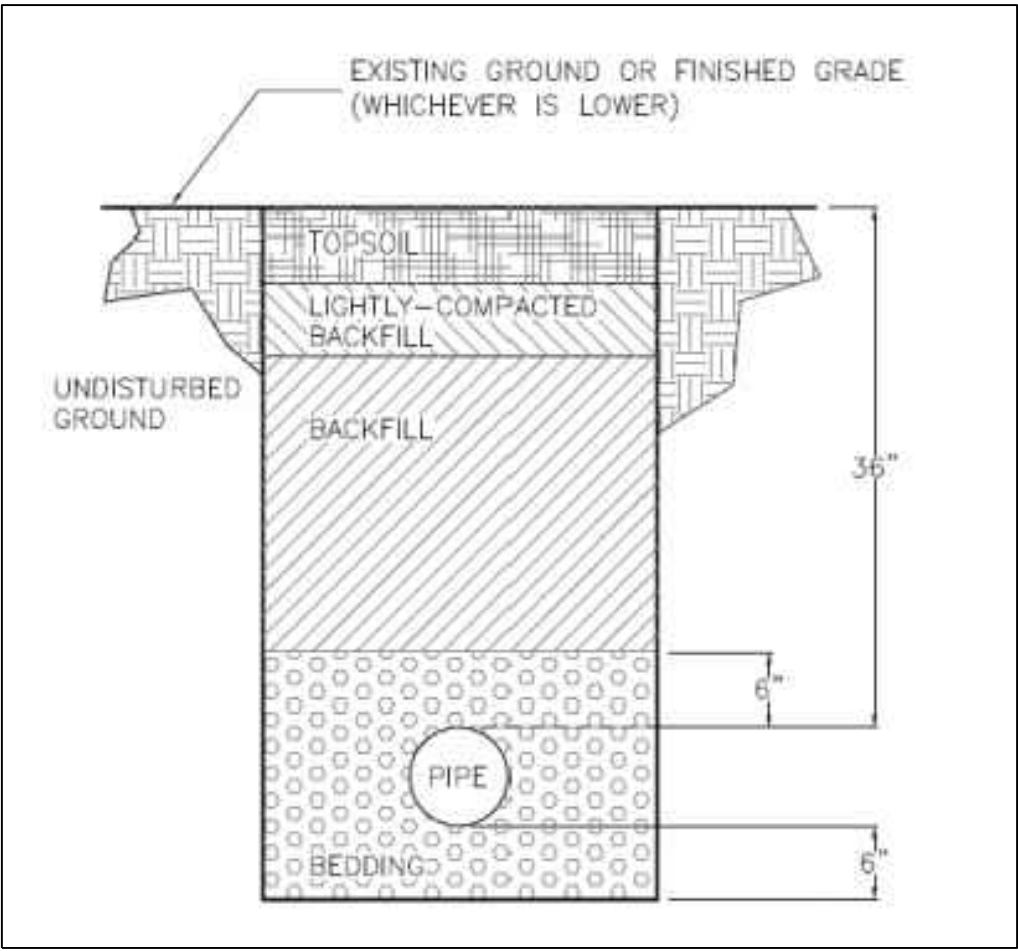
TRENCH AND BACKFILL DETAIL
