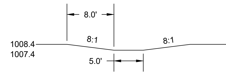
SWALE 3 NOT TO SCALE
