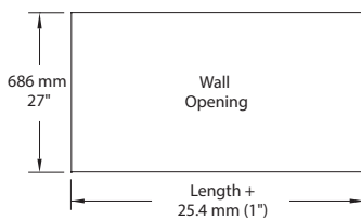
Installation with Recess Trim Kit
