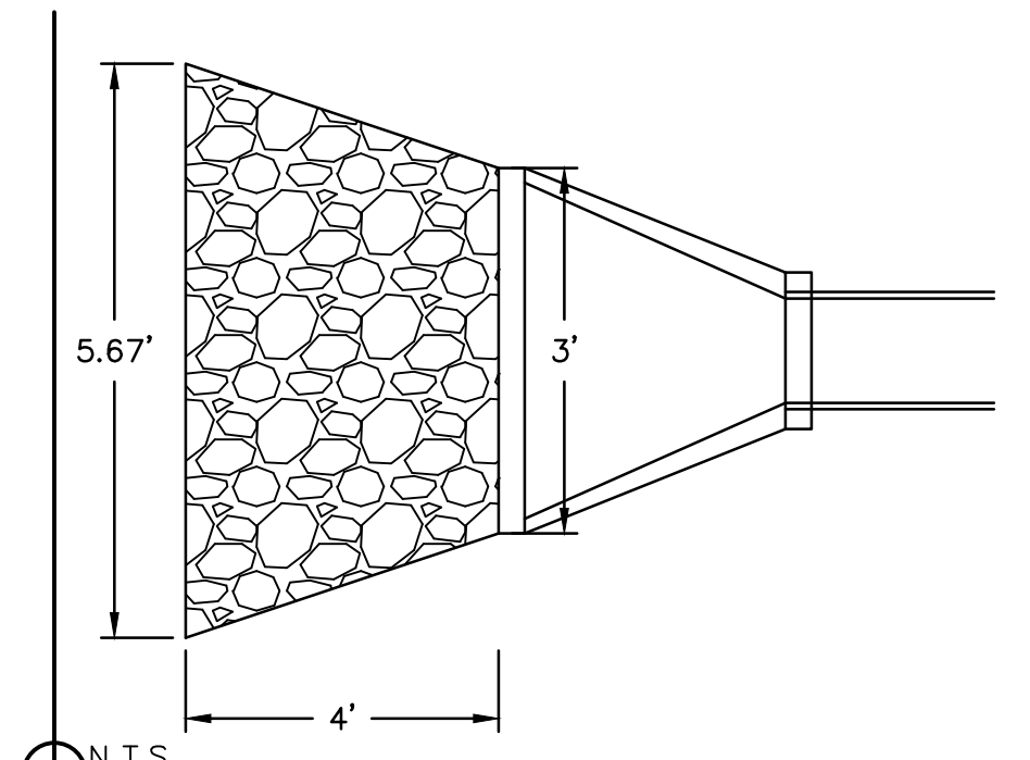
02 RIPRAP OULET PROTECTION
