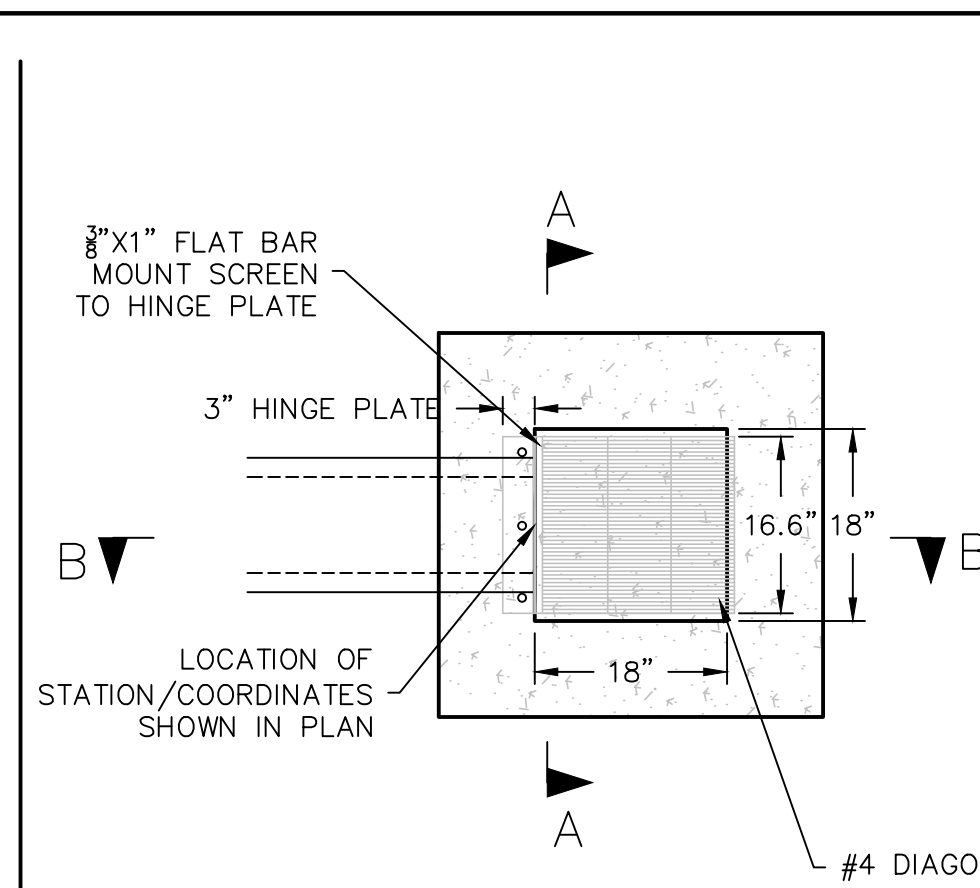
01 WATER QUALITY BASIN OULET STRUCTURE
