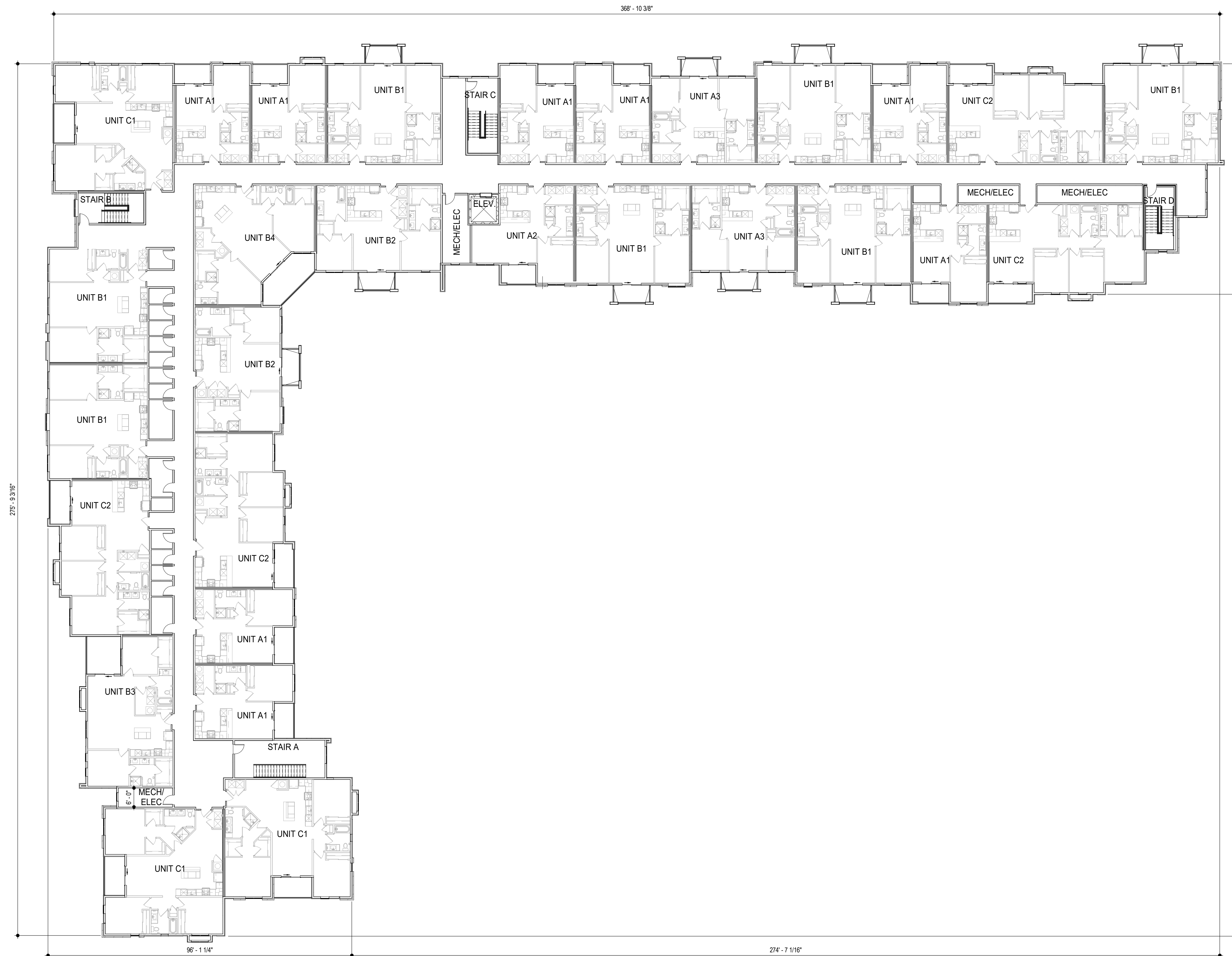
1 BLDG 2 - THIRD FLOOR PLAN SCALE: 1/16" = 1'-0"
