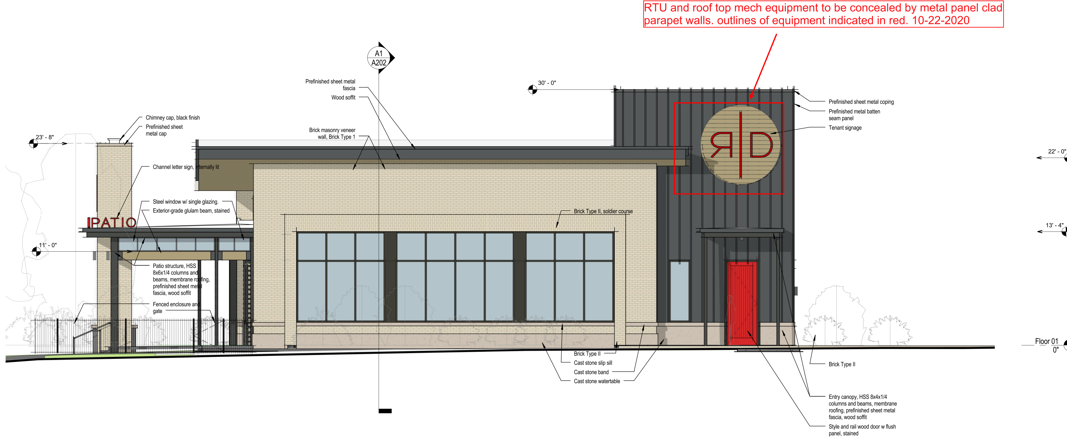
E4 3/16" = 1'-0"
