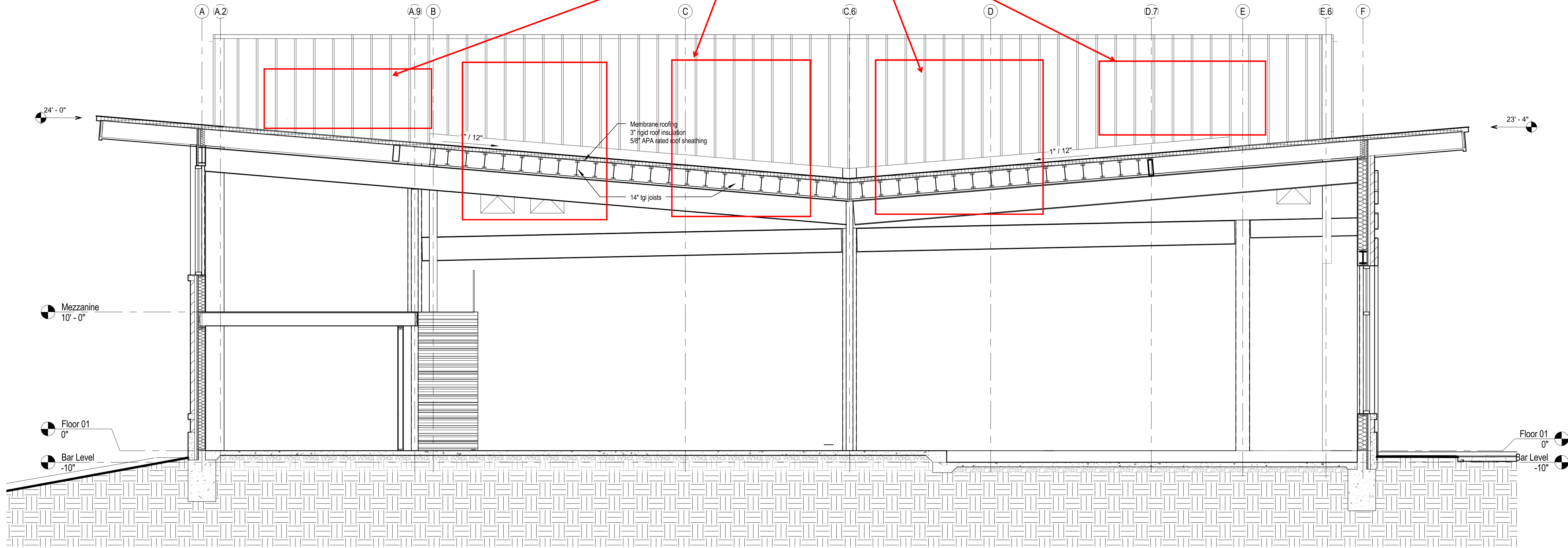
A1 1/4" = 1'-0" Building Section
