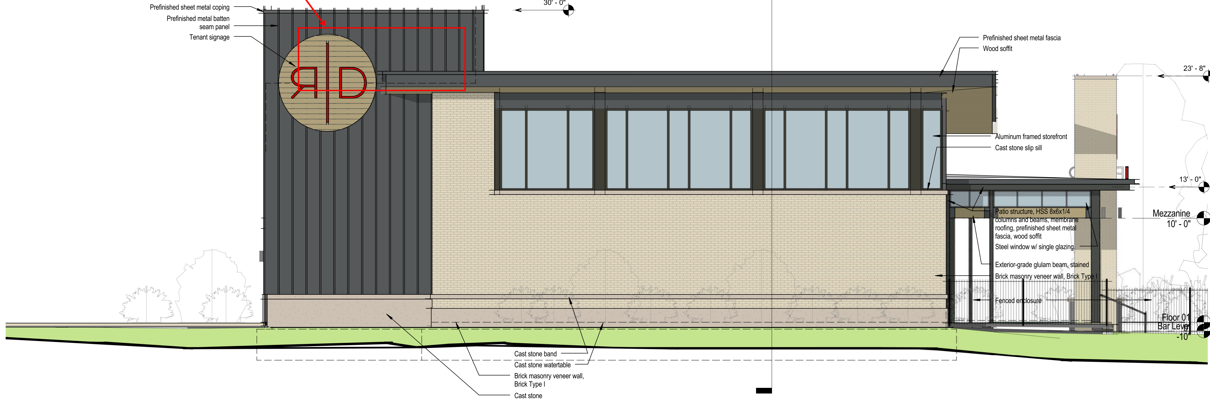
E4 3/16" = 1'-0" Elevation 3
