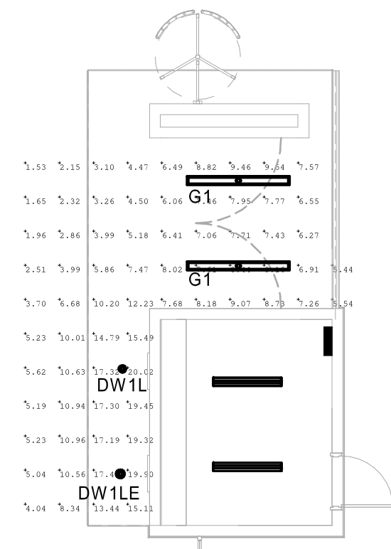
② SITE PHOTOMETRIC PLAN - SOUTH TICKET BOOTH 1/8" = 1'-0"
