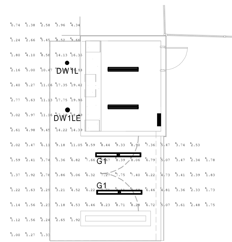
① SITE PHOTOMETRIC PLAN - NORTH TICKET BOOTH 1/8" = 1'-0"
