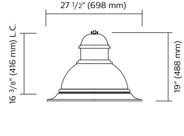
DMS50 - F optics Flat lens
