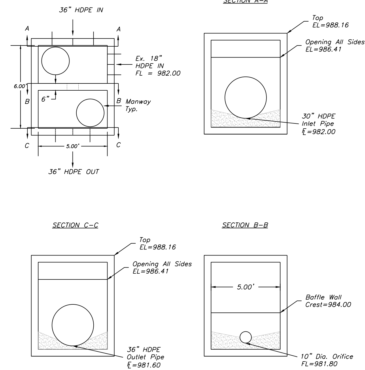
CONTROL STRUCTURE -- BASIN E 1/4" = 1'-0"
