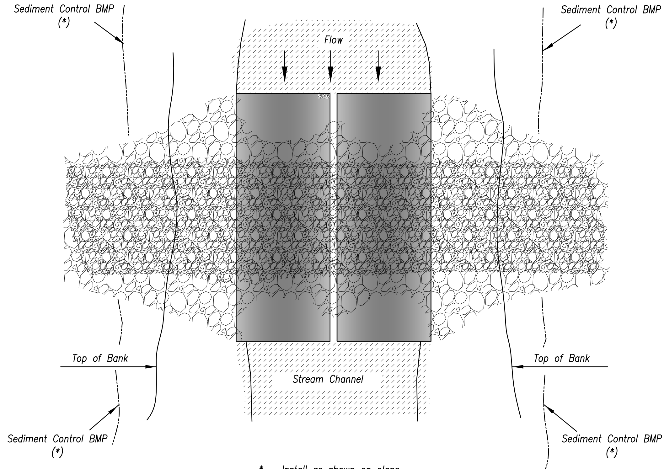
PLAN VIEW
