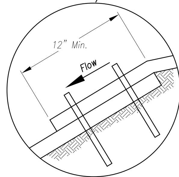
Splice Seam
