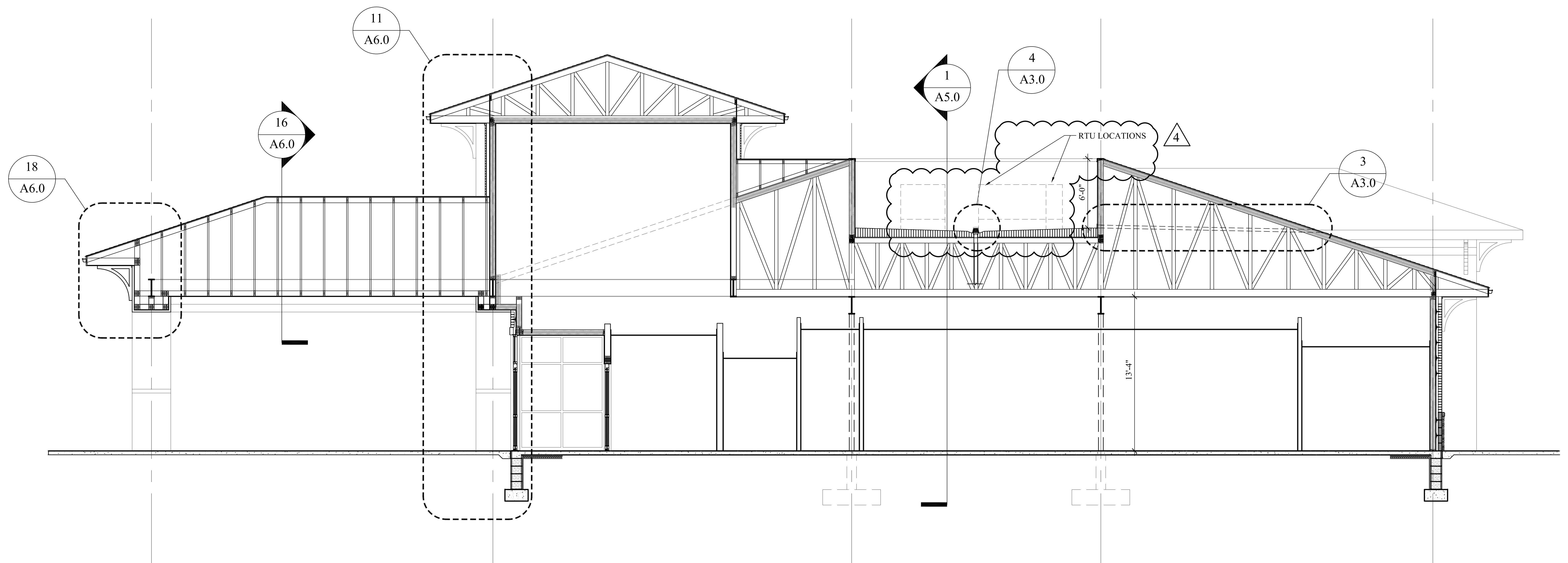
BUILDING SECTION AT ENTRANCE
