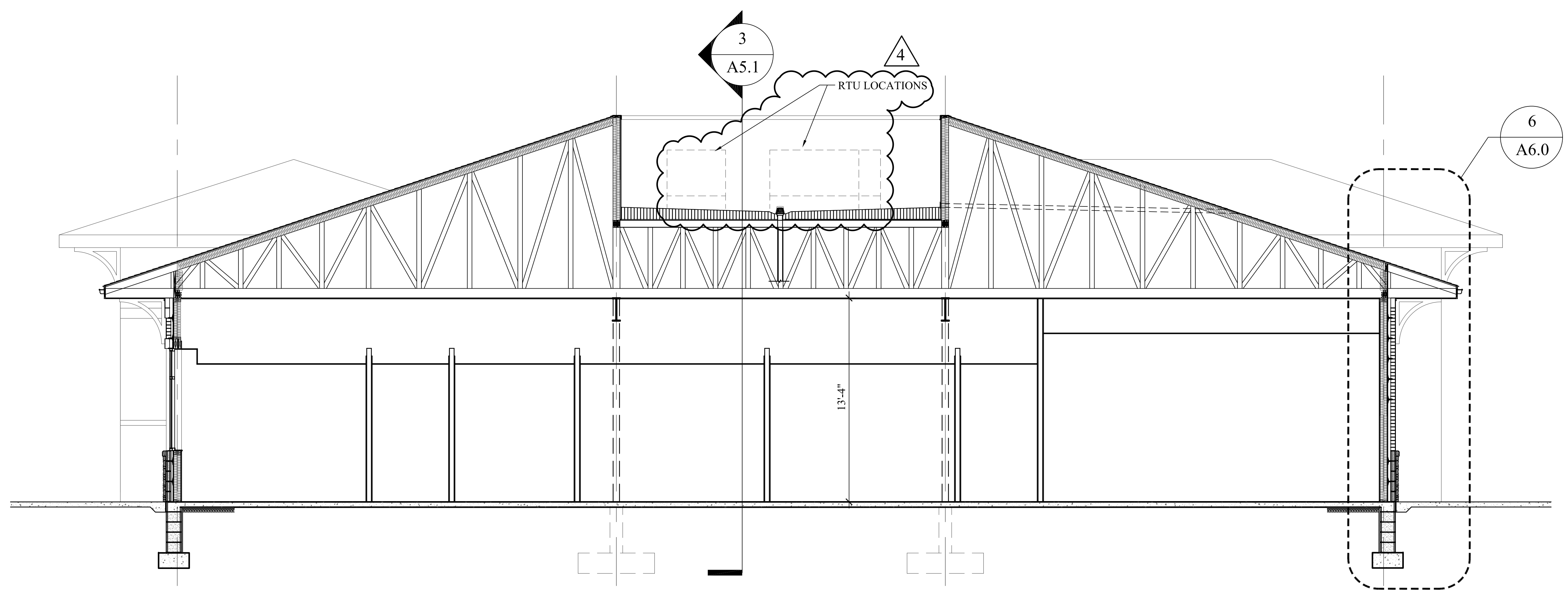
BUILDING SECTION AT ENTRANCE
