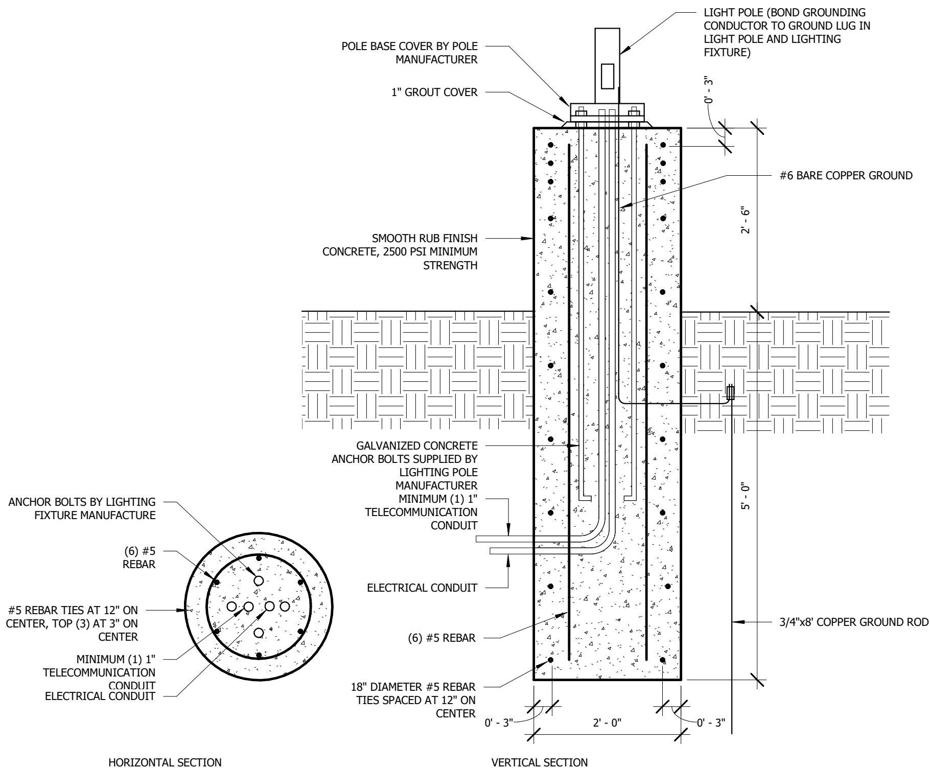
2 PARKING LOT LIGHT POLE BASE NOT TO SCALE
