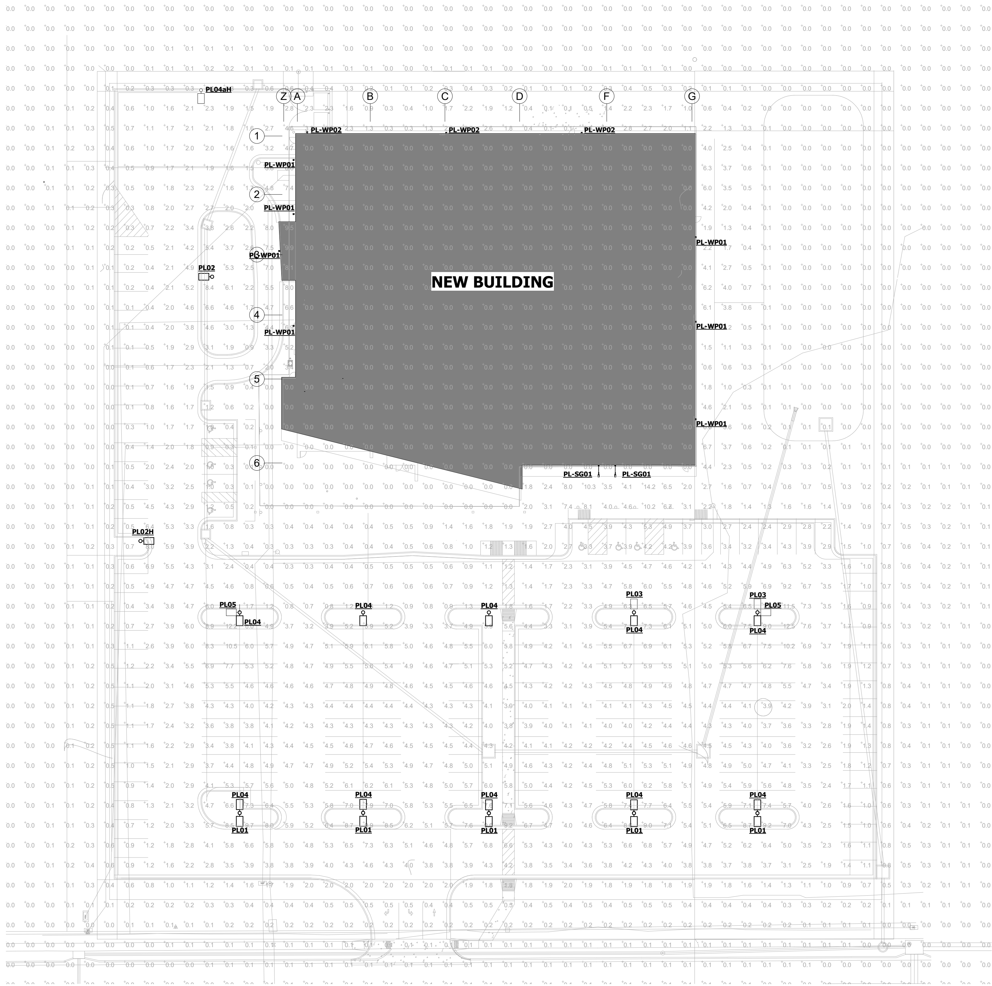
1 SITE PHOTOMETRIC PLAN 1" = 30'-0"
