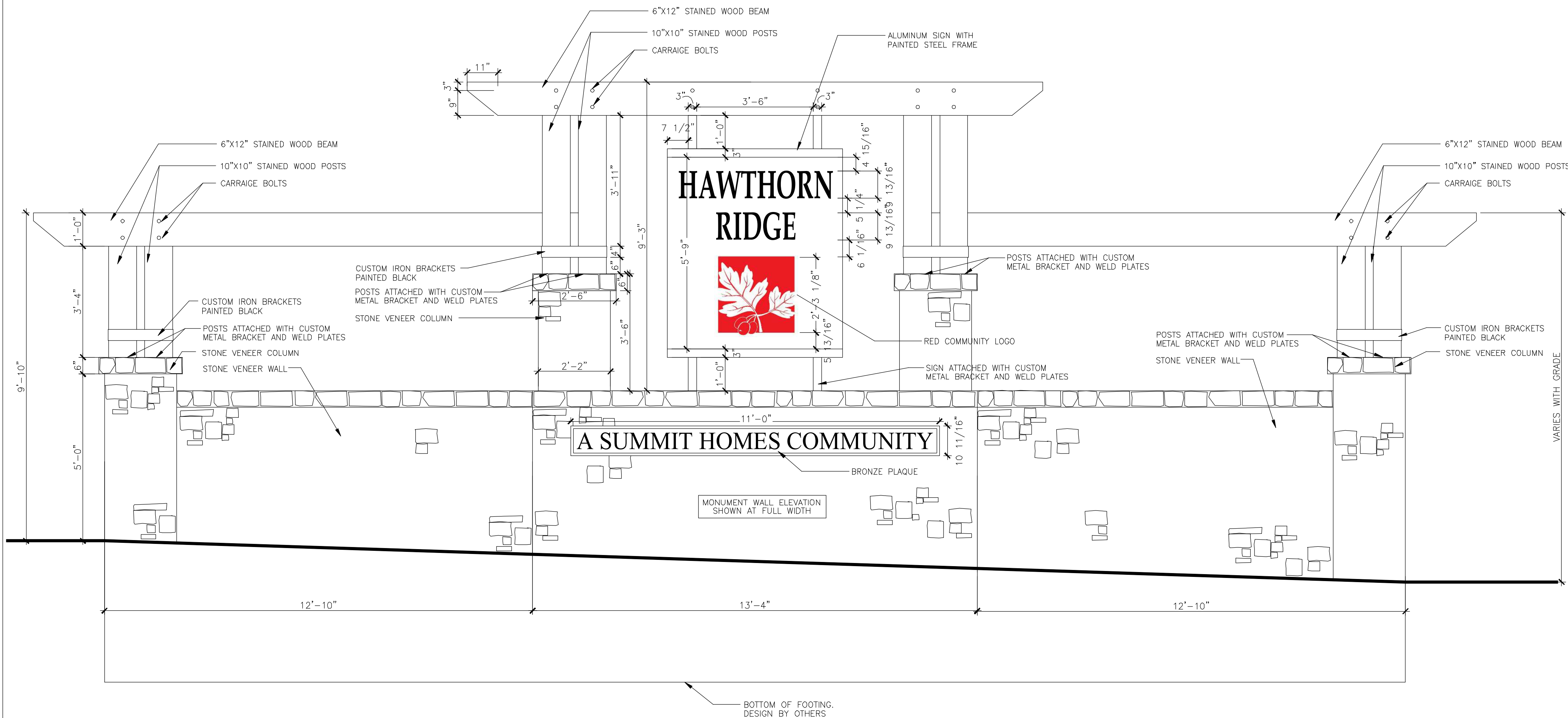
2 MONUMENT ELEVATION
