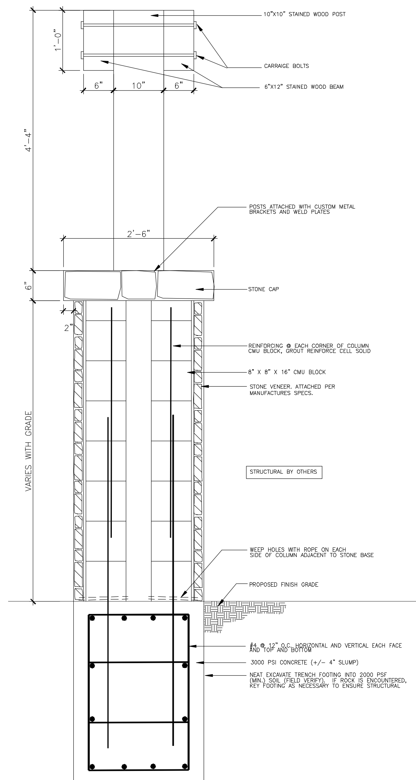
4 MONUMENT- SECTION A
