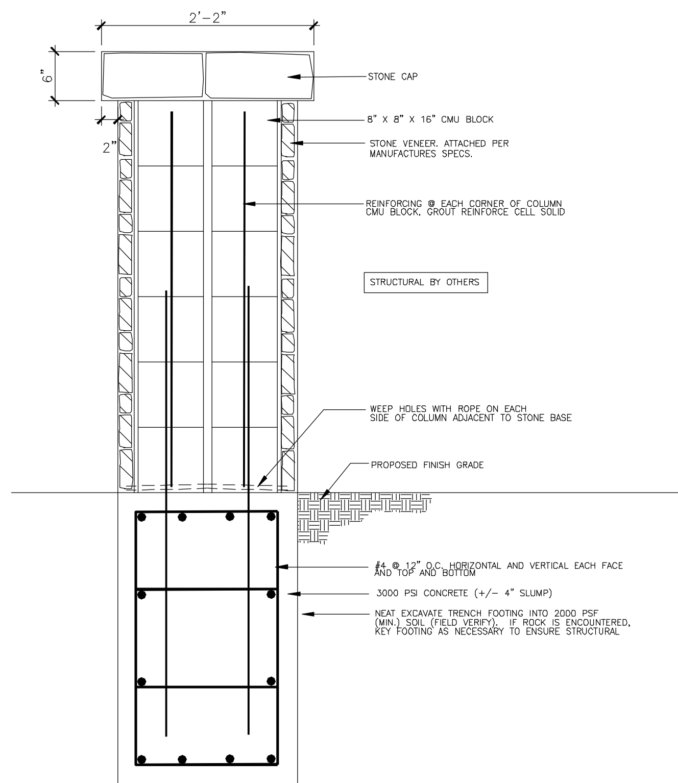
3 MONUMENT- SECTION B
