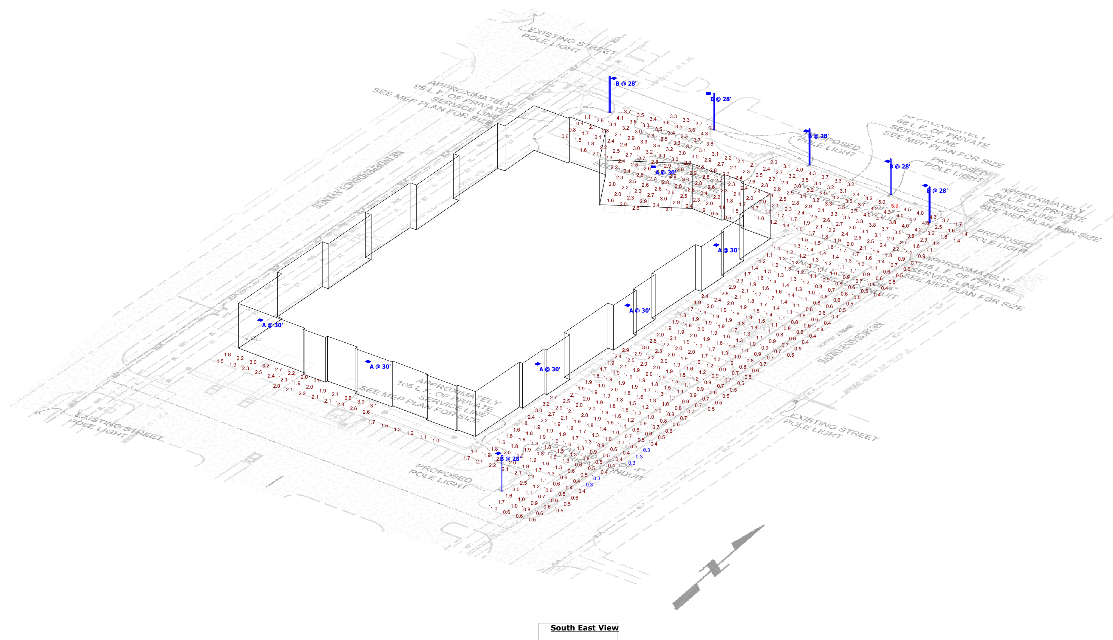
South East View
