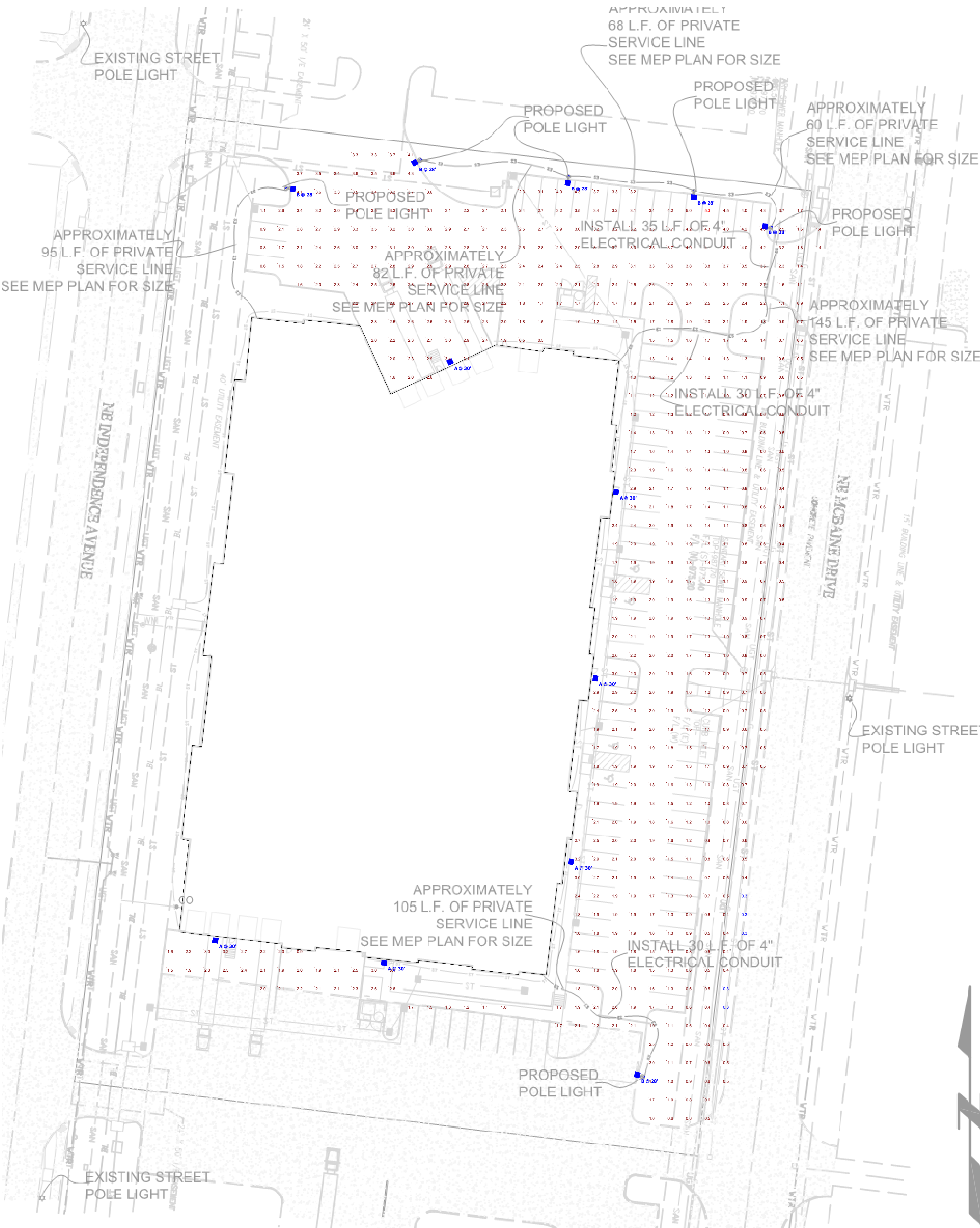
Plan View Scale: 1" = 25'
