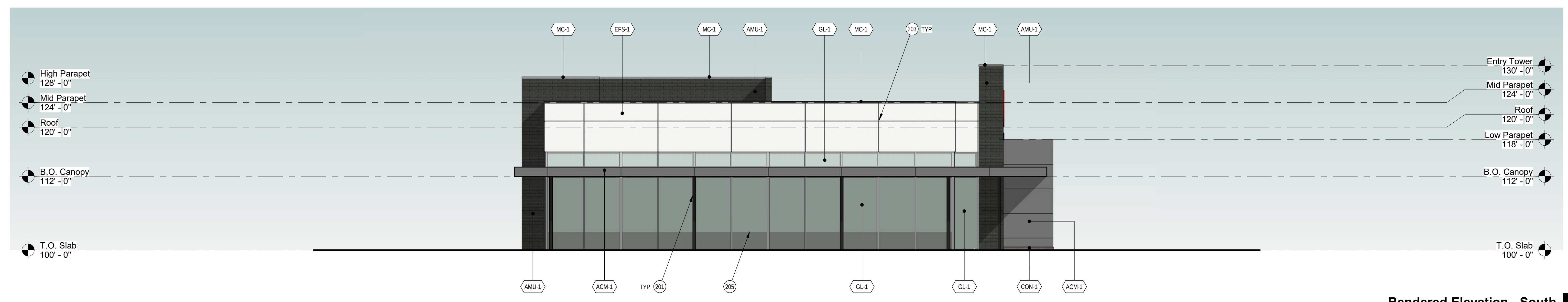
Rendered Elevation - South 1/8" = 1'-0" 2
