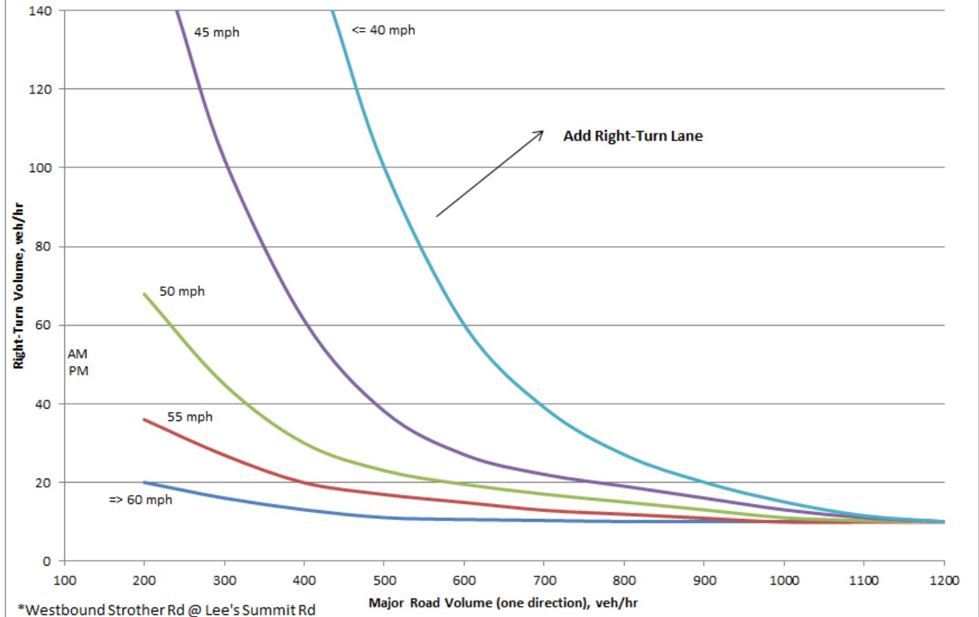
Right-Turn Guidelines for Two-Lane Roadways (Existing + Phase 1 Development)
