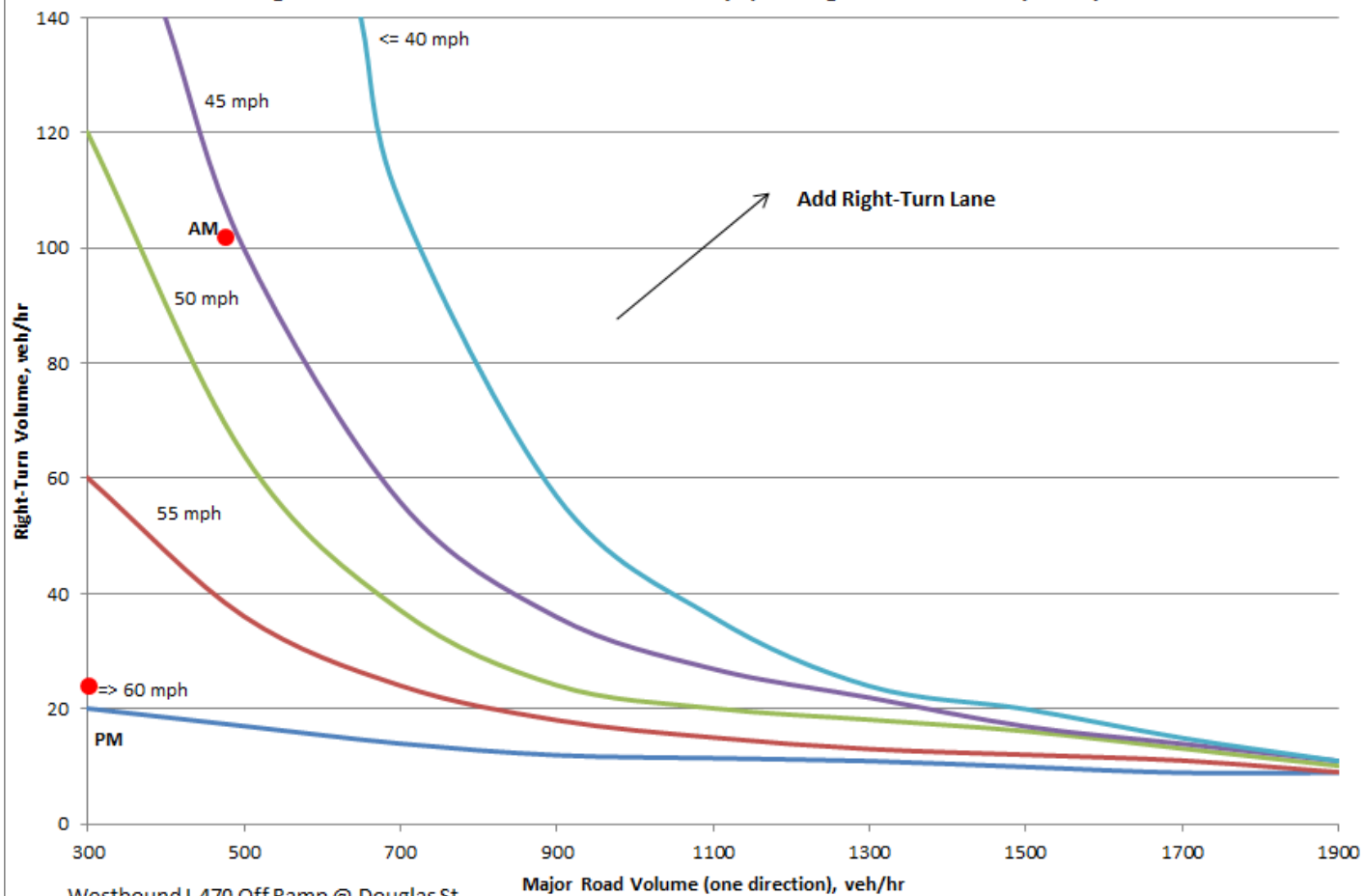
Right-Turn Guidelines for Four-Lane Roadways (Existing + Phase 1 Development)
