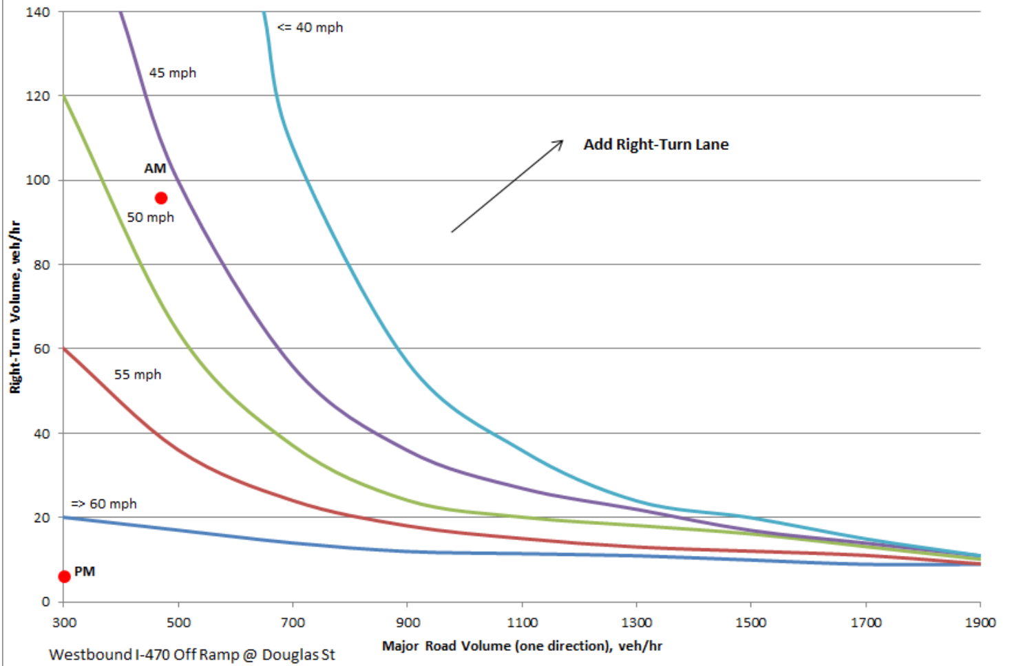
Right-Turn Guidelines for Four-Lane Roadways (Existing)
