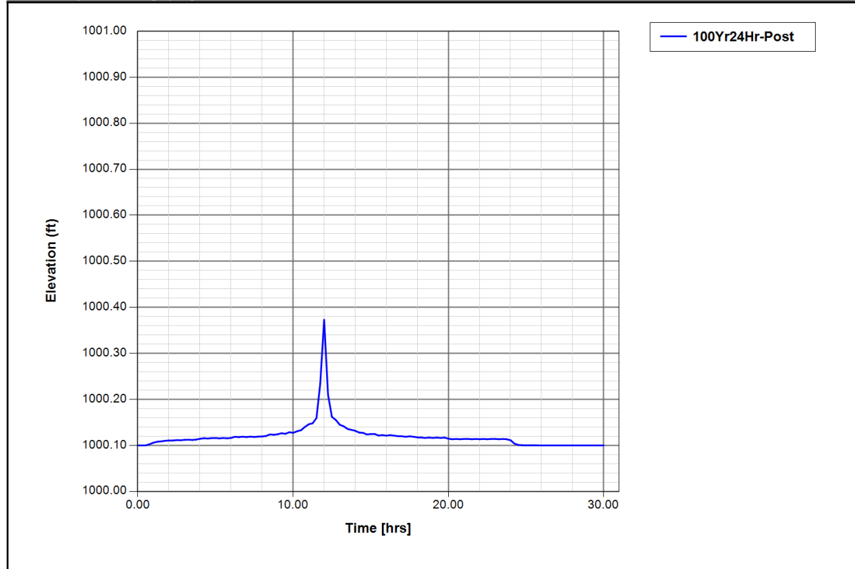
Node Stage: Pond A [Icpr3]
