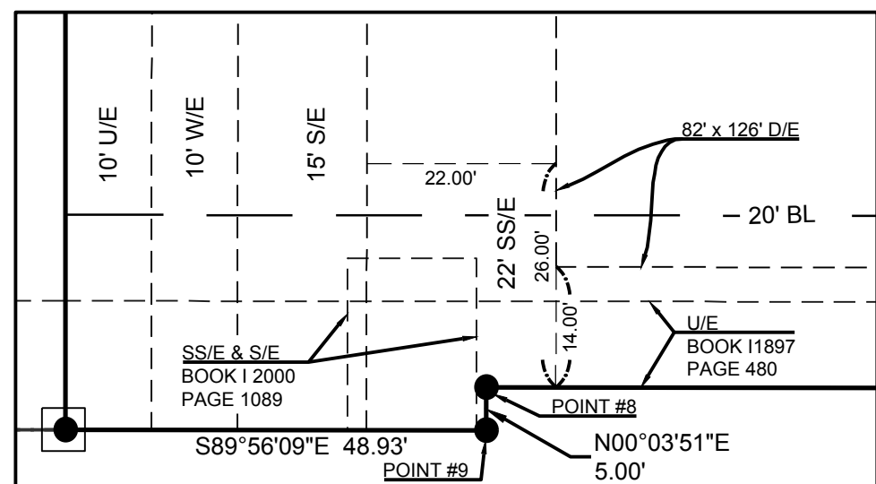
DETAILED AREA: SCALE: 1" = 20'
