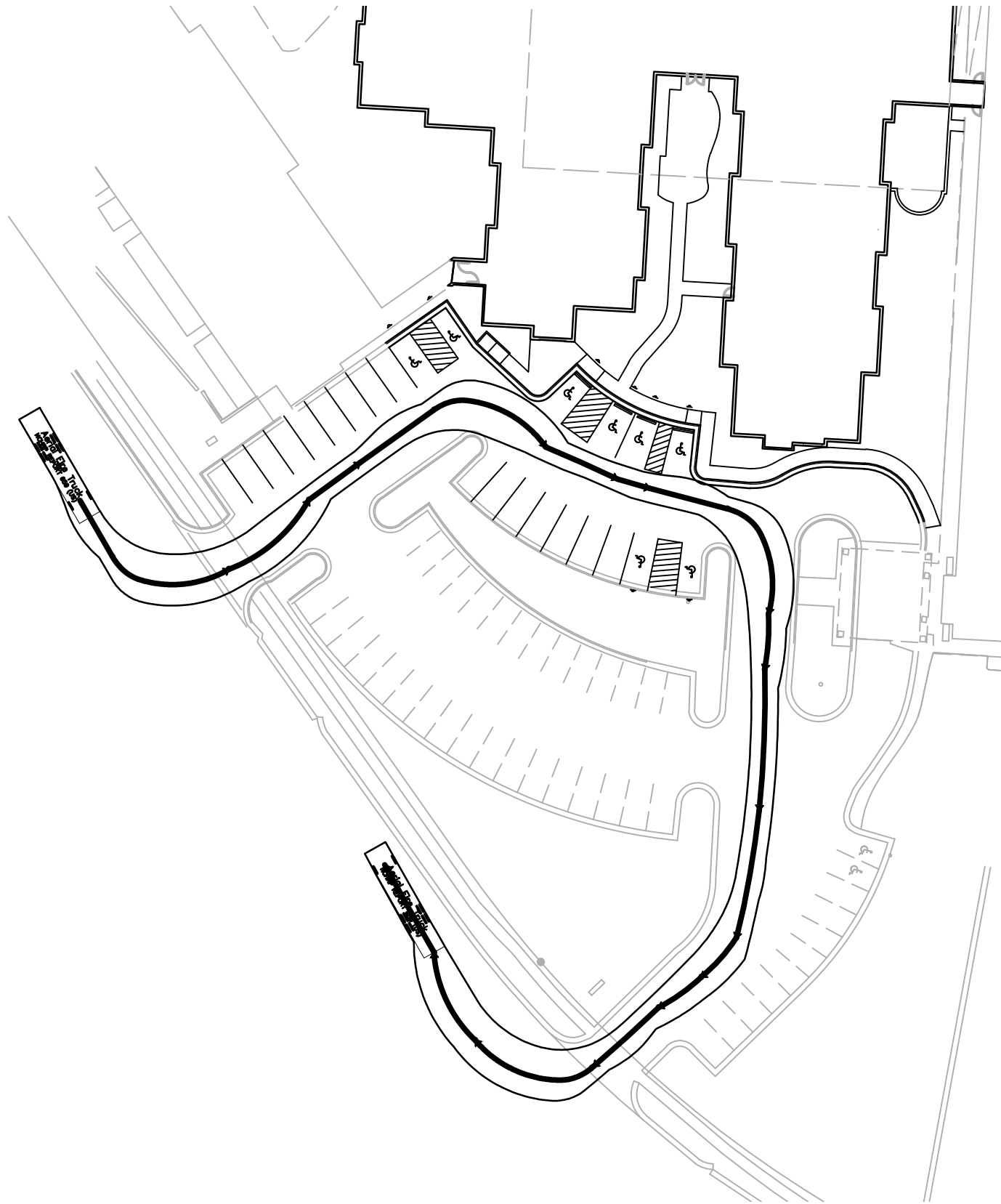
FIRE TRUCK TURNING EXHIBIT
