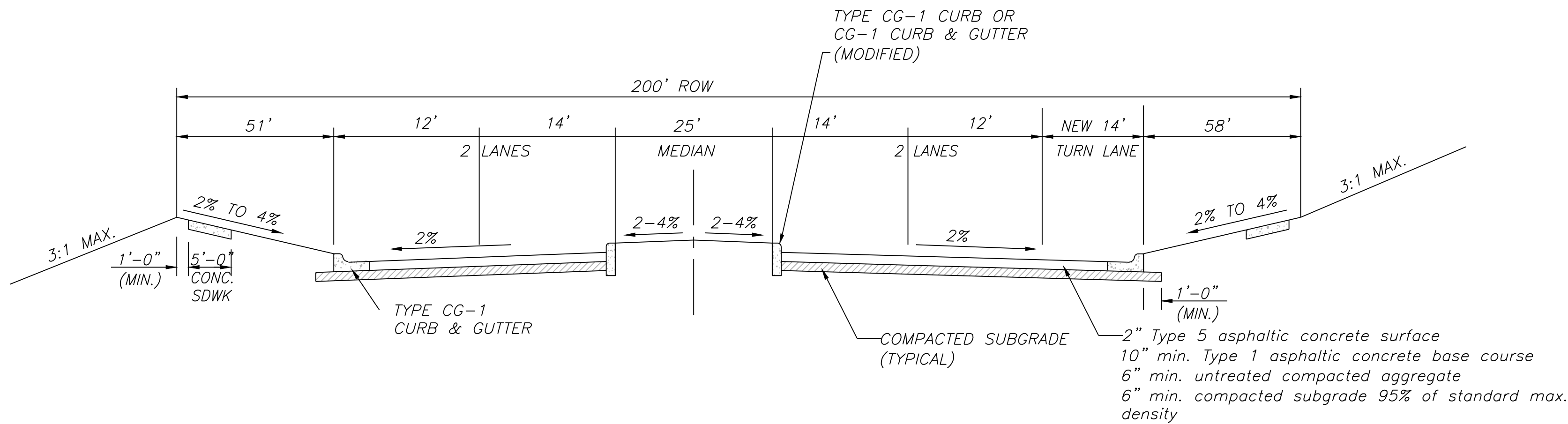
VIEW HIGH DRIVE TYPICAL SECTION (MAJOR ARTERIAL) N.T.S.
