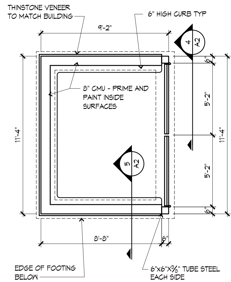
3 TRASH ENCLOSURE 1/4"=1'-0"
