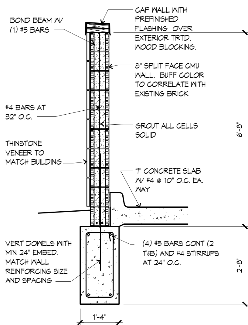
5 TRASH SECTION 1/2"=1'-0"
