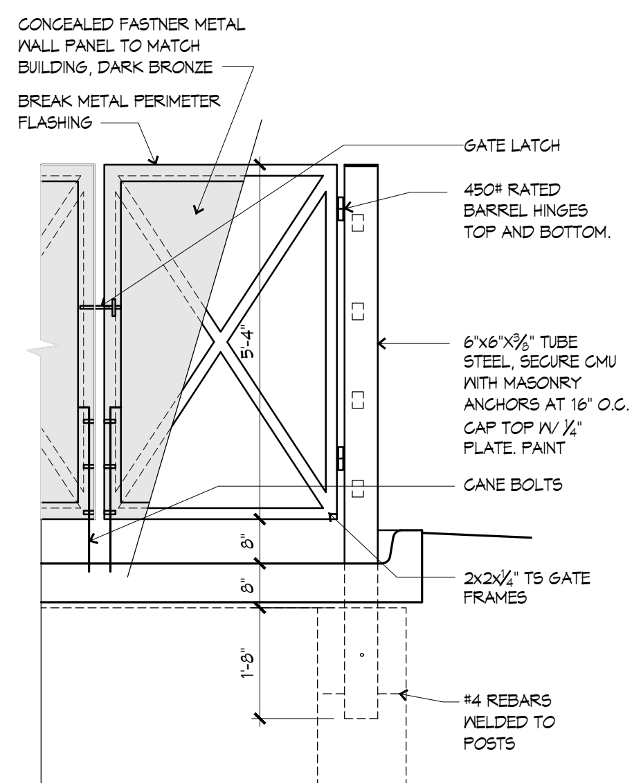
4 GATE ELEVATION 1/2"=1'-0"
