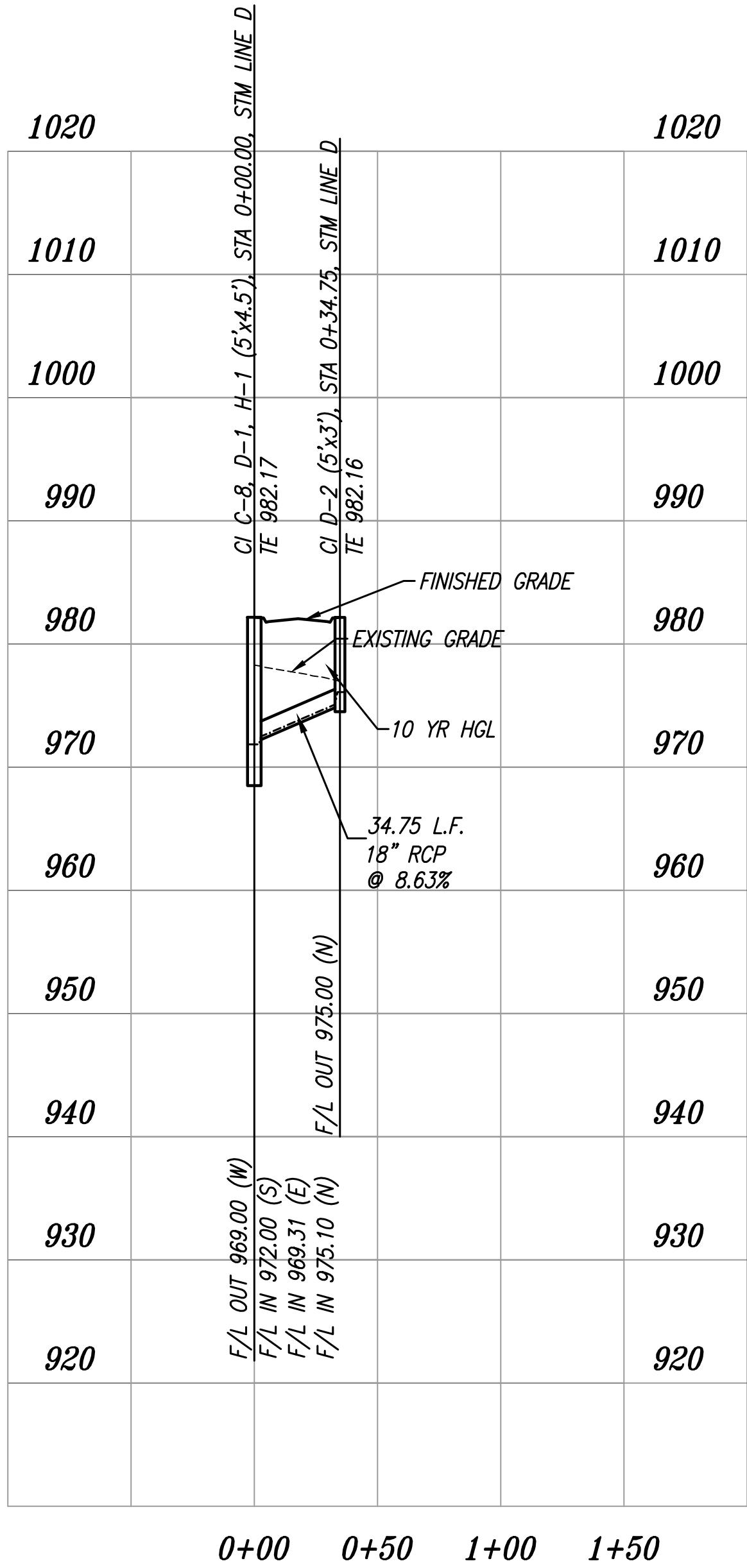
PROPOSED STORM LINE D
