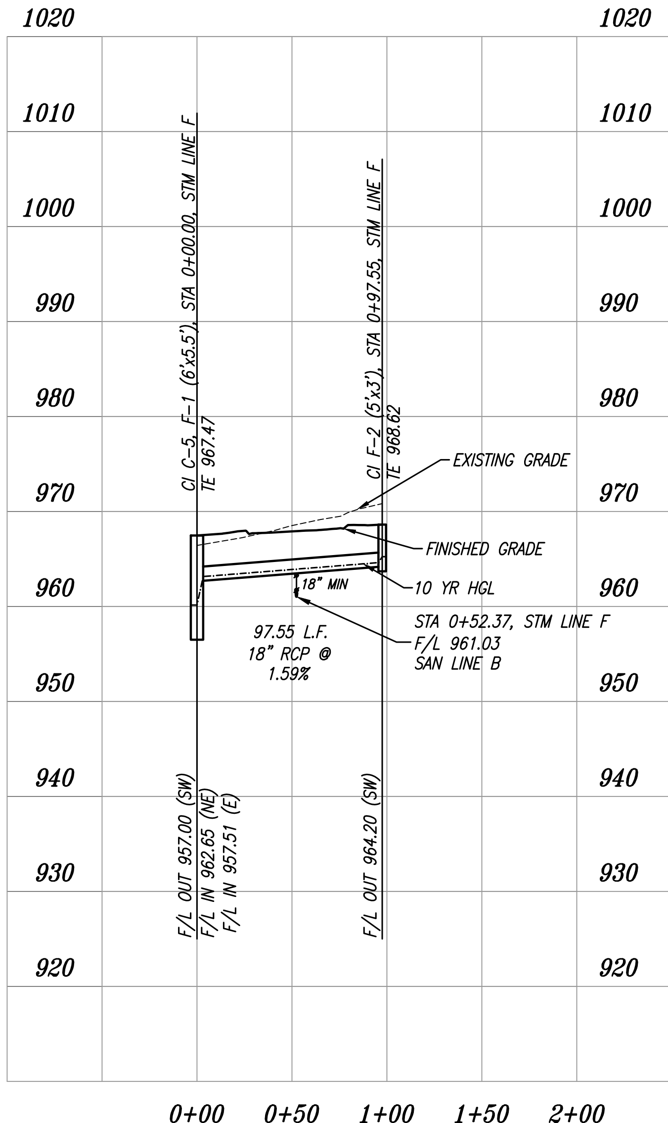
PROPOSED STORM LINE F
