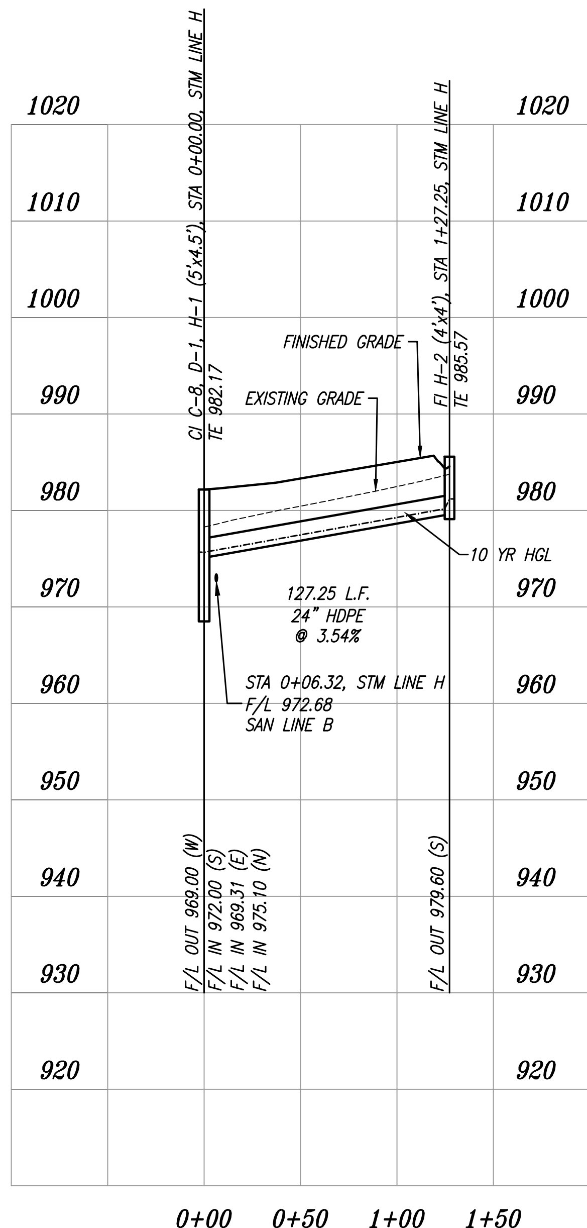
PROPOSED STORM LINE H
