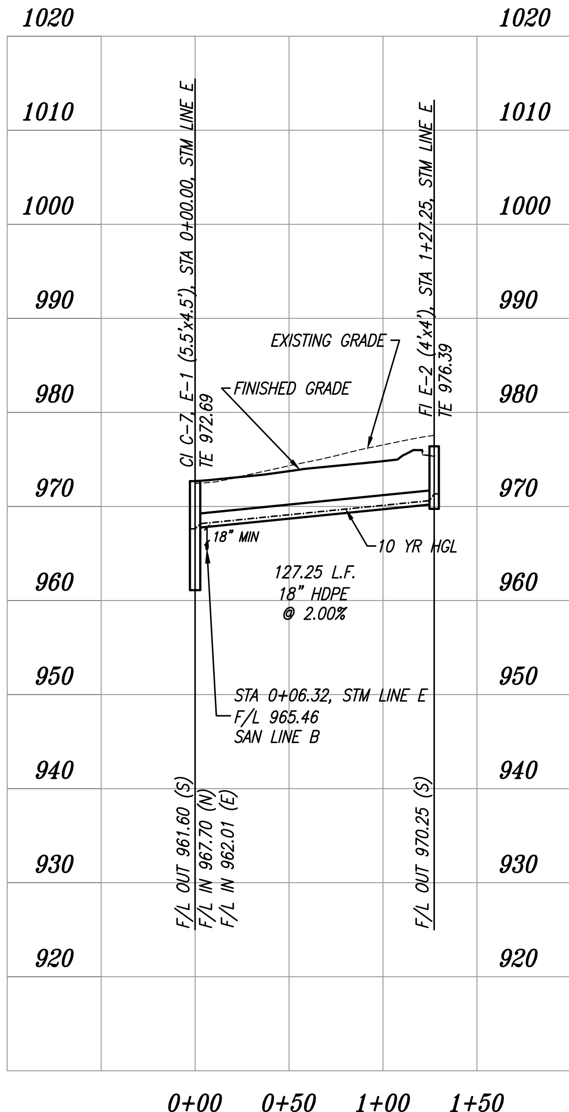
PROPOSED STORM LINE E
