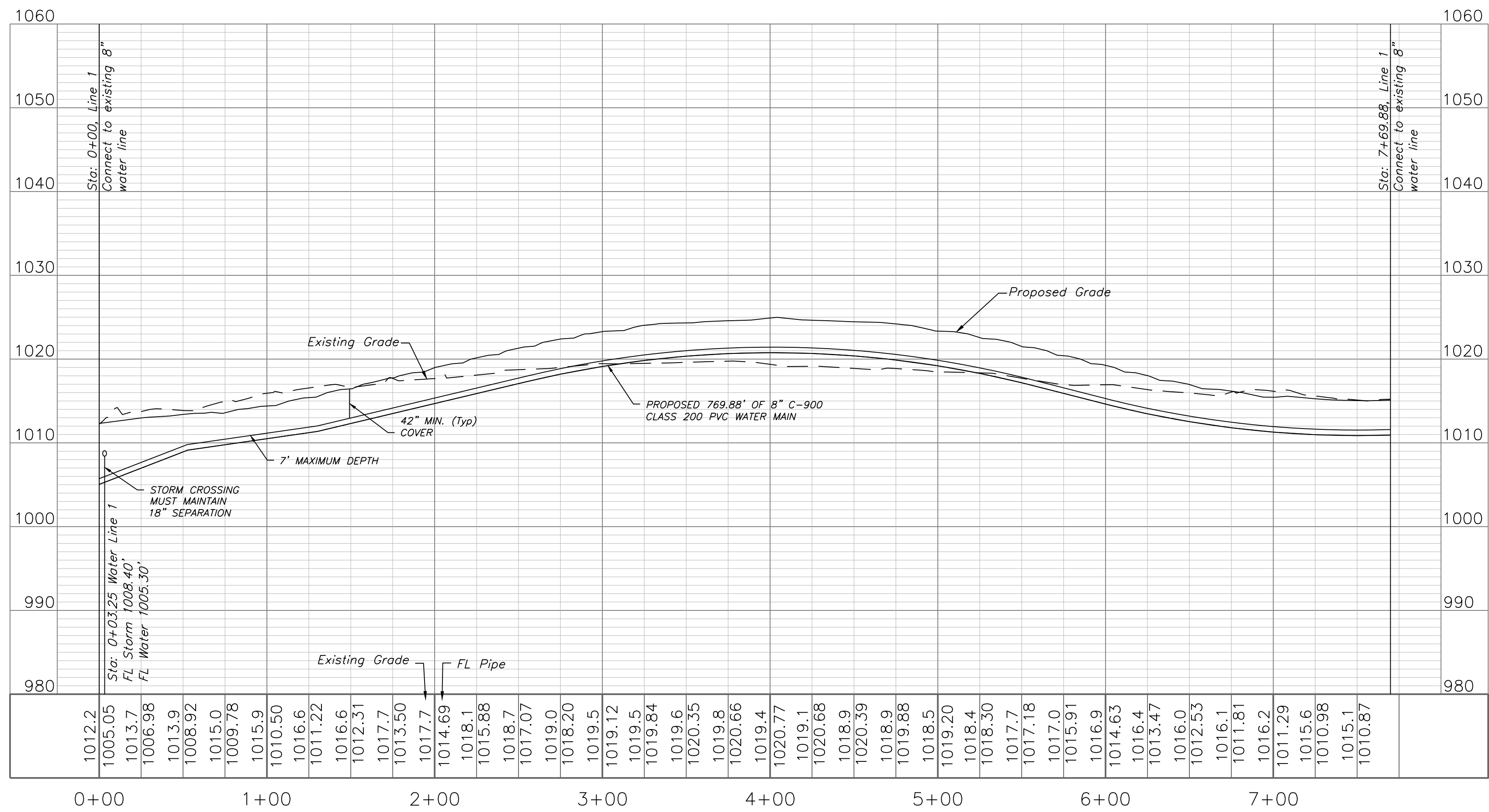
WATER LINE 1
